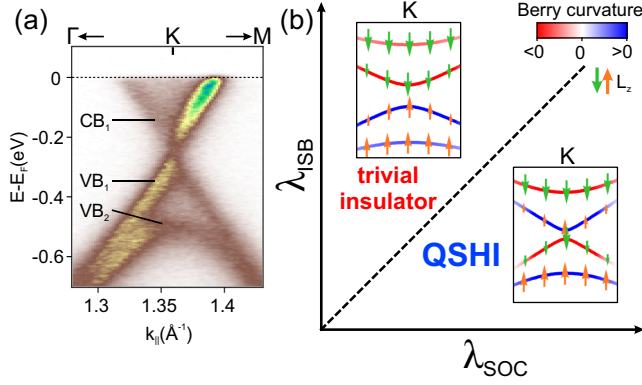
FIG. 1. (a) ARPES dispersion at the K point of n -doped indenene showing the two valence bands ( VB_1 , VB_2 ) as well as a partially occupied conduction band CB_1 ( h\nu = 21.2 eV 20 K). (b) Topological phase diagram of a p -electron system on the triangular lattice as a function of ISB ( \lambda_{\text{ISB}} ) and SOC strength ( \lambda_{\text{SOC}} ). The insets show the \langle L_z \rangle polarization (green and orange arrows) and the Berry curvature (red and blue curves) of the valence and conduction band states at K , calculated by DFT for the topologically trivial and nontrivial (QSHI) system. The topology of the system is reflected in both the OAM as well as the Berry curvature ordering sequence [19,21,22].
