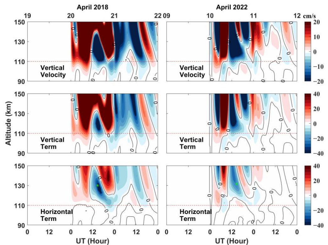
Figure 4. Storm-time differences ( r_{kp} - c_{kp} ) in vertical velocity, vertical term, and horizontal term at the location of ( 78.75^{\circ} S, 60^{\circ} E) in the altitude ranges of 90 km to 150 km in the two storms. The vertical velocity was the sum of the vertical term and horizontal term. The red dashed lines represent 110 km. The black lines represent the zero value. The green asterisks corresponded to the time and altitude of 14:20 UT and \sim 130 km, respectively.
