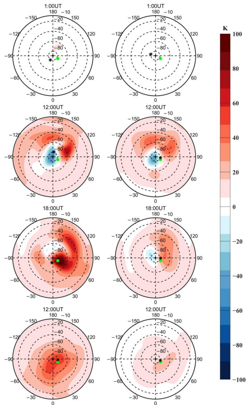
Figure 2. The first three rows correspond to the temperature difference ( rkp - ckp ) for TIMEGCM simulations at 01:00 UT (first row), 12:00 UT (second row), and 18:00 UT (third row) on the first day of the storm (20 April 2018 on the left column and 10 April 2022 on the right column) at 110 km in the southern hemisphere. The fourth row is the same as the first three rows but at 12:00 UT on the second day of the storm (21 April 2018 on the left column and 11 April 2022 on the right column). The black asterisks mark the locations of the satellite observation points at the corresponding time. The green dots mark the position of ( 78.75^\circ S, 60^\circ E), which is used for the subsequent thermodynamic diagnostic analysis.
