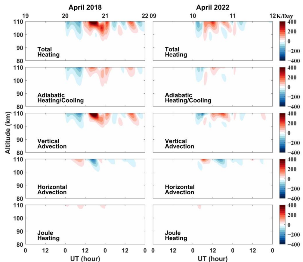
Figure 3. Storm-time differences (rkp-ckp) in total heating terms and major heating terms at the location of ( 78.75^\circ S, 60^\circ E) in the altitude ranges of 80 km to 110 km in the two storms: total heating, adiabatic heating/cooling, vertical heat advection, horizontal heat advection, and Joule heating.
