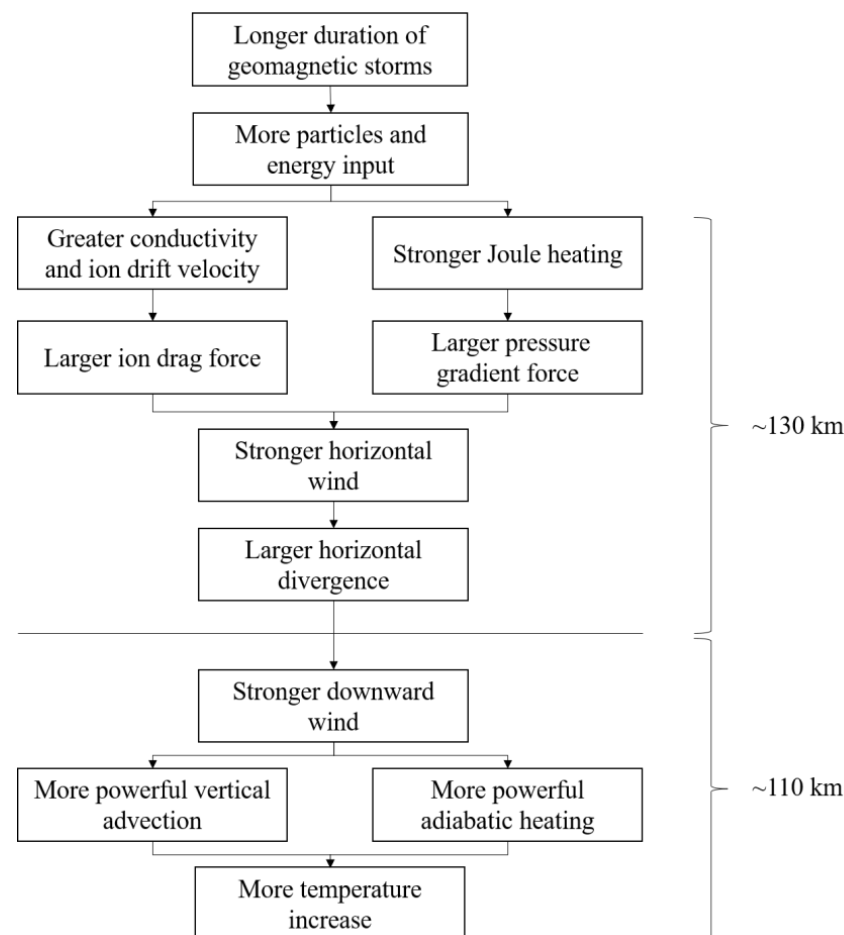
Figure 9. Schematic figure of the physical process of temperature increases due to geomagnetic storms with longer duration.
