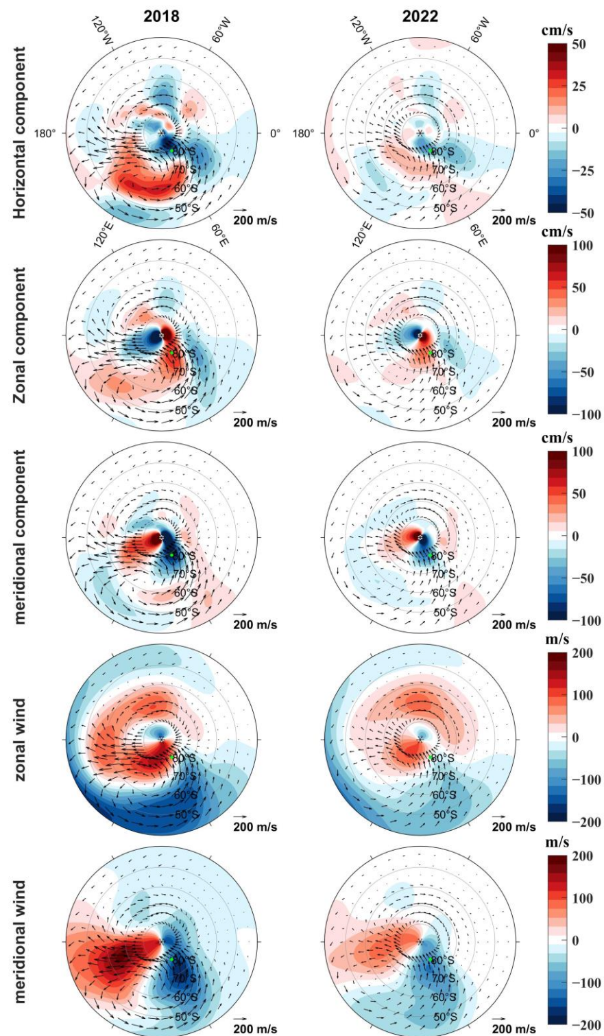
Figure 5. The left column corresponds to the 2018 storm event and the right column represents the 2022 storm event. The different rows show the effects of magnetic storms on the total horizontal divergence term (first row, same as the third row in Figure 4), the zonal component of the horizontal divergence term (second row), the meridional component of the horizontal divergence term (third row), the zonal wind (fourth row), and the meridional wind at 14:20 UT around 130 km. The green dot is located at (78.75° S, 60° E), which is the location where the kinetic diagnostic analysis is performed. The arrows show the magnitude and direction of the horizontal wind. The black asterisks mark the locations of the South Pole.
