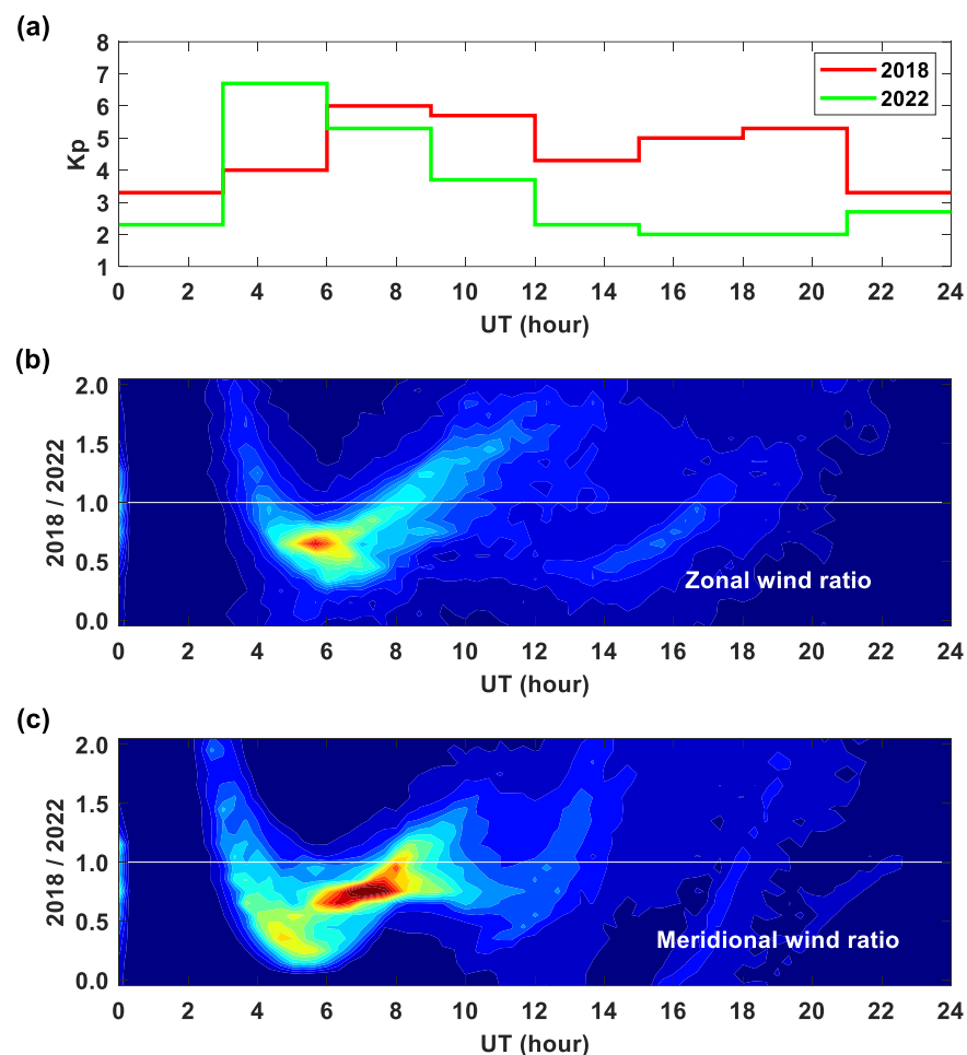
Figure 6. (a) The red line represents the Kp values on 20 April 2018 and the green line stands for the Kp values on 10 April 2022. (b) Each grid zonal wind velocity during the 2018 storm is divided by the 2022 zonal wind velocity on the same grid to obtain the ratio of the zonal wind speed for two events in each grid. Then, the number of grids are counted in each ratio and its proportion to the total number of grids is calculated. The figure shows the statistical distribution of zonal wind ratios (2018/2022) of grids from 50^\circ S to 90^\circ S in the two events over time, where >1 ( <1 ) represents a larger zonal wind velocity in the 2018 (2022) storm. (c) Same as (b), but corresponding to the meridional wind.
