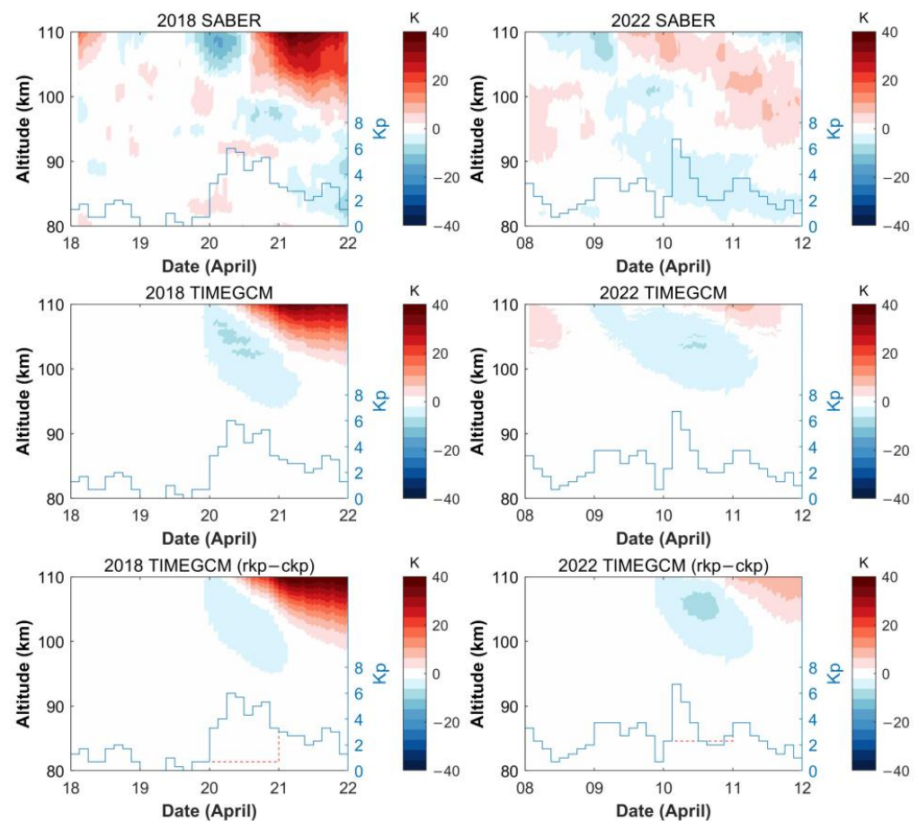
Figure 1. The difference between the zonal running SABER temperature (first row) during two geomagnetic storms in April 2018 (the left column) and April 2022 (the right column) and the average temperature of the two days before the storms (18–19 April 2018 and 8–9 April 2022, respectively) in the altitude ranges of 80–110 km from 77.5° S to 82.5° S. The second row is similar to the first row, but the data are simulated by TIMEGCM driven by real geomagnetic conditions (rkp). The third row shows the variations in temperature obtained by subtracting the simulation driven by constant geomagnetic conditions (ckp) from the simulation driven by real geomagnetic conditions (rkp). The blue lines are the real K_p values. The red lines are the quiet time K_p values as the driving condition of the ckp simulation. The two ckp are 1^+ for 20 April 2018, and 2^- for 10 April 2022, respectively. Then the constant K_p values are set the same as the real ones.
