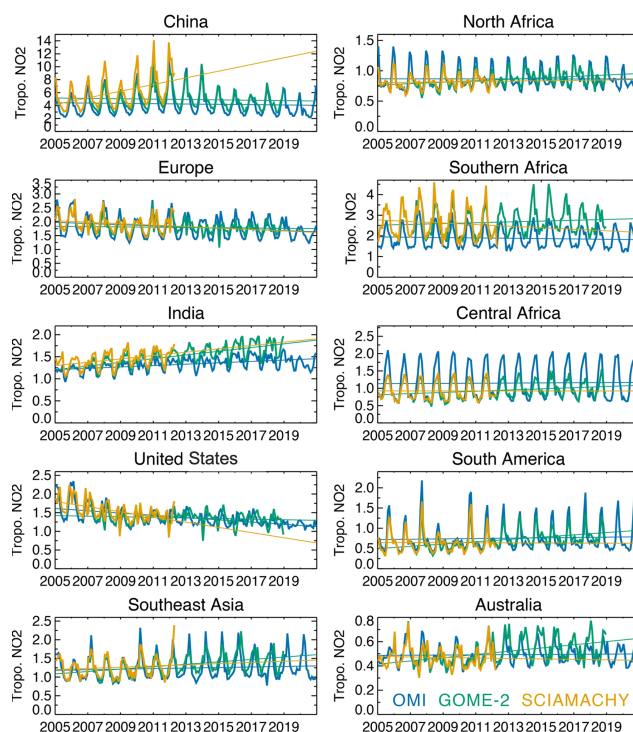
Figure 14. Time series of regional monthly mean tropospheric NO 2 columns (in 10^{15} \text{ molec. cm}^{-2} ) averaged over China (110–123° E, 30–40° N), Europe (10° W–30° E, 35–60° N), the US (70–125° W, 28–50° N), India (68–89° E, 8–33° N), South America (50–70° W, 20° S–Equator), northern Africa (20° W–40° E, Equator–20° N), central Africa (10–40° E, Equator–20° S), southern Africa (25–34° E, 22–31° S), southeastern Asia (96–105° E, 10–20° N), and Australia (113–155° E, 11–44° S) obtained from OMI (black), GOME-2 (blue), and SCIAMACHY (red).
