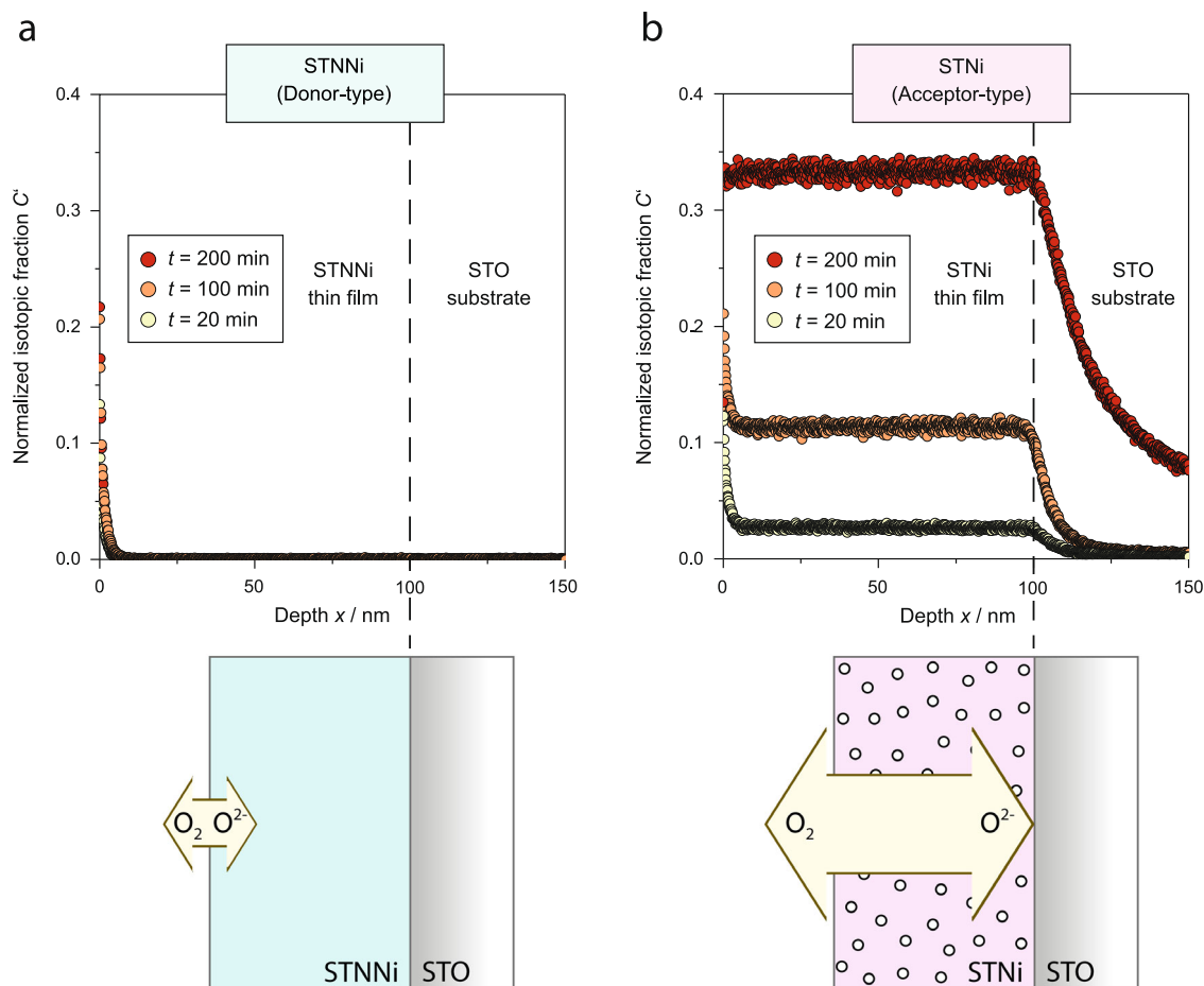
Fig. 1 | Oxygen tracer exchange studies. a ^{18}O profiles determined by SIMS analysis for STNNi (donor-type) and b STNi (acceptor-type) after joint equilibration in ^{18}O_2 gas and subsequent exchange in ^{18}O_2 gas for different annealing times of t = 20 min, t = 100 min, and t = 200 min at T = 400^\circ C and p(O_2) = 200 mbar. The tracer fraction C^*(x, t) incorporated into the thin film samples during oxygen exchange is plotted versus the sputter depth, respectively. A schematic illustration
