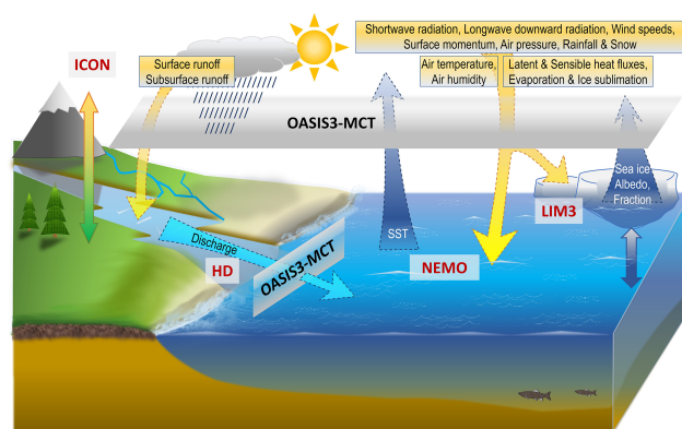
Figure 1. Model components of GCOAST-AHOI and variables exchanged via the OASIS3-MCT coupler. Two solid arrows display the communication between the atmosphere and land (yellow-green arrow) and between the ocean and sea ice (grey-blue arrow), which is done via subroutines inside ICON-CLM and NEMO, respectively. Dotted arrows show the transfer between components via the OASIS interface. Yellow arrows present atmospheric transfer to ocean sea ice and river runoff. The cyan arrow shows the discharge from the river to the ocean. Blue arrows demonstrate the transfer of sea surface temperature (SST) from the ocean as well as the sea ice albedo and sea ice fraction to the atmosphere.
