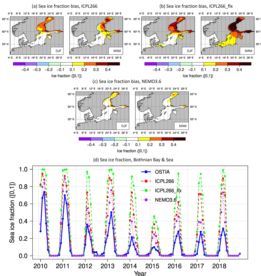
Figure 11. Sea ice fraction bias of (a) ICPL266, (b) ICPL266_fix, and (c) NEMO3.6 compared to the OSTIA data in winter (DJF) and spring (MAM) averaged over the period 2010–2018. (d) Monthly mean of the sea ice fraction averaged over the Bothnian Bay and Bothnian Sea (red box in Fig. 11a) for OSTIA, ICPL266, ICPL266_fix, and NEMO3.6 during 2010–2018.
