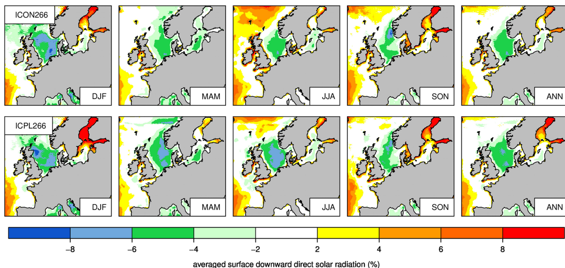
Figure 7. Seasonal (DJF, MAM, JJA, SON) and ANN means of the shortwave downward radiation bias (%) of ICON266 (top) and ICPL266 (bottom) compared to the ERA5 data for the period 2010–2018 over the GCOAST domain.
