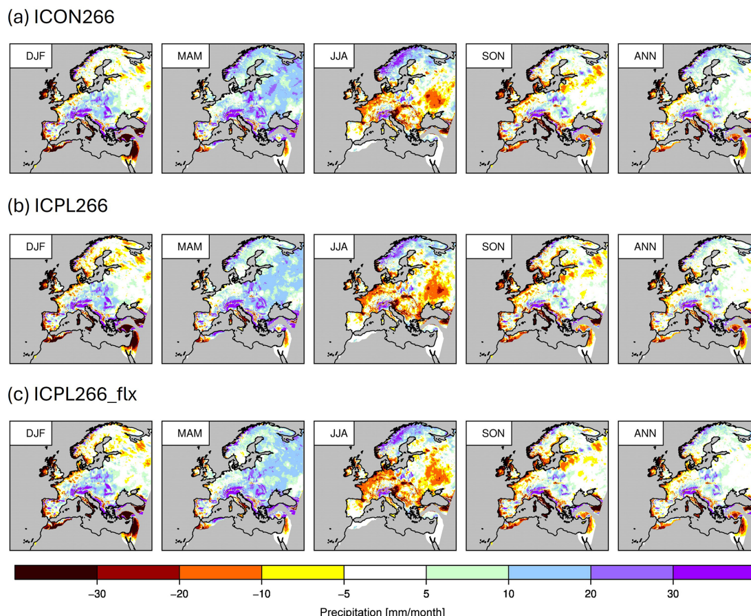
Figure 9. Seasonal (DJF, MAM, JJA, SON) and ANN differences of precipitation (millimetres per month) for (a) ICON266, (b) ICPL266, and (c) ICPL266_flx compared to the E-OBS data for the period 2010–2018.
