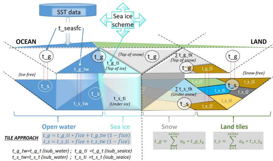
Figure 3. Surface temperature exchange between the atmosphere and ocean or land in ICON and GCOAST-AHOI.
