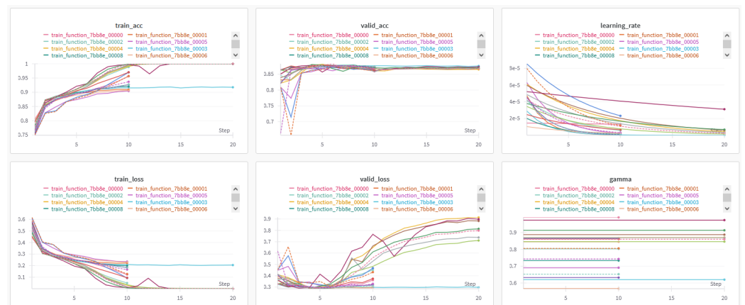
ASHA - Scheduler
