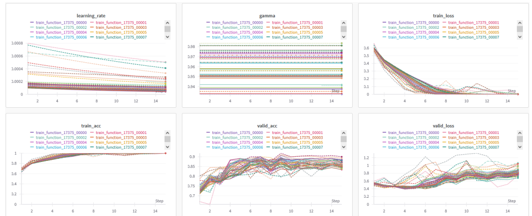
FIFO - Scheduler
