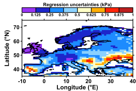
Figure 5. Regression uncertainties for each grid cell. Uncertainties are calculated as the time-averaged 10 %–90 % range of individual reconstructions from each grid point (for the longest period with reconstruction skills, see Fig. 4).
