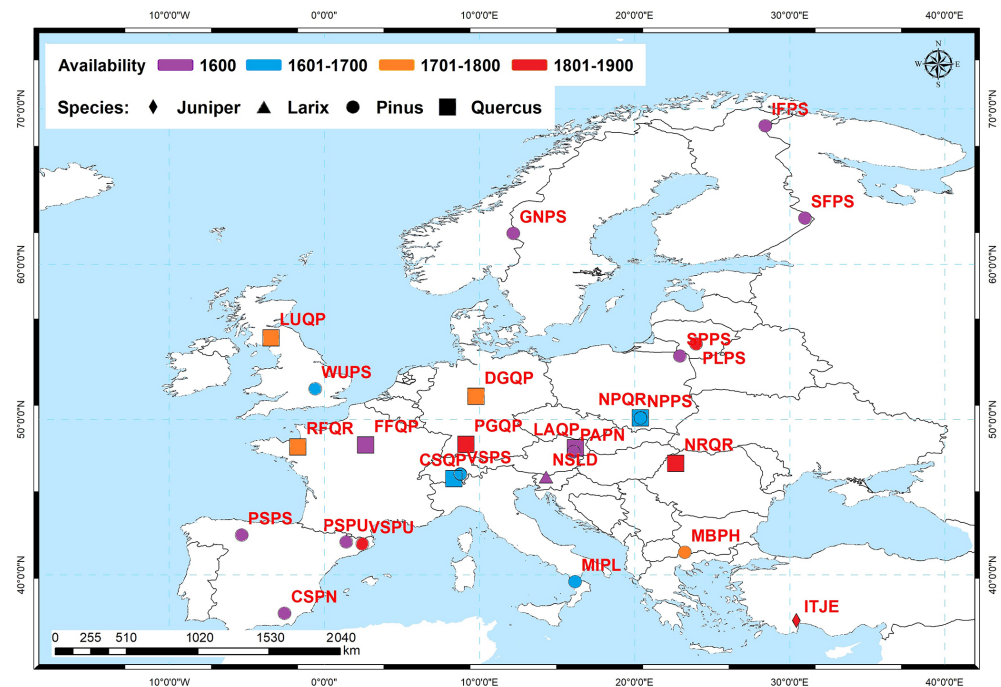
Figure 1. The site distribution of the \delta^{18}\text{O} network composed of 21 ISONET and 5 additional datasets (see Table 1). Colors indicate the past temporal availability of each tree ring dataset: starts in 1600 or earlier (purple), starts between 1601 and 1700 (blue), starts between 1701 and 1800 (orange), and starts between 1801 and 1900 (red). Symbols indicate tree species used for each record: Juniper (diamond), Larix (triangle), Pinus (circle), and Quercus (square).
