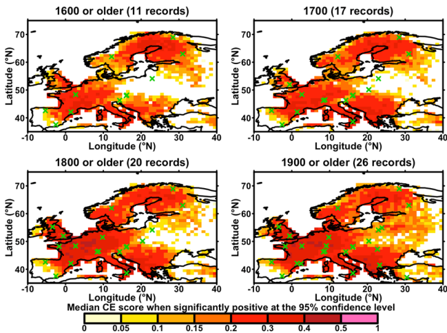
Figure 4. The median Nash–Sutcliffe S_{\{CE\}} for four different time slices. The colored areas show the regions where the model setup has a suitable quality, which was tested with a one-sided Student's t test for the average of 30 S_{\{CE\}} scores obtained for testing samples ( p < 0.05 , Sect. 2.5). For the sake of graphical representation, for each time slice plotted here, the median S_{\{CE\}} scores were averaged over the corresponding nested time frames. Locations of available records for each time slice are given by green crosses (see Table 1).
