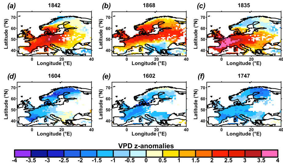
Figure 10. Spatial pattern of VPD anomalies for selected years. Values of each grid cell are VPD z anomalies (standardized and centered) with respect to the whole period of study (1600–1994). The chosen years were selected as they are the three with the highest VPD z anomalies (a–c, a is the highest) and the three with lowest VPD z anomalies (d–f, d is the lowest) for preindustrial data (1600–1899). Time series only include years where S_{\{CE\}} scores are significantly positive at the 95 % confidence level (see Fig. 4).
