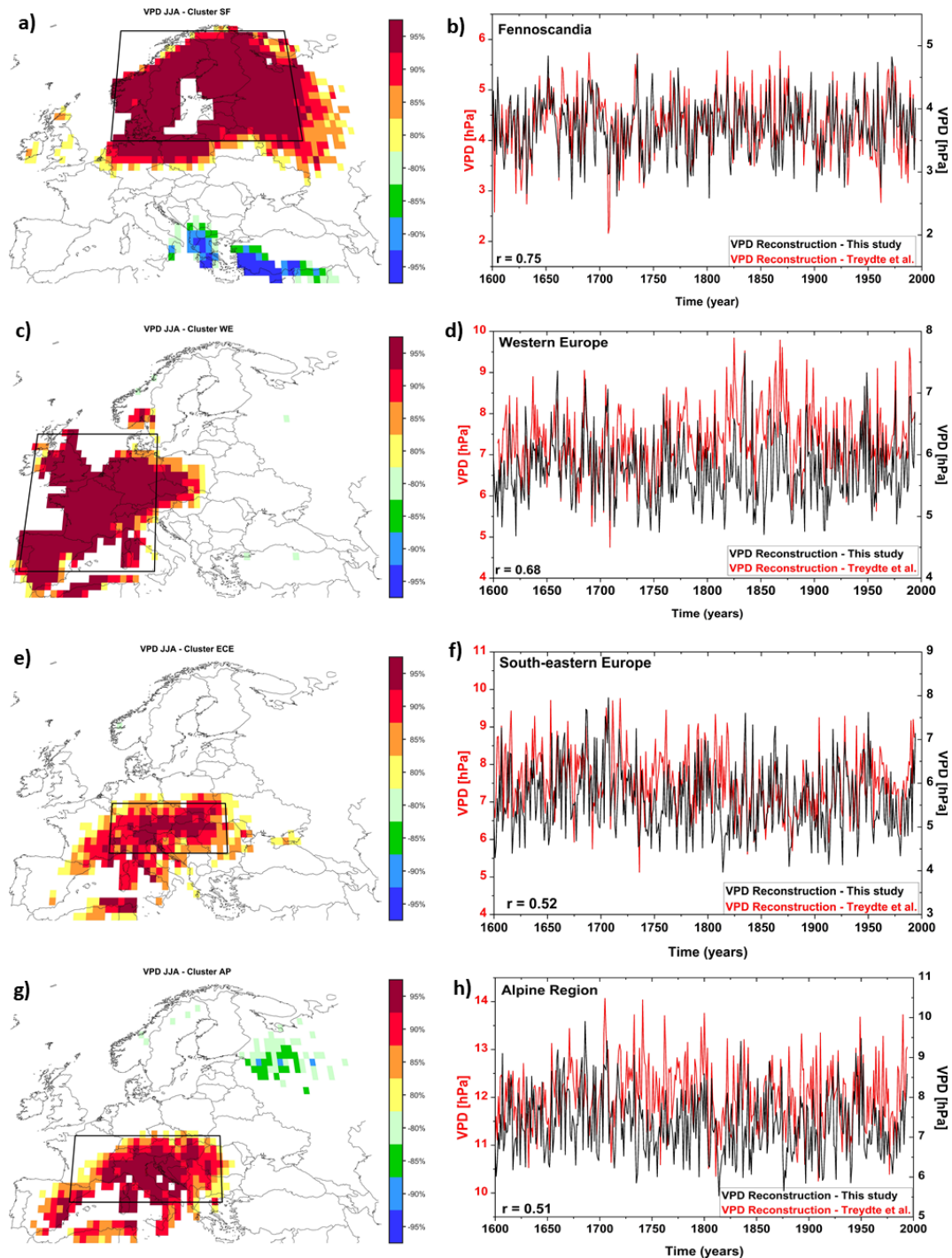
Figure 8. (a) Stability maps between the gridded VPD reconstruction from this study and the reconstructed time series of VPD over southern Fennoscandia (Treydte et al., 2023). (b) The temporal evolution of the VPD time series averaged over the black box in (a) and the VPD time series over southern Fennoscandia (Treydte et al., 2023). Panel (c) is the same as (a) but for western Europe, panel (d) is the same as (b) but for western Europe, panel (e) is the same as (a) but for southeastern Europe, panel (f) is the same as (b) but for western southeastern Europe, panel (g) is the same as (a) but for the Alpine region, and panel (h) is the same as (b) but for the Alpine region. In (a), (c), (e), and (g) the regions where the correlation is stable, positive, and significant for at least 80 % of the 31-year moving window correlations are shaded with dark red (95 %), red (90 %), orange (85 %), and yellow (80 %). The corresponding regions where the correlation is stable but negative are shaded with dark blue (95 %), blue (90 %), green (85 %), and light green (80 %).
