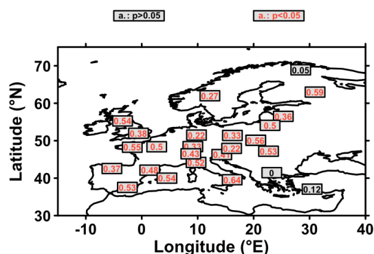
Figure 3. Correlation of the \delta^{18}\text{O} time series with local summer VPD for the period 1900 to 1994. For each tree ring dataset, the correlation is computed with the time series from the closest grid point. The significance of correlations is calculated using a Student's t test for correlation with corrected degrees of freedom from time series as in McCarthy et al. (2015) and Michel et al. (2020). Significant correlations at the 95 % confidence level are highlighted in red ( p < 0.05 ).
