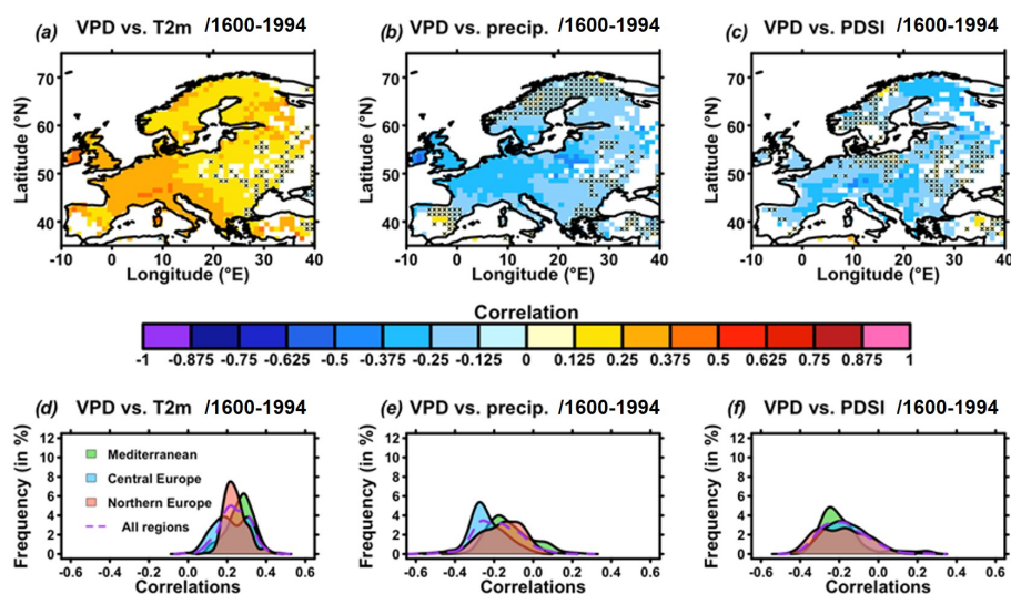
Figure 7. Comparison with former climate field reconstructions. (a–c) Correlations between the VPD reconstruction from this study and other climate reconstructions: (a) temperature at 2 m (T2m) (Luterbacher et al., 2004), (b) precipitation (precip) (Pauling et al., 2006), and (c) Palmer Drought Severity Index (PDSI) (Cook et al., 2015) for the period 1600–1994. Black crosses indicate no significance at the 95 % confidence level. (d–f) Distribution of correlations from (a–c) for the same three variables, respectively, for the three regions investigated, i.e., Mediterranean (green), central Europe (blue), northern Europe (red), and all regions (purple dashed line), following IPCC AR6 (Iturbide et al., 2020; Fig. 5).
