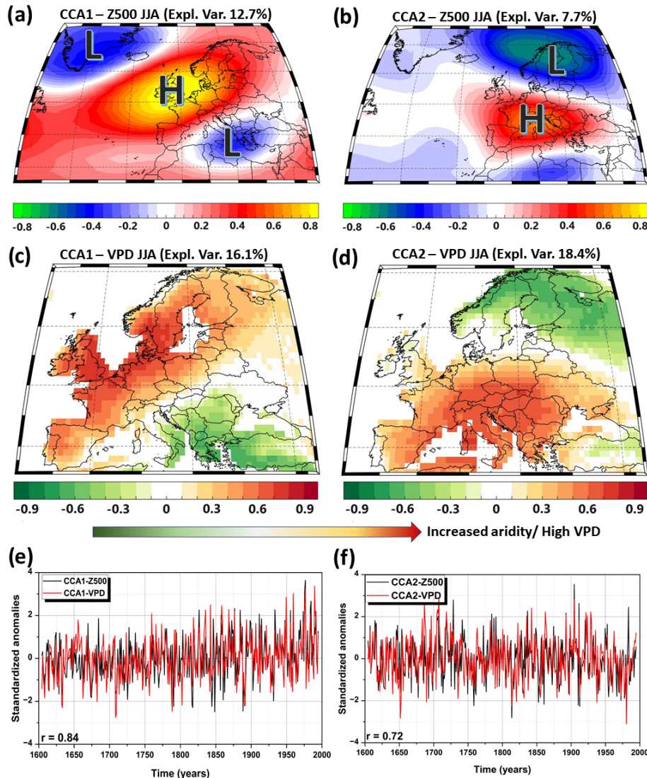
Figure 9. The first coupled mode of variability (CCA1 – left column) and second coupled mode of variability (CCA2 – right column) between summer Z_{500} (a, b) and summer VPD (c, d). (e) The standardized amplitudes corresponding to CCA1 Z_{500} (black line) and CCA1 VPD (red line). (f) The standardized amplitudes corresponding to CCA2 Z_{500} (black line) and CCA2 VPD (red line).
