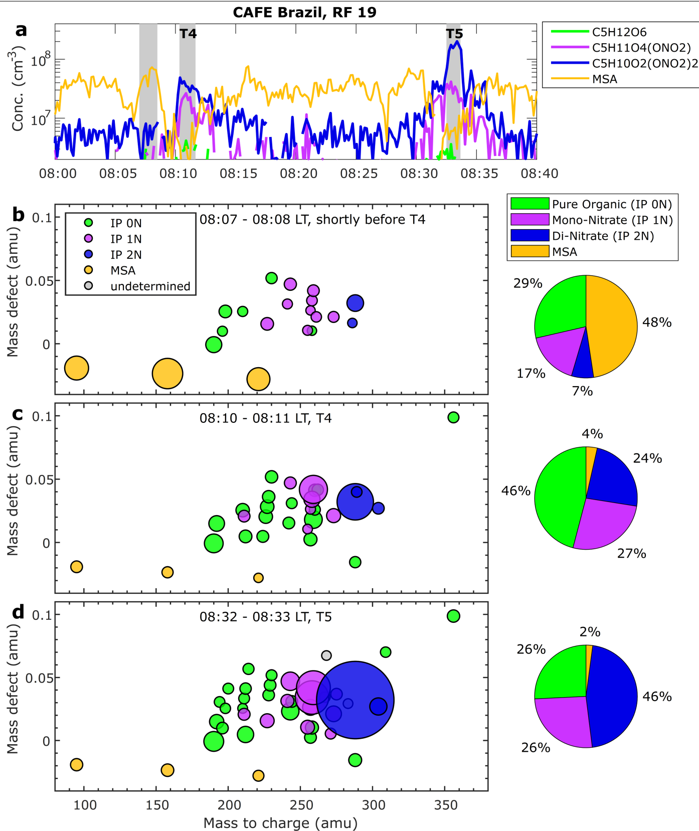
Extended Data Fig. 5 | Time series and mass-defect plots for CI-API-TOF data before and during NPF events of RF 19. a , Time series of the most prominent mononitrates and dinitrates C 5 H 11 O 4 (ONO 2 ) and C 5 H 10 O 2 (ONO 2 ) 2 , representative IP ON compound C 5 H 12 O 6 and MSA. b , Signals strongly shift between an air parcel that is not influenced by the fresh convection (which
