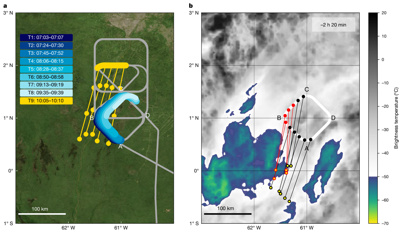
Fig. 2 | Flight path and air-mass back trajectories. a , Flight path for RF19 (grey). The diamond-shaped pattern ABCD was flown repeatedly and the NPF air mass was encountered several times (thick-coloured sections T4–T9) also before the NPF event started (T1–T3). Coloured sections T1–T8 are each slightly shifted to the right to prevent overlap. Thin yellow lines with 1-h markers indicate 3 h of back trajectories from the NPF period T9 used to calculate and identify periods T1–T8. b , Back trajectories from the locations of the aircraft between 08:05 and 08:15 local time (black and red markers) to 140 min before (yellow-centred markers) and infrared satellite image (GOES-16, band 13:
