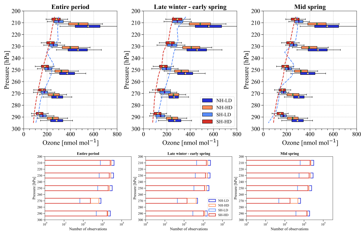
Figure C1: Ozone box plot (nmol mol -1 ) and associated observation numbers by pressure bins obtained from CAMS reanalysis (45°-60°S and 90°-40° W). The plots include ozone data with RH lower than 20%. The vertical red and blue dashed lines are the ozone medians in the SH obtained from ozonesondes (high depletion years) and SouthTRAC measurements (low depletion years), respectively. In the upper panel, the left, middle and right plots show the entire period, late winter-early spring and mid-spring, respectively, for the northern and southern hemispheres and high-depleted and low-depleted years. Box plots indicate the median, the 25th and 75th percentiles. The whiskers extend to the 5th and 95th percentiles. In the lower panels, the X-axis shows the observation numbers. The rest of the plot information is the same as described in the upper panel.
