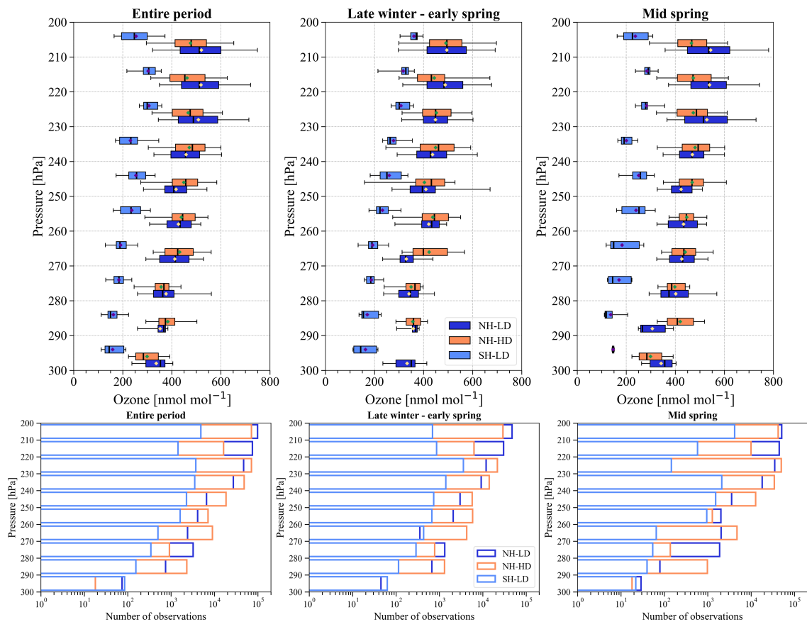
Figure B1: Ozone box plot ( \text{nmol mol}^{-1} ) and associated observation numbers by pressure bins. The plots include ozone data with CO lower than 50 \text{ nmol mol}^{-1} . In the upper panel, the left, middle and right plots show the entire period, late winter-early spring and mid-spring for the northern and southern hemispheres and high-depleted and low-depleted years. Box plots indicate the median, the 25th and 75th percentiles. The whiskers extend to the 5th and 95th percentiles. In the lower panels, the X-axis shows the observation numbers. The rest of the plot information is the same as described in the upper panel.
