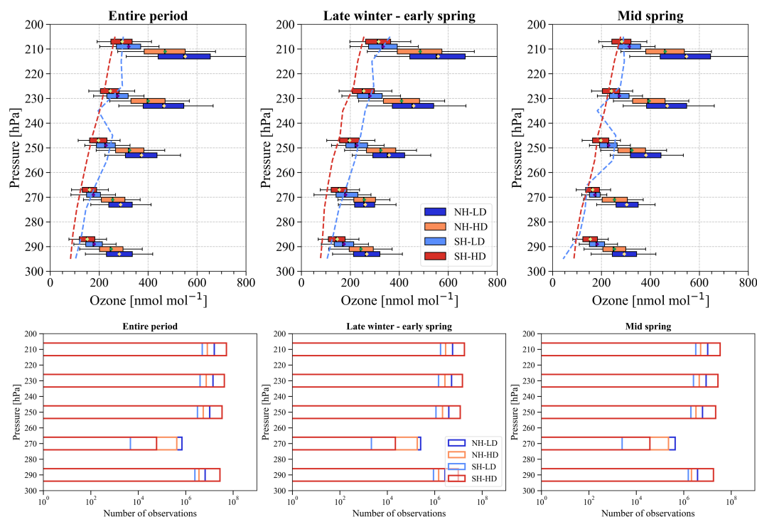
Figure 5: Ozone box plot ( \text{nmol mol}^{-1} ) and associated observation numbers by pressure bins obtained from CAMS reanalysis. The plots include ozone data with RH lower than 20%. The vertical red and blue dashed lines are the ozone medians in the SH obtained from ozonesondes (high depletion years) and SouthTRAC measurements (low depletion years), respectively. In the upper panel, the left, middle and right plots show the entire period, late winter-early spring and mid-spring, respectively, for the northern and southern hemispheres and high-depleted and low-depleted years. Box plots indicate the median, the 25th and 75th percentiles. The whiskers extend to the 5th and 95th percentiles. In the lower panels, the X-axis shows the observation numbers. The rest of the plot information is the same as described in the upper panel.
