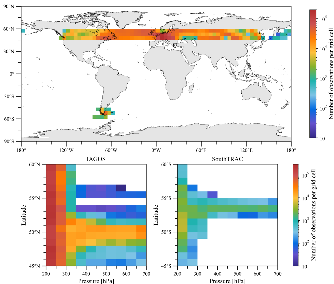
Figure 1: Routes position frequency obtained from aircraft GPSs. All panels show only SouthTRAC and IAGOS data within the same latitudinal band 45°-60° in the SH and NH. The upper panel shows the number of GPS observations by grid cell (5° x 5°) between 700 and 200 hPa. The lower panels show the number of GPS observations in every grid cell (1° x 50 hPa) between 700 and 200 hPa for IAGOS (left) and SouthTRAC (right).
