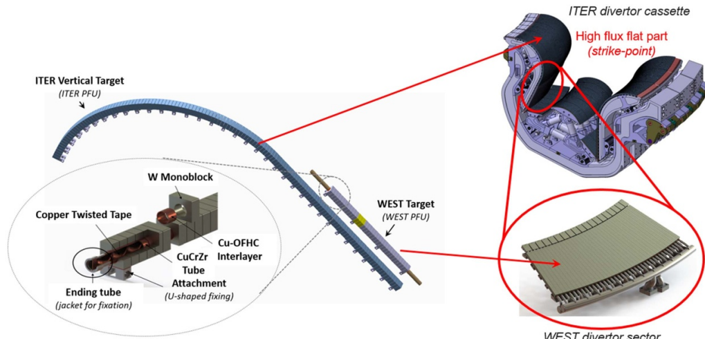
Figure 2. Comparison of an ITER divertor cassette and the WEST lower divertor. WEST uses the same mono-block technology, the same geometrical shape of the mono-blocks (toroidal bevel) and the same thermohydraulic conditions as ITER. Reprinted from [2], Copyright (2023), with permission from Elsevier.
