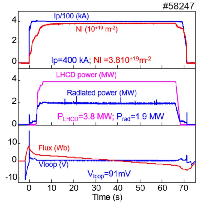
Figure 17. Plasma scenario used for the high fluence campaign at the end of the C7 experimental campaign.
