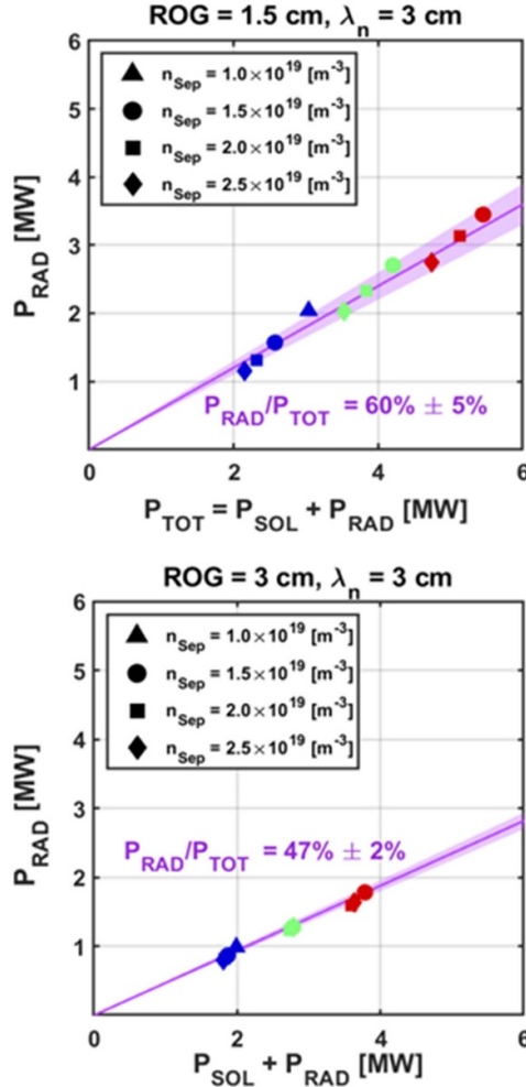
Figure 8. 3D transport simulations with SOLEDGE-ERO2.0 [16, 17] for two different radial outer gaps (ROG) between the RF antennas and the separatrix. Reproduced with permission from [17]. 29th IAEA Fusion Energy Conference (FEC 2023), Oct 2023, Londres, United Kingdom. (cea-04566270).
