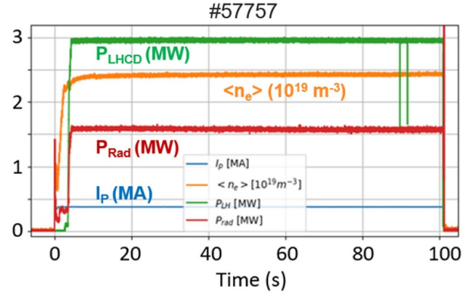
Figure 4. Example of 100 s long discharge in WEST phase 2.
