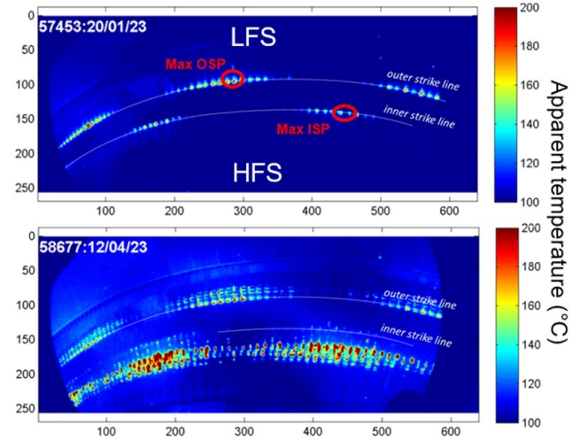
Figure 21. IR images of the ITER-grade divertor (top view, standard IR camera) in apparent temperature (assuming \varepsilon = 1 ) during the high fluence campaign, at the beginning (top) and end (bottom) of the campaign. The divertor heat load pattern is modulated toroidally by the magnetic field ripple (see [9] for more details).
