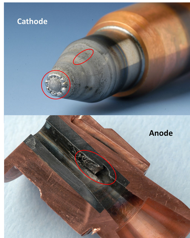
Fig. 1 Worn cathode (top) and anode (bottom, cross-section) of a single-cathode/anode conventional F4 plasma torch
