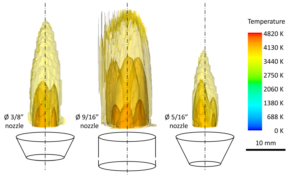
Fig. 8 Tomographic 3D reconstruction temperature distribution in the plasma jet of an Axial III TM plasma torch when using three different nozzle diameters (3 x 230 A, 112 slpm N 2 , 38 slpm H 2 , nozzle Ø 3/8"); reproduced and rearranged from (Ref 20), licensed acc. to the terms of the Creative Commons Attribution 4.0 International License ( https://creativecommons.org/licenses/by-nc/4.0/ )
