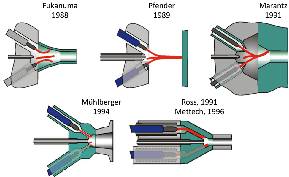
Fig. 7 Examples of multiple-arc plasma generators; reproduced from (Ref 3), licensed acc. to the terms of the Creative Commons Attribution Non-Commercial License CC BY-NC 3.0 ( https://creativecommons.org/licenses/by-nc/3.0/ )
