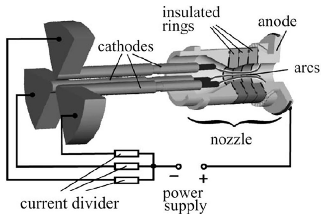
Fig. 10 Design of the Triplex I gun with three cathodes and one anode, left schematic reproduced from (Ref 3), licensed acc. to the terms of the Creative Commons Attribution Non-Commercial License CC BY-NC 3.0 ( https://creativecommons.org/licenses/by-nc/3.0/ )
