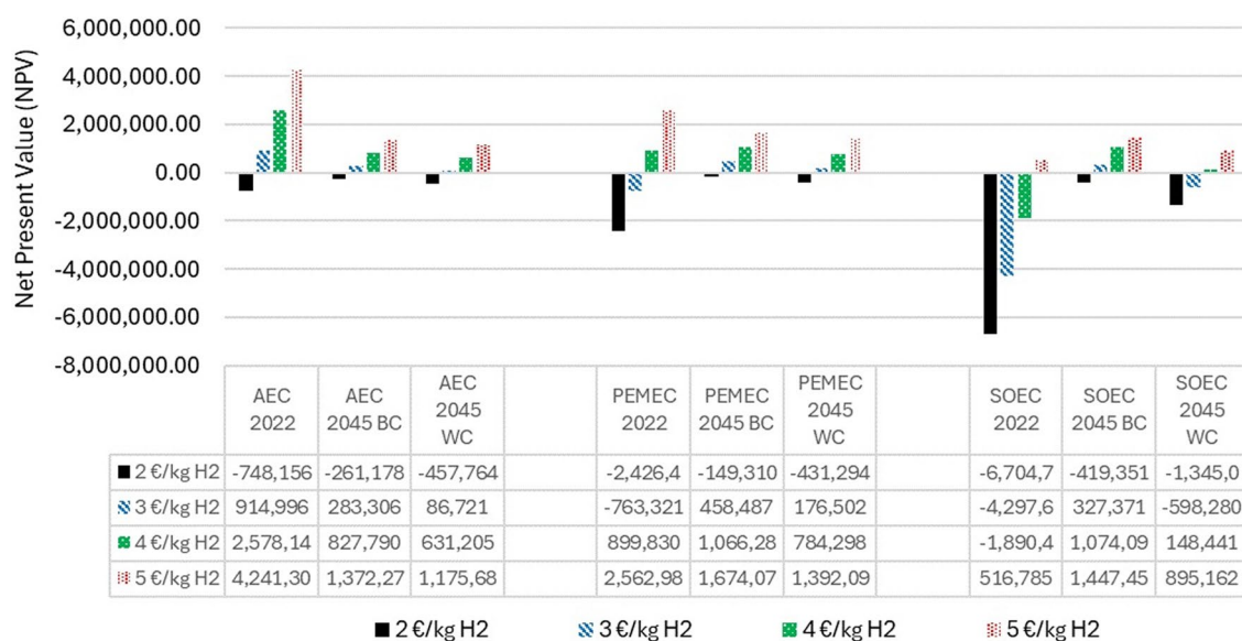
Fig. 11 NPV results of AEC, PEMEC, and SOEC for the years 2022 and 2045
