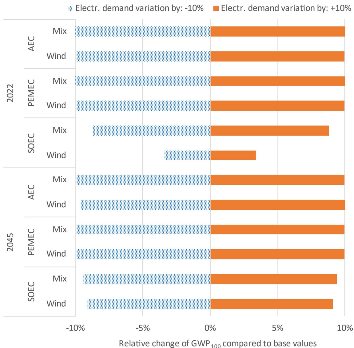
Fig. 13 Effects of electricity demand variations of \pm 10\% on the GWP_{100} results for three electrolysis technologies
