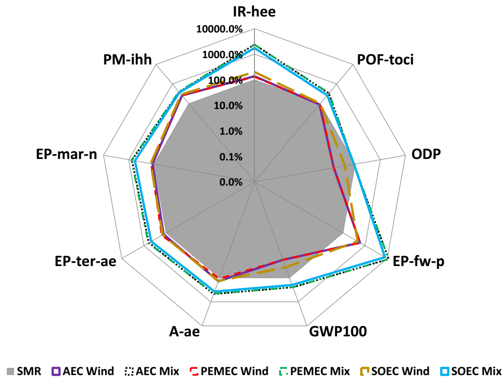
Fig. 8 Comparison of AEC, PEMEC, and SOEC with SMR for the year 2022 using several environmental indicators
