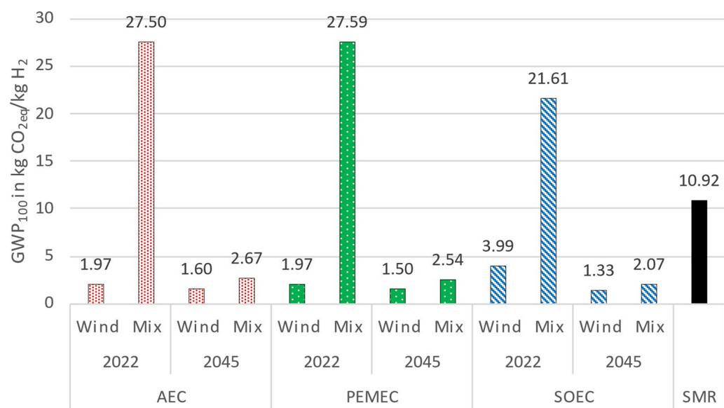
Fig. 5 GWP 100 results for power supply variants (Wind, electricity mix (Mix)) of hydrogen production by AEC, PEMEC, and SOEC compared to SMR
