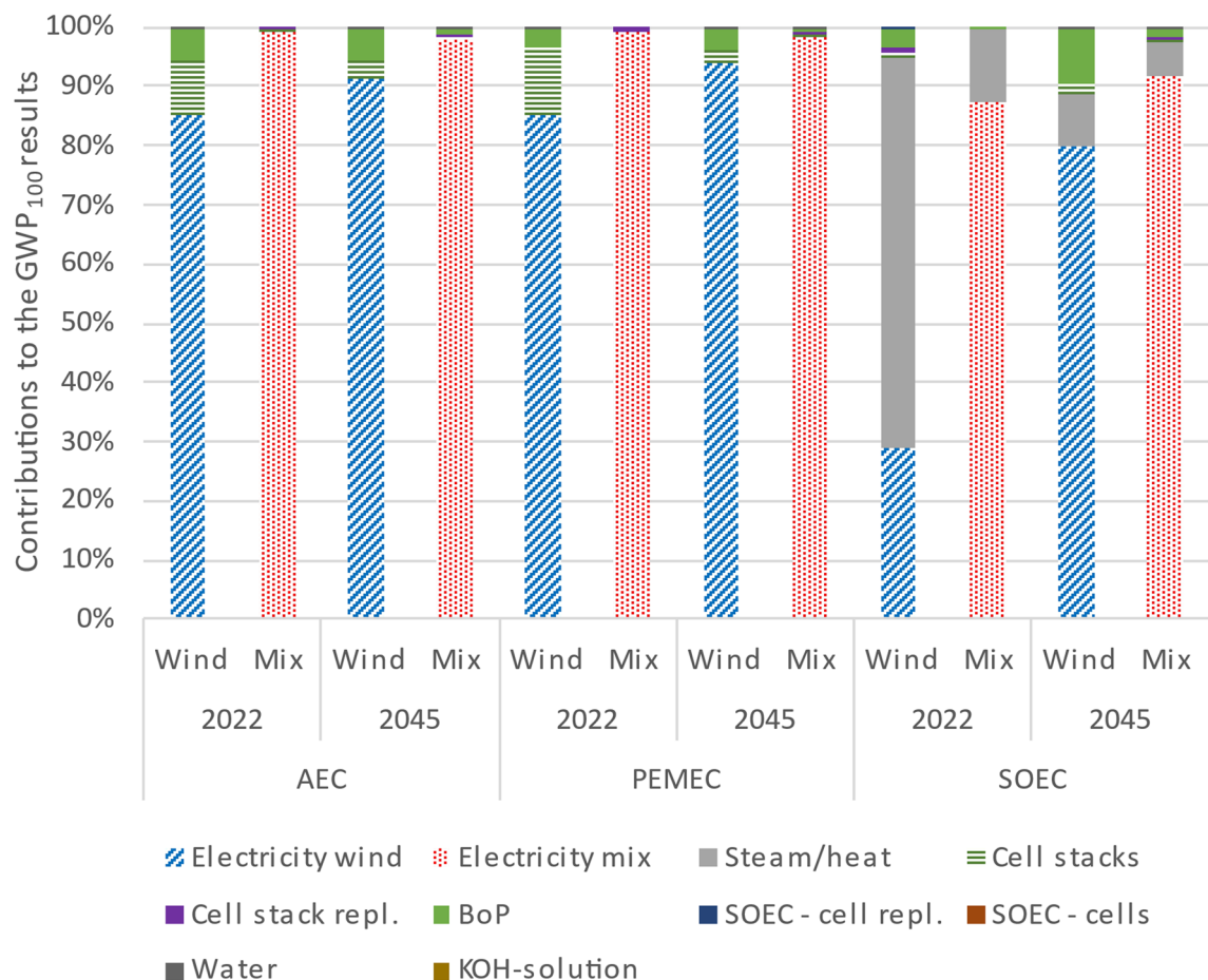
Fig. 6 Contribution analysis for AEC, PEMEC, and SOEC for the indicator GWP 100
