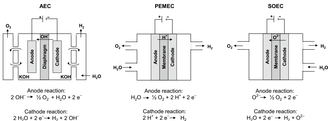
Fig. 1 AEC, PEMEC, and SOEC: schematic illustration of cell concepts and reactions; based on Steinmüller et al. and Liu et al. [3, 19]
