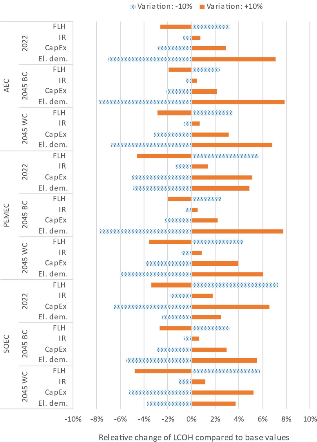
Fig. 14 Effects of parameter variations (FLH, IR, CapEx, El. dem.) of ± 10% for three electrolysis technologies on the LCOH results for three electrolysis technologies—including prospective best cases (BC) and worst cases (WC)
