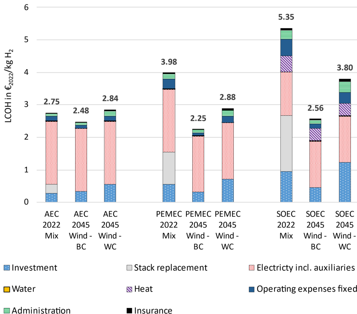
Fig. 10 LCOH results of AEC, PEMEC, and SOEC for the years 2022 and 2045
