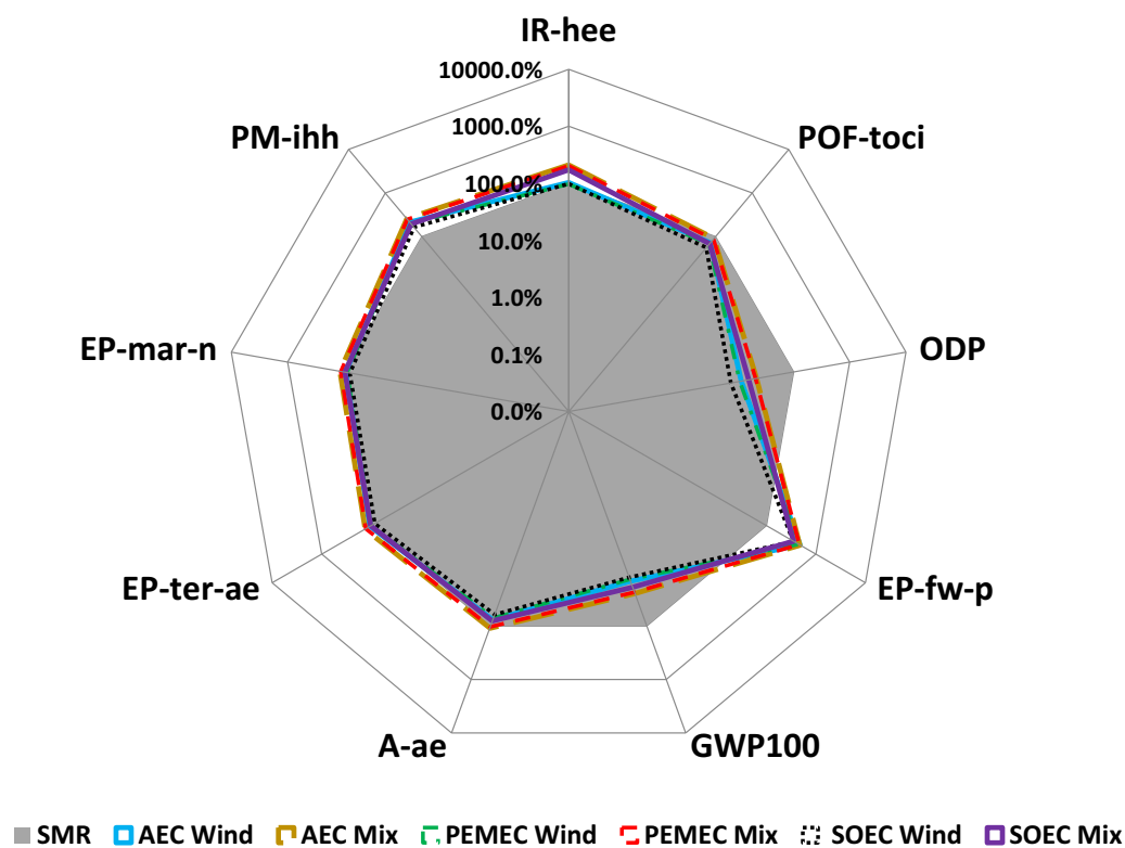
Fig. 9 Comparison of AEC, PEMEC, and SOEC with SMR for the year 2045 using several environmental indicators
