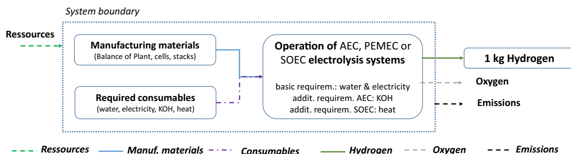
Fig. 2 System boundaries of cradle-to-gate hydrogen production; based on Koj et al. [16]
