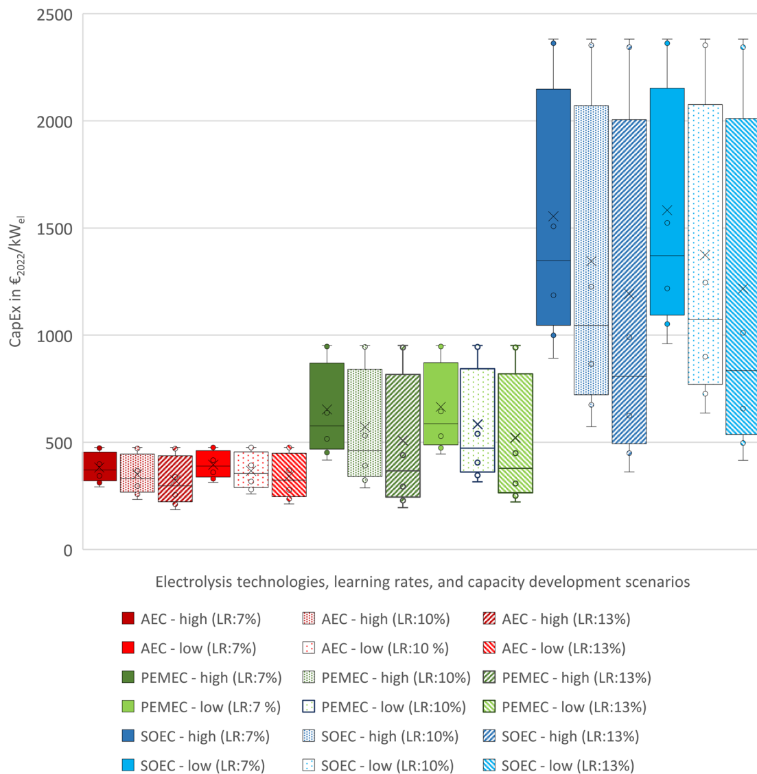
Fig. 4 CapEx of electrolysis technologies based on learning curve analysis taking into account different learning rates and capacity increases
