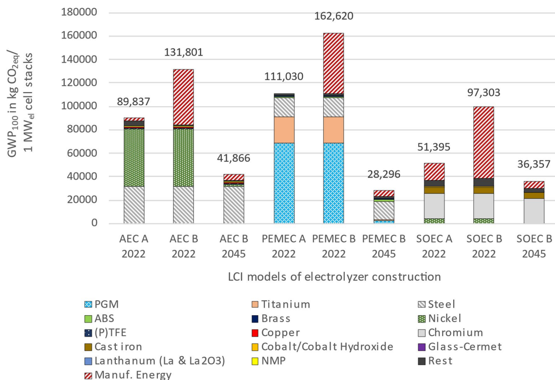
Fig. 7 GWP_{100} results for different LCI stack manufacturing and construction models
