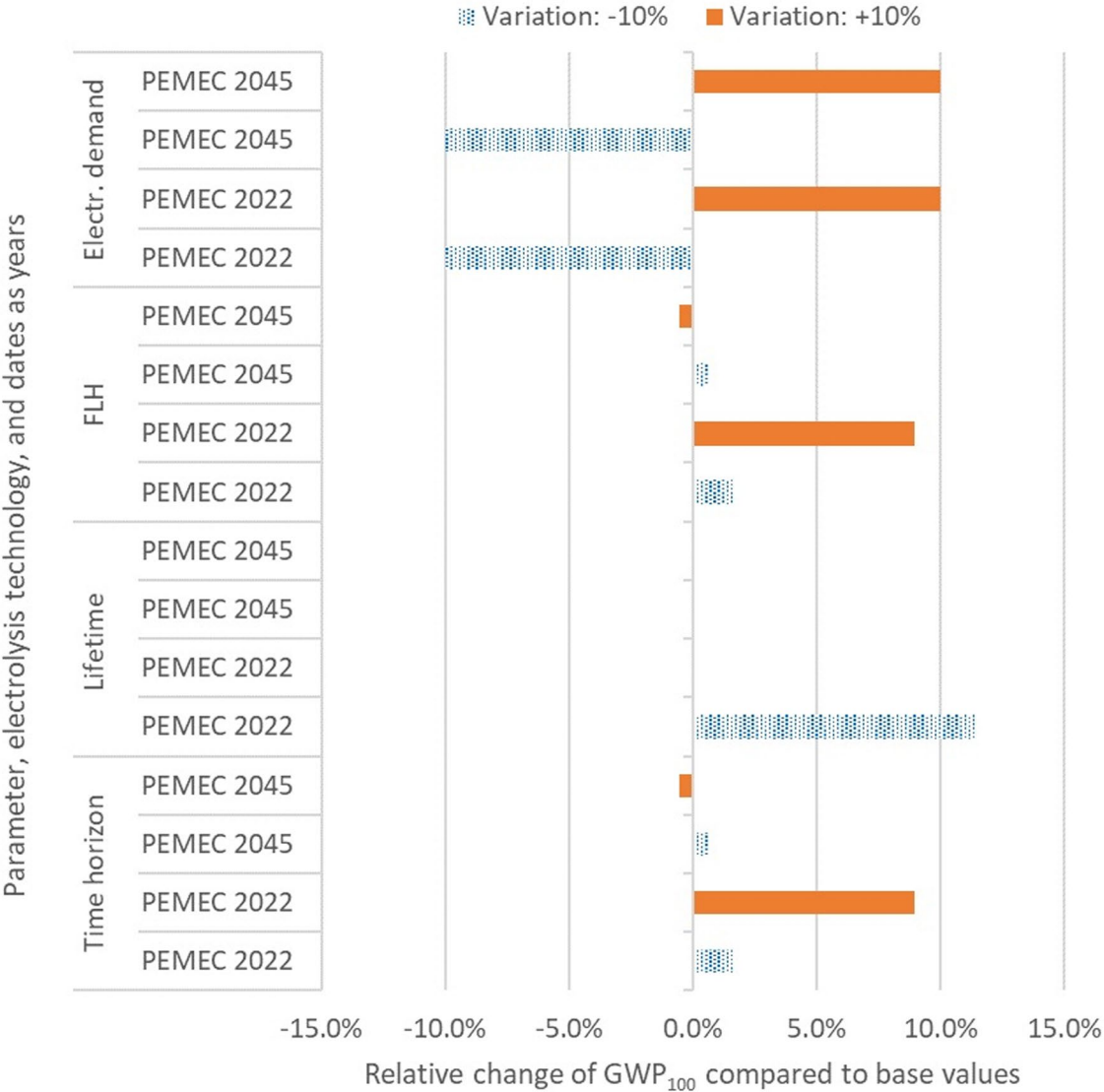
Fig. 12 Effects of parameter variations (electricity demand, FLH, lifetime, time horizon) of \pm 10\% on the GWP_{100} results for PEMEC operation with wind power
