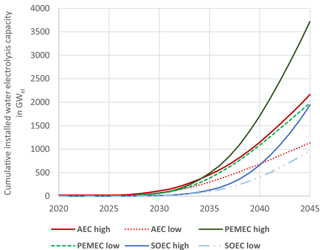
Fig. 3 Assumed cumulative installed capacities of AECs, PEMECs, and SOECs until the year 2045; based on [47, 48, 51]
