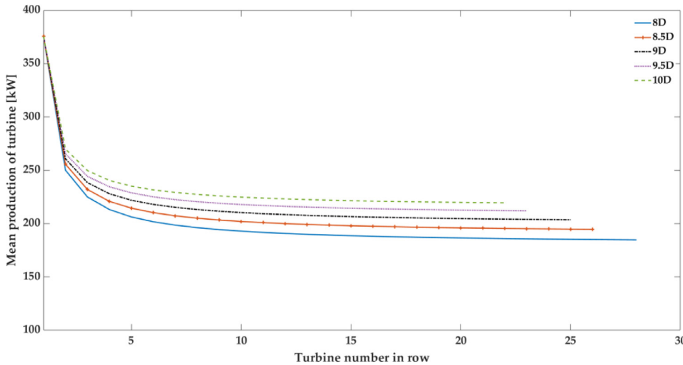
Fig. 11. Mean production of each turbine as a function of turbine number, turbine number 1 being the front wind turbine
