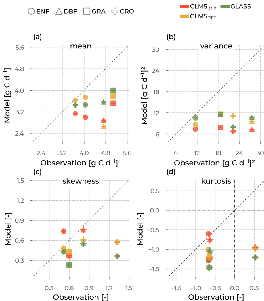
Figure 11. The mean (a), variance (b), skewness (c), and excess kurtosis (d) of the gross primary production (GPP) distributions (visualized in Fig. 10) from the models (y axis; colors, namely Community Land Model v5 (CLM5), CLM5 grid in red; CLM5PFT in yellow; and Global Land Surface Satellite (GLASS) in green), as opposed to the corresponding values from observations (x axis) aggregated for each plant functional type (marker type), namely evergreen needleleaf forest (ENF), deciduous broadleaf forest (DBF), grasslands (GRA), and croplands (CRO). The error bars are the standard errors in the respective moment, depending on the sample size.
