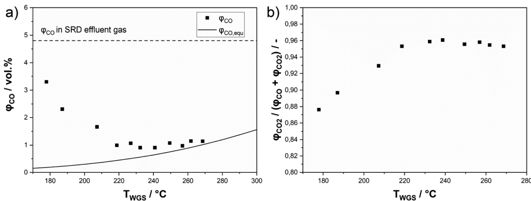
Fig. 9 Results of a water-gas-shift reactor in series with SRD: (a) CO concentrations as measured in the product stream (dotted line: CO concentration of operation without the WGS reactor; solid line: calculated equilibrium concentration of CO) and (b) carbon oxide selectivity to CO 2 at different WGS catalyst bed temperatures ( p = 2 bar(a); T_{\text{SRD}} = 400 °C; molar ratio of n_{\text{H}_2\text{O}} : n_{\text{DME}} : n_{\text{N}_2} = 5 : 1 : 1.5 ; m_{\text{In}_2\text{O}_3/\text{ZrO}_2} = 36 g (3.6 wt% indium content); m_{\gamma\text{-Al}_2\text{O}_3} = 9 g; m_{\text{WGS-catalyst}} = 10 g; GHSV = 1100 h -1 ).
