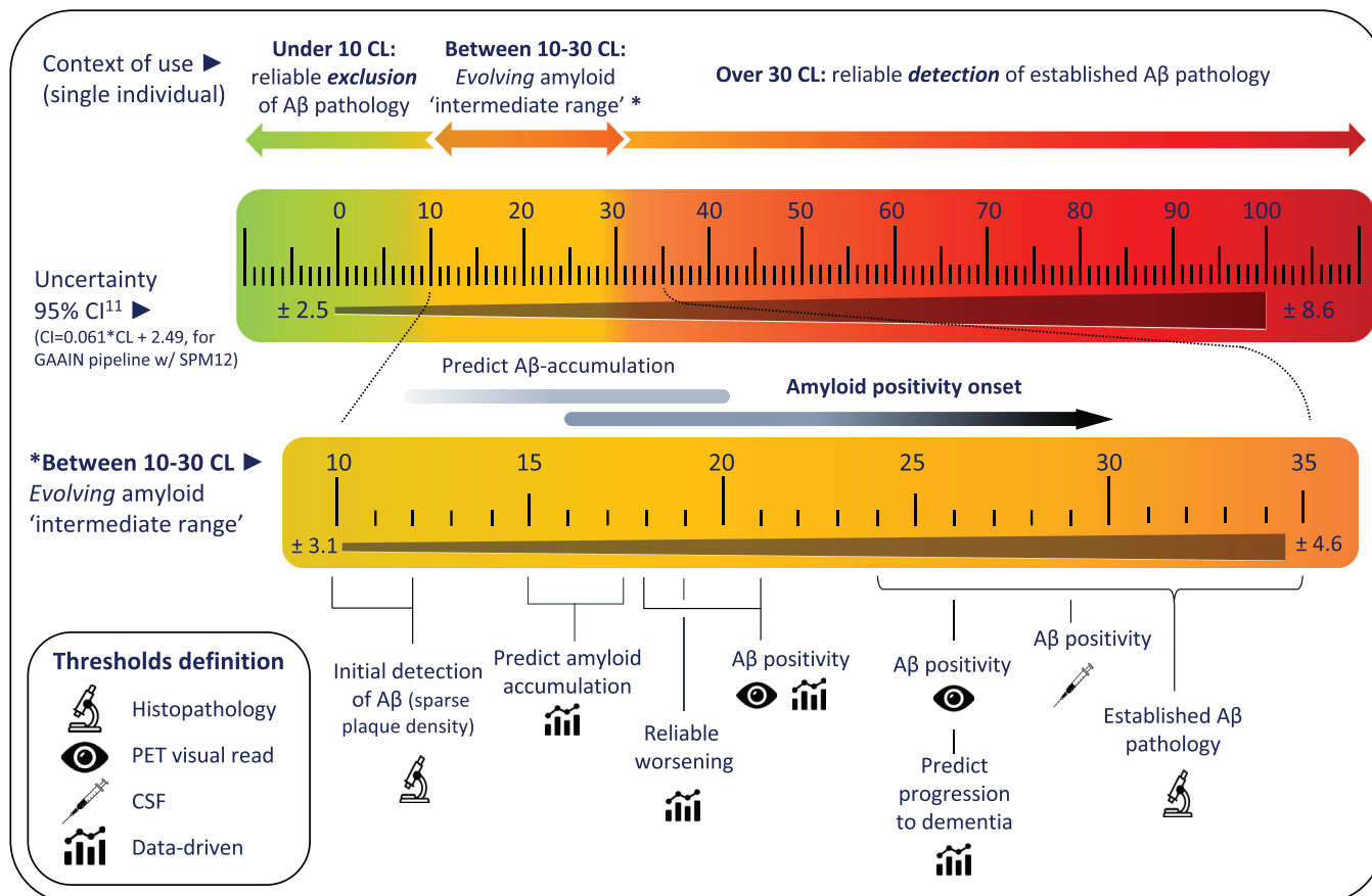
FIGURE 4 Overview of Centiloid scale interpretation. An illustrative figure summarizing the main studies regarding CL-based cut points to reliability exclude (<10 CL) and include (>30 CL) Aβ-pathology at the individual level. In addition, the 95% confidence interval across the scale is provided and detailed cutoffs in the "intermediate range" are highlighted. Aβ, amyloid-beta; CL, Centiloid; CI, confidence interval; CSF, cerebrospinal fluid; GAAIN, Global Alzheimer's Association Interactive Network; PET, positron emission tomography; SPM, Statistical Parametric Mapping.
