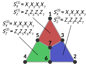
FIG. 5. The stabilizer generators of the seven-qubit color code, which encodes one logical qubit into seven physical qubits. A code state is a +1 eigenstate of all six weight-4 stabilizer generators \{S_X^{(i)}, S_Z^{(i)}\} defined on the colored plaquettes. Pauli- X ( -Z ) on all qubits corresponds to the logical operator X_L ( Z_L ), which is, up to multiplication with stabilizer generators, equivalent to weight-3 operators.
