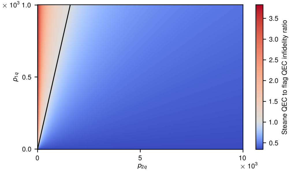
FIG. 10. The infidelity ratio from numerical simulations for Steane-type and flagged syndrome extraction in the limiting case of small two-qubit and single-qubit gate errors. All error probabilities, apart from the gate errors p_{2q} and p_{1q} , are set to p_{\text{init}} = p_{\text{meas}} = p_{\text{midcirc}} = 0 . We calculate the leading order in the infidelity for both schemes by performing fault-path counting (see Appendix B) on the respective circuits. We plot the infidelity ratio of Steane-type over flagged syndrome extraction, such that values below (above) 1 indicated in blue (red) indicate an advantage for Steane-type (flagged) syndrome extraction. The black line indicates the contour of equal infidelity of Steane-type and flagged QEC. The results of our simulations show that when the two-qubit gate error is dominant ( p_{2q} \gg p_{1q} ), Steane-type syndrome readout also offers an advantage at low physical error rates.
