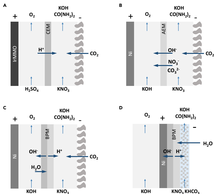
Figure 6. Reactor designs
