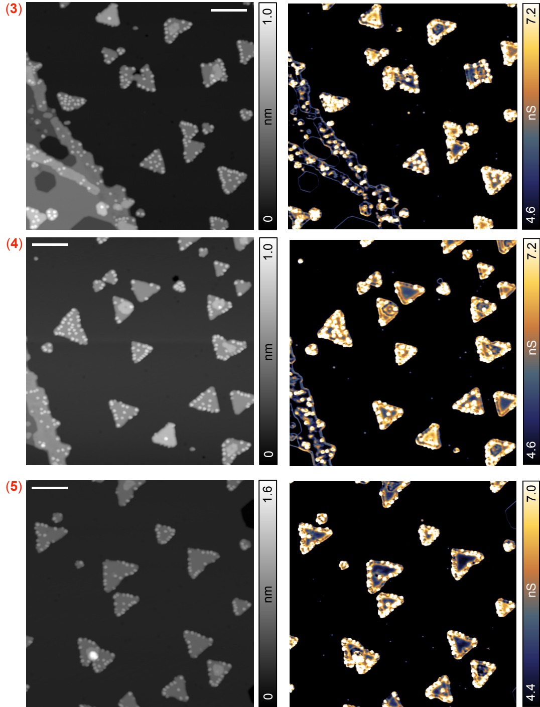
Figure A.1: Constant current topographies and corresponding dI/dV maps of scan number 3 to 5 in mosaic image presented in Figure 3.2. Data were obtained with the following parameters: V_{\text{bias}} = -620 mV, I_t = 300 pA, V_{\text{mod}} = 20 mV, f_{\text{mod}} = 752 Hz, at a temperature of 5 K, using a Co-functionalized W tip. The scale bars represent 20 nm.
