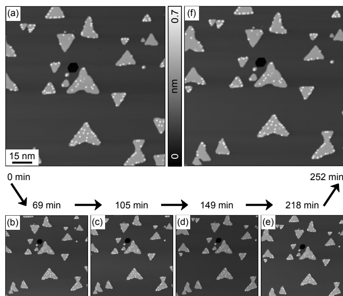
Suppl. Fig. S5 Time series at 78 K of [7]\text{H} molecules on Co nanoislands. a-f , Time series of constant-current topographic images of [7]\text{H} molecules deposited on Co nanoislands on \text{Cu}(111) at RT and imaged at 78 K. a , The first measurement of the series (0 min) and f the last after 252 min. b-e , Intermediate images of approximately the same area after 69, 105, 149, and 218 min, respectively. No molecular motion is observed. Slight shifts of the field of view are due to thermal drift, which was compensated for as best as possible by manually tracking the sample ( V_{\text{bias}} = 500 \text{ mV} , I_t = 100 \text{ pA} , 78 K, W tip).
