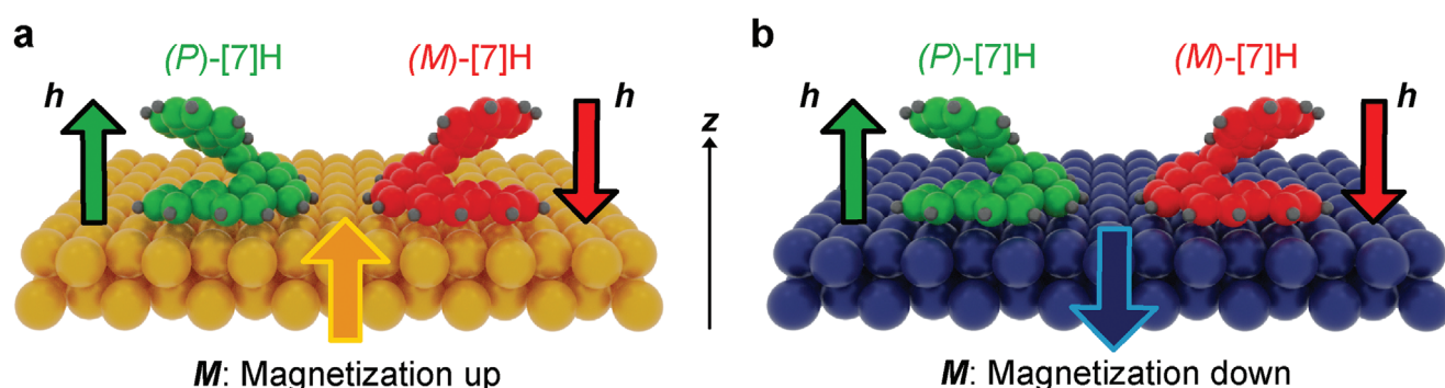
Figure 3. Adsorption configurations of [7]H on Co nanoislands. Both enantiomers, (P) -[7]H and (M) -[7]H, can adsorb on Co nanoislands with both a) magnetization up ( M = \uparrow ) or b) magnetization down ( M = \downarrow ). The pitch vectors of the molecular helices h = \uparrow (green) and h = \downarrow (red) represent (P) -[7]H and (M) -[7]H enantiomers, respectively (see Section S1, Supporting Information).
