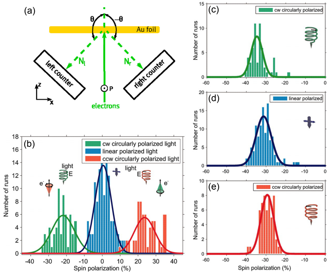
Figure 1.4: (a) Schematic sketch of a Mott electron polarimeter setup. (b) Spin polarization measured for electrons emitted from bare Au(111) with clockwise (cw) (green) and counterclockwise (ccw) (red) circularly polarized light, and with linearly polarized light (blue). The polarization is -22 , +22 , and 0\% , respectively. The longitudinal spin polarization is measured; the spin is oriented parallel (green) or antiparallel (red) to the direction of propagation of the electron. (c-e) Spin polarization of electrons transmitted through 50-bp dsDNA/Au(111). The polarizations were -35 , -31 , and -29\% for light polarized cw circularly [(c), green], linearly [(d), blue], and ccw circularly [(e), red], respectively. Figures adapted from Ref. [8]
