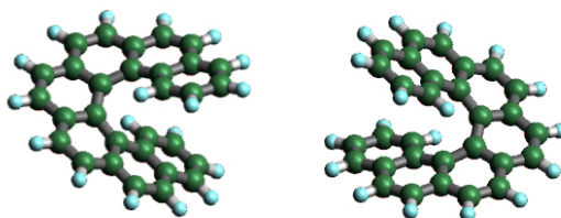
Figure 1.2: Schematic representation of the ( M )-[7]H (left side of the figure) and ( P )-[7]H (right side of the figure) molecules.
