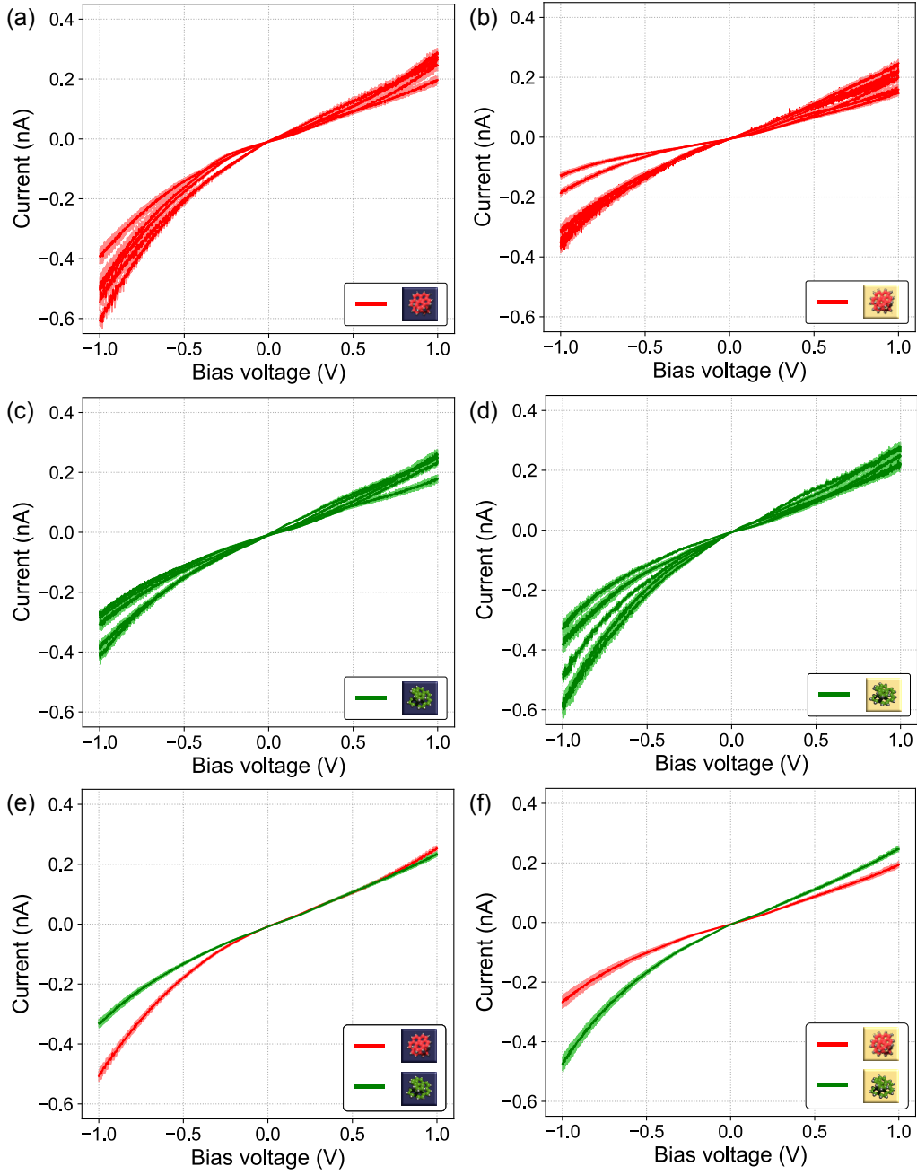
FIG. S2. I - V curves of molecules adsorbed on two oppositely magnetized Co islands. (a) and (c) Five single-molecule I - V curves of individual (M) -[7]H and (P) -[7]H molecules on the dark island, respectively. (b) and (d) Five single-molecule I - V curves of individual (M) -[7]H and (P) -[7]H molecules on the bright island, respectively. (e) and (f) Averaged I - V curves of the five molecules each with the same handedness on dark and bright islands, respectively. All I - V curves were obtained with a non-magnetic STM tip ( V_{\text{stab}} = 2 \text{ V} and I_{\text{stab}} = 800 \text{ pA} ). The dark lines represent the averaged I - V curves, while the light-colored regions indicate the calculated standard errors.
