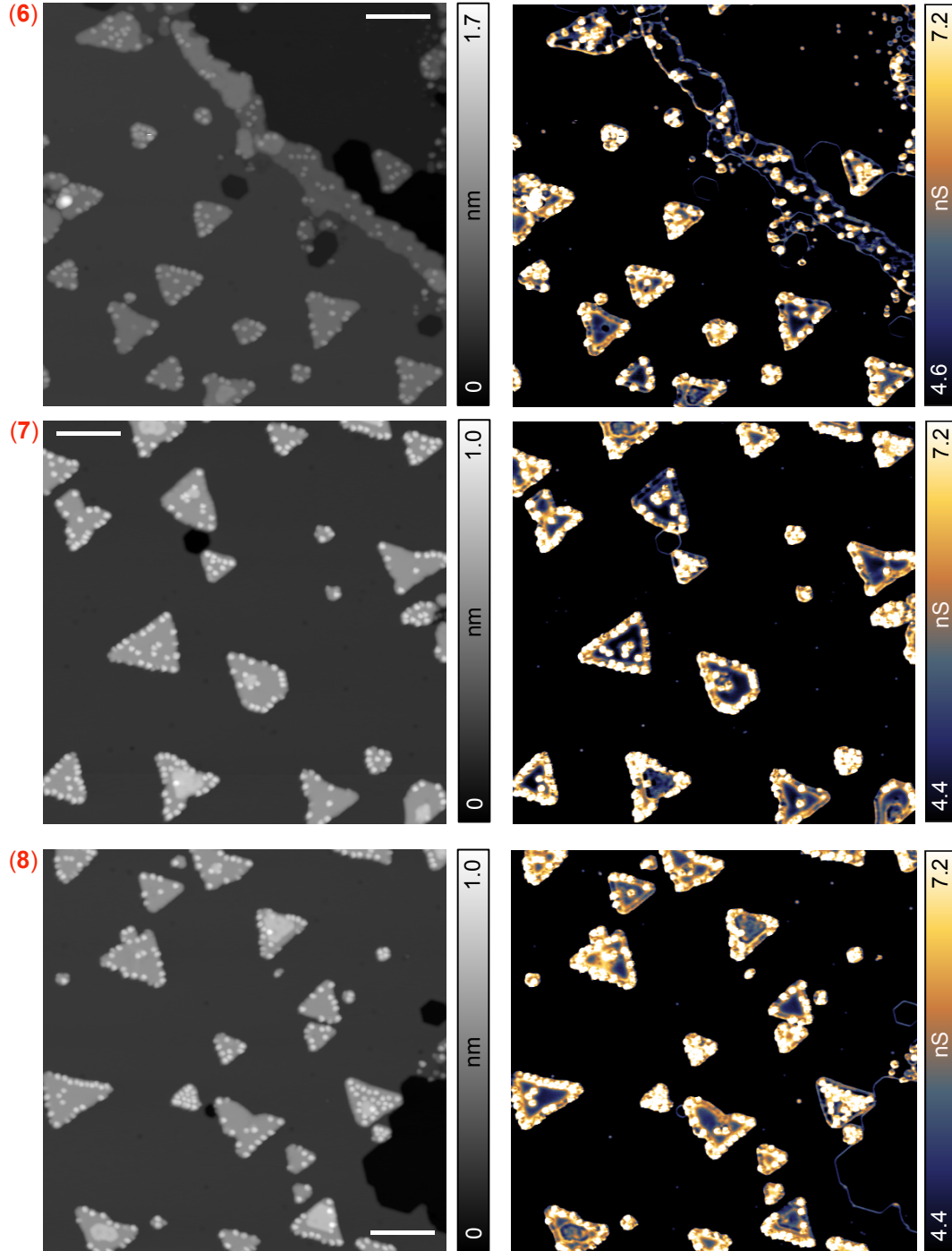
Figure A.2: Constant current topographies and corresponding dI/dV maps of scan number 6 to 8 in mosaic image presented in Figure 3.2. Data were obtained with the following parameters: V_{\text{bias}} = -620 mV, I_t = 300 pA, V_{\text{mod}} = 20 mV, f_{\text{mod}} = 752 Hz, at a temperature of 5 K, using a Co-functionalized W tip. The scale bars represent 20 nm.
