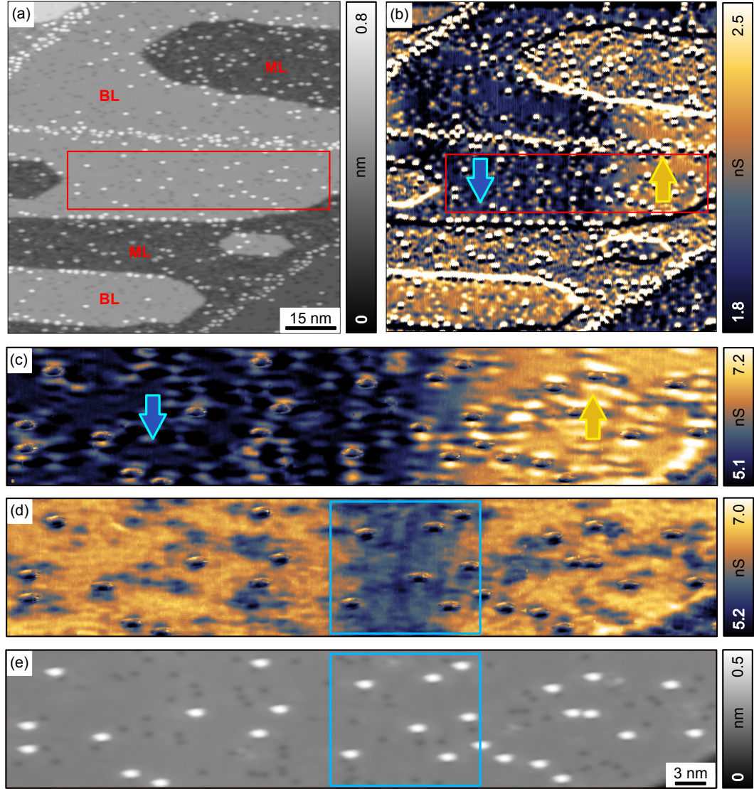
Figure 3.3: (a) Constant-current STM topography of (M) -[7]H molecules on a substrate of 1.7 ML of Fe on W(110), where BL and ML denote the first and second ML of Fe, respectively. (b) dI/dV map acquired simultaneously with (a), displaying opposite alignments of the OOP magnetized domains in the BL region, indicated by blue and yellow arrows ( V_{\text{bias}} = -100 mV and I_t = 150 pA, V_{\text{mod}} = 20 mV, f_{\text{mod}} = 752 Hz). (c) and (d) High-resolution dI/dV maps of the area marked by a red frame in (b), measured at V_{\text{bias}} = -100 mV and I_t = 450 pA and V_{\text{bias}} = 50 mV and I_t = 250 pA, respectively. The blue frame in (d) marks the approximate location of the magnetic domain wall. (e) High-resolution constant-current topography of the region outlined in red frame in (a) and (b), with a blue frame indicating the molecules deposited on the domain wall ( V_{\text{bias}} = 50 mV, I_t = 250 pA). All STM data were obtained at 5 K using a Fe-functionalized W tip.
