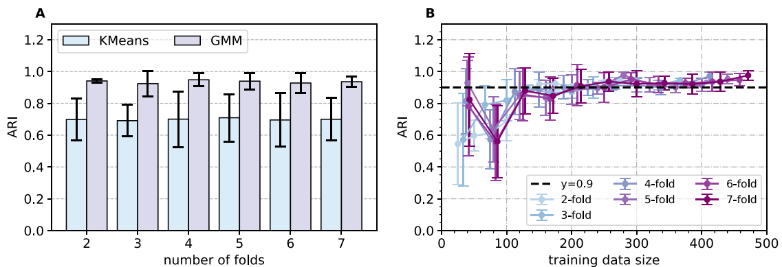
FIGURE 8 k -fold cross validation results of CuCr60. (A) the performance of two unsupervised models, KMeans and GMM, measured by the ARI value and as a function of the number of folds of the k -fold cross-validation. (B) ARI values of k -fold cross-validation using GMM with varying the amount of training data.
