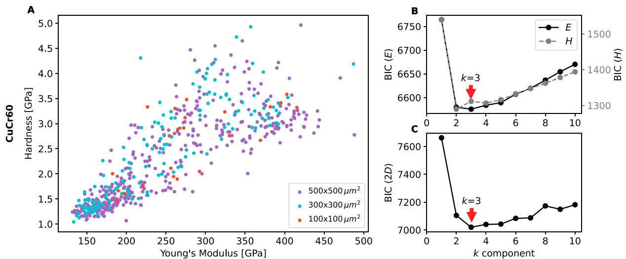
FIGURE 7 (A) Distribution of the CuCr60 data over the depth range of 500–2,000 nm (combined datasets for indentation arrays of 100 × 100 μm 2 , 300 × 300 μm 2 , and 500 × 500 μm 2 ) (B) 1D BIC for E and H , and (C) 2D BIC for E and H .
