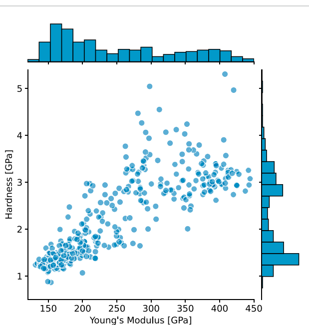
FIGURE 2 Scatter plot with marginal histograms of all obtained values for Young's modulus and hardness measured for CuCr60 at an average indentation depth of 1 \mu\text{m} .
