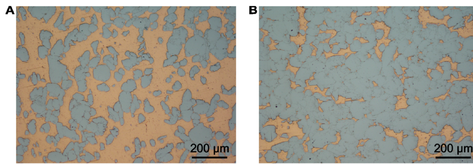
FIGURE 1 Optical micrographs of Cu-Cr composites produced by field-assisted sintering technique with (A) 25 wt% Cr, (referred to as CuCr25), and (B) 60 wt% Cr (referred to as CuCr60) were investigated by indentation.
