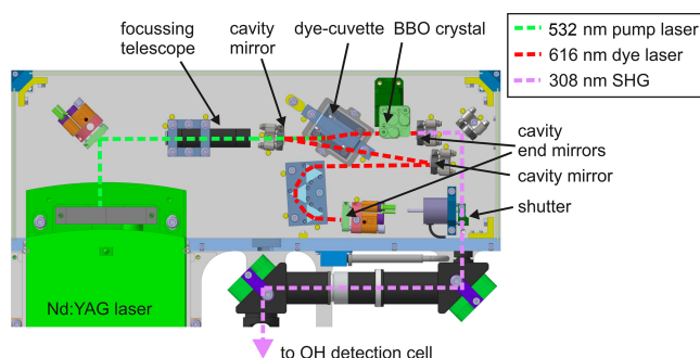
Figure 2. Schematic of the simplified dye laser system (wavelength 616 nm) pumped by a commercial Nd : YAG laser (wavelength 532 nm) used for the OH detection. The dye laser cavity consists of the two end mirrors and two additional mirrors that fold the beam path of the cavity. The dye cuvette is positioned at the Brewster angle. Prisms are used to select the wavelength of the dye laser, which can be tuned by the horizontal position of the end mirror, which is mounted in a motorised mirror mount. The dye laser radiation is frequency converted to a wavelength of 308 nm by a BBO crystal inside the laser cavity. The UV light is directed to the detection cell in a lens tube system via deflection mirrors (Fig. 1).
