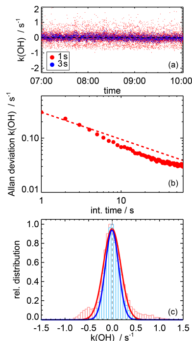
Figure 4. Allan deviation plot (b) of OH reactivity measurements (a) from measurements after subtracting the zero reactivity value in a mixture of humidified synthetic air (water vapour mixing ratio: 1.5 %) with ozone (60 ppbv). The dashed line gives the Allan deviation expected from Gaussian noise. The distribution (c) of zero measurements for 1 s data (red) shows deviations from a Gaussian distribution (lines) that are reduced when three traces are summed before the single exponential fit is applied (blue).
