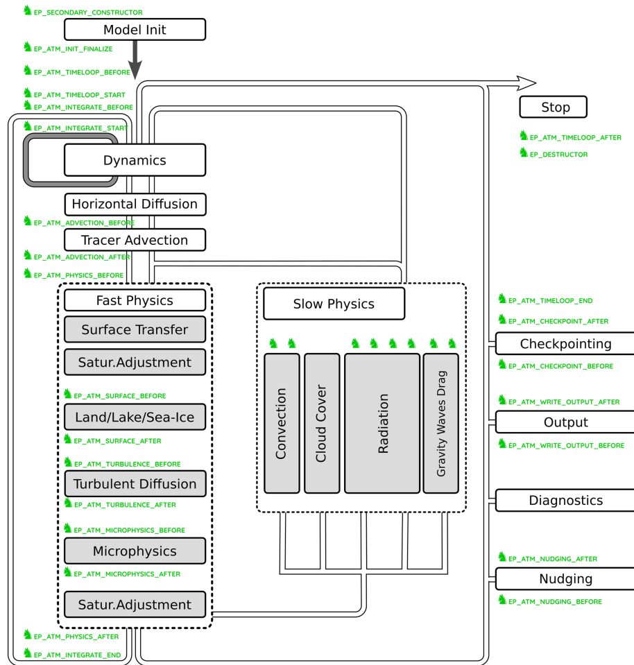
Figure 2. Schematic representation of the integration of entry points into the ICON control flow. At specific entry points, plugin subroutines can be called from within ICON if they have been registered for these entry points through the ComIn library. After initialisation, the model's integration is conducted in a time loop (main part of the schematic). The time integration can be divided into three parts: (i) the dynamical core “sub-stepping” (dark grey) with a time step shorter than \Delta t , (ii) the fast-physics process loop with the models basic time step \Delta t , and (iii) the slow-physics process loop with a larger time step than \Delta t depending on the slow-physics process. Entry points are marked in green, and for some, names are provided. The naming scheme and placement are further discussed in Sect. 3.6, and the white paper (see e.g. in the Supplement) provides a full list of entry points.
