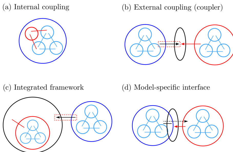
Figure 1. Overview of model extension methods. In each approach one ESM component acts as the host model (blue circle with smaller light blue circles indicating internal functionalities like parameterisations and dynamical core), which can be extended by these four methods. Extensions are highlighted in red, and software to support these extensions in approaches (b) to (d) is represented by black circles and ellipses. Red circles are set around new ESM components (approach b–d) or smaller extensions (approach a). Straight lines indicate exchange of data and access to routines. An arrow is added if access to routines between components is only possible one way. For example software A can call routines of software B but not vice versa, where software A could be an ESM component and software B a coupler. In this case, the arrowhead is located at software B (the coupler) to indicate the software of which routines are called. Dashed red rectangles indicate that additional infrastructure is required for each host-model component when it becomes connected to the coupler or IF for the first time but that the corresponding coding effort is only required once. The red line in approach (c), connecting the new component and the IF, indicates that the component needs to be integrated into the IF. For a model-specific interface (approach d) the dot-dashed line from the host model to the new component visualises the fact that routines are called but only indirectly via the interface itself (callback mechanism introduced in Sect. 2).
