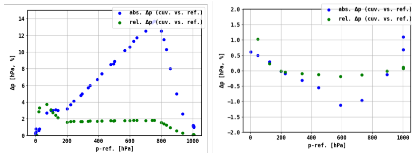
Figure 3 Comparison of CAR-O3 air pressure sensor (inside UV-absorption cuvette) against accurate pressure sensor (Omega, HHP360, uncertainty: 0.25 hPa) before (left diagram) and after (right diagram) solving the electronic artifact of the AD-converter (details see main text). Displayed are the pressure differences in hPa (blue dots) and their relative differences in % (green dots).
