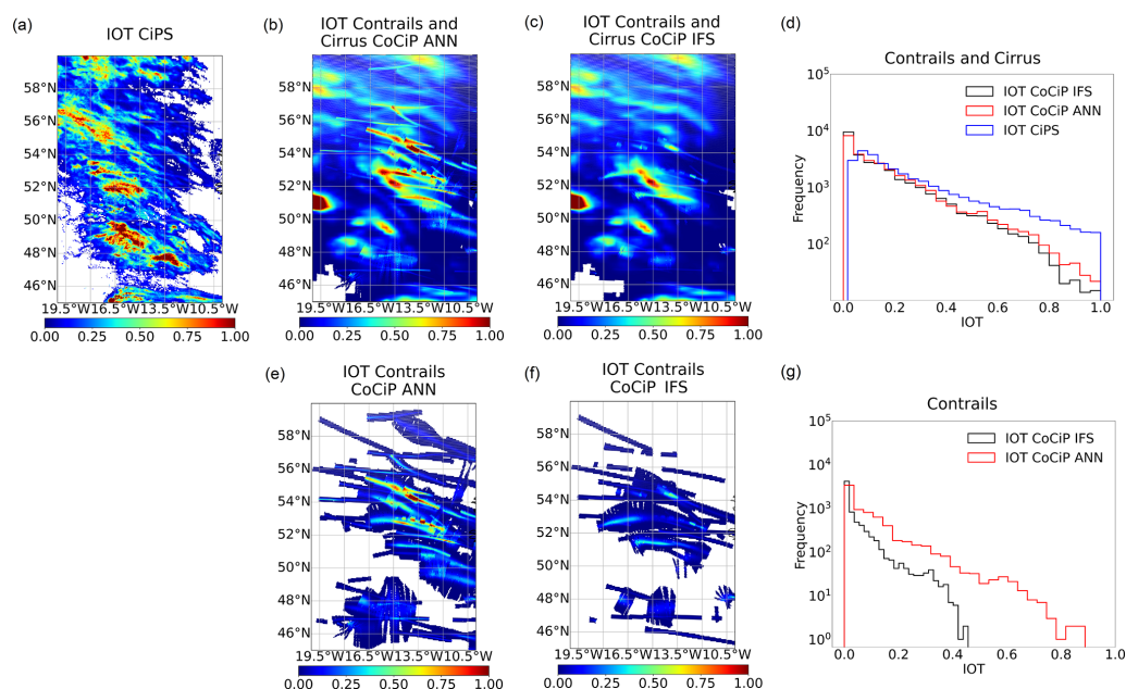
Figure 7. Distributions of IOT for contrails and cirrus retrieved from (a) MSG observations using the CiPS algorithm and simulated using the CoCiP model with (b) q_{ANN} or (c) q_{IFS} at 10:00 UTC on 14 April 2021. The IOT distribution for contrails from CoCiP simulations is shown in (e) and (f). The linear structures of contrails correspond to the associated flight tracks. The IOT frequencies (histograms) for contrail cirrus and contrails are shown in (d) and (g), respectively.
