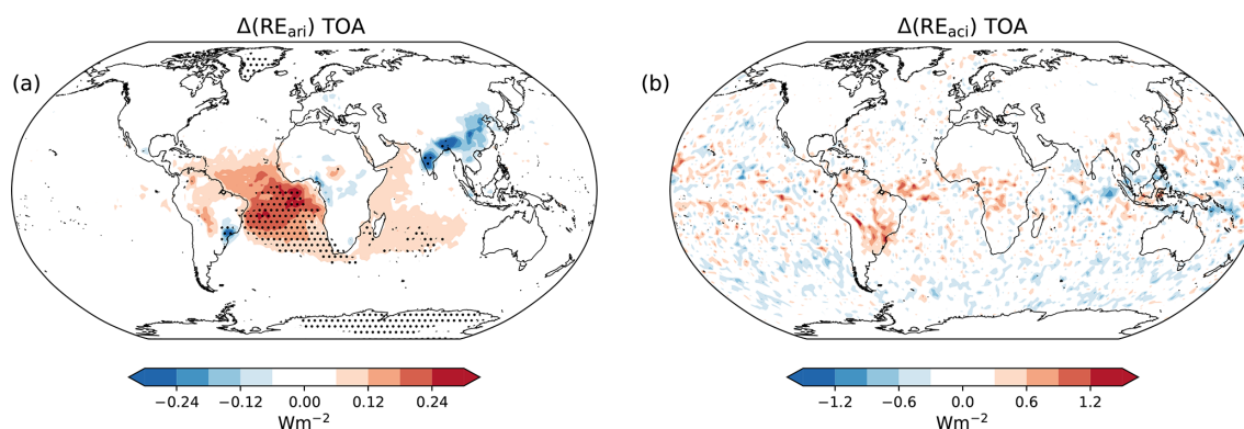
Figure 7. Aerosol and cloud radiative effects mediated by aerosol changes from the deforestation (DCGL – PNV) scenario. Panels ( a ) and ( b ) show the top-of-the-atmosphere (TOA) direct radiative effect (ARI) and indirect radiative effect (ACI), respectively. A dotted pattern is used to highlight areas with statistically significant differences, based on a two-tailed Student's t test with a 90 % confidence level.
