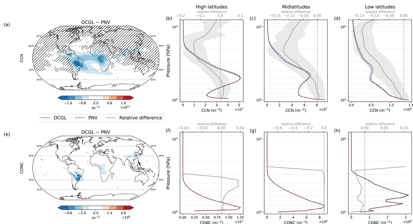
Figure 6. Changes in cloud condensation nuclei (CCN) at 0.2 % supersaturation ( a–d ) and cloud droplet number concentration (CDNC) ( e–h ). Panels ( a ) and ( e ) show the spatial differences in the total column burden (the number of particles per square metre) for CCN and CDNC, respectively, emerging from the DCGL scenario as compared to natural vegetation (DCGL – PNV). Panels ( b )–( d ) and ( f )–( h ) show vertical profiles of total column data from the DCGL and PNV simulations, along with their relative differences. The figure details are the same as those in Fig. 5; however, the grey area representing 1 standard deviation of the spatio-temporal mean is depicted only in panels ( b ), ( c ), and ( d ). In panel ( e ), a dotted pattern is used to highlight areas with statistically significant differences.
