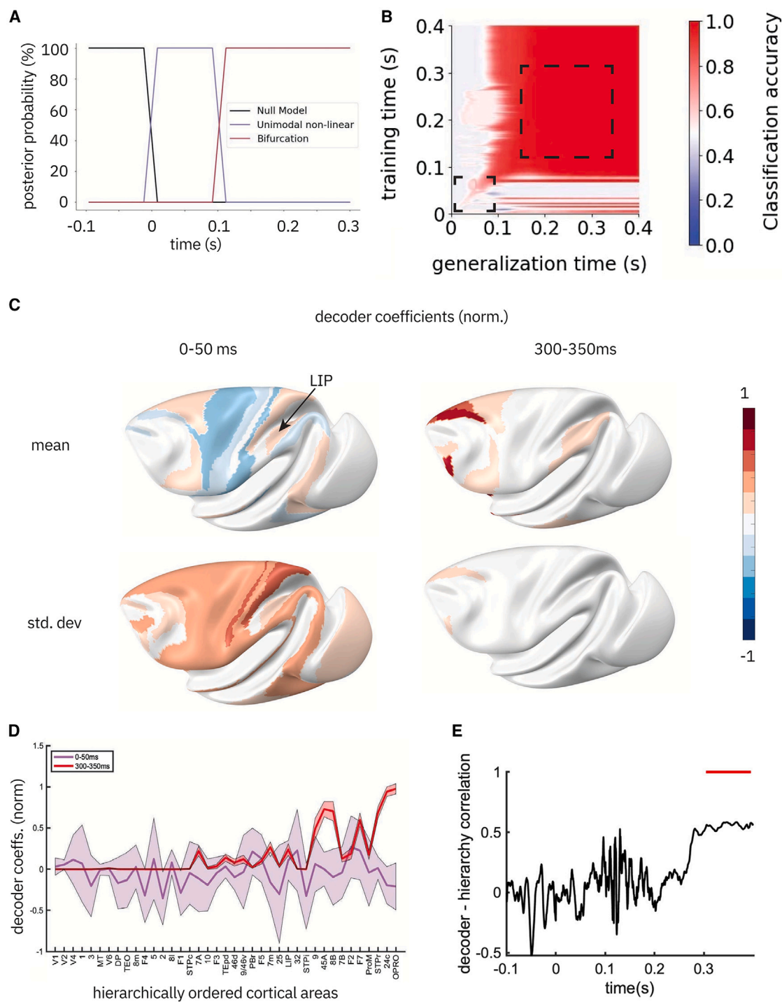
Figure 3. A dynamic-to-sustained progression of activity states associated with ignition
