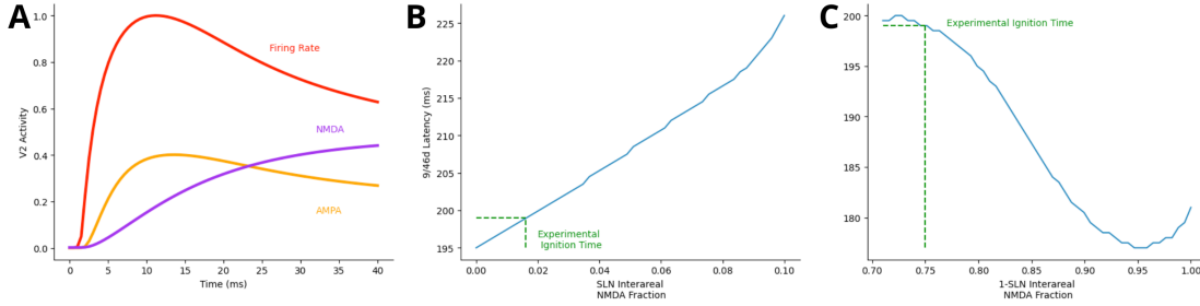
Supplemental Figure 1. Dynamics of AMPA and NMDA Receptor Activity and Their Impact on Ignition Timing Across Inter-Areal Connections A) The dynamics of activity in area V2 (normalized firing rate) reflects the distinct dynamics of AMPA and NMDA receptors at feedforward and feedback connections. B) Impact of Receptor Type on Ignition Timing. Ignition times (time to reach 95% of peak dLPFC activity) vary with the fraction of NMDA receptors in inter-areal connections from B) SLN projections and C) 1-SLN projections.
