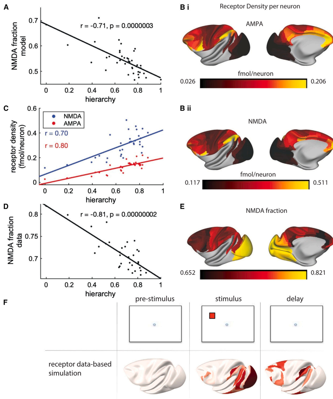
Figure 6. The NMDA/AMPA ratio decreases along the cortical hierarchy and supports ignition
