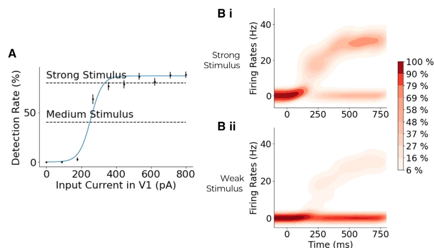
Figure 2. A sigmoidal relationship between stimulus intensity and detection probability
