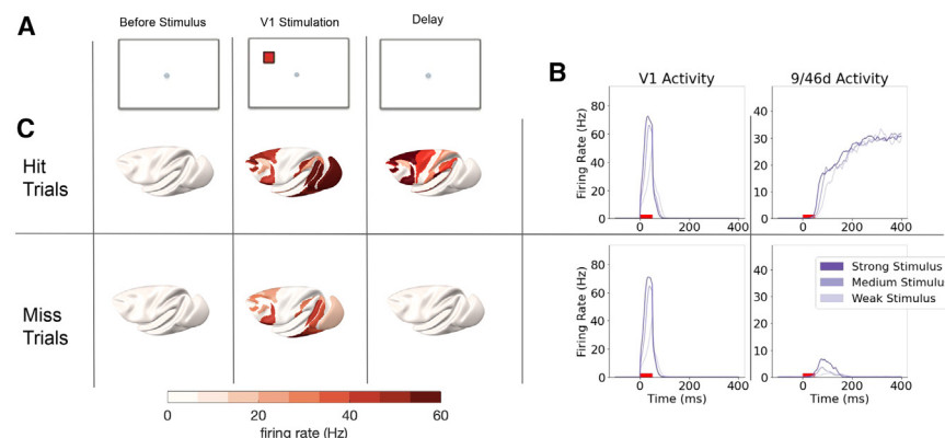
Figure 1. Stimulus detection is accompanied by widespread ignition of activity throughout the frontoparietal network
