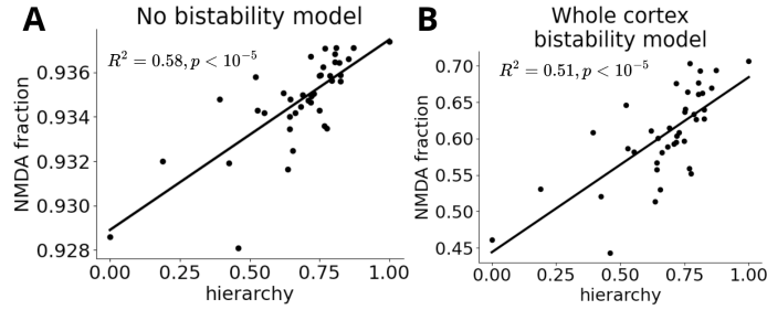
Supplemental Figure 2. NMDA Fraction Along the Cortical Hierarchy in Alternative Models For both alternative models, the fraction of excitatory inputs via NMDA receptors (compared to total NMDA+AMPA inputs) increases along the cortical hierarchy.
