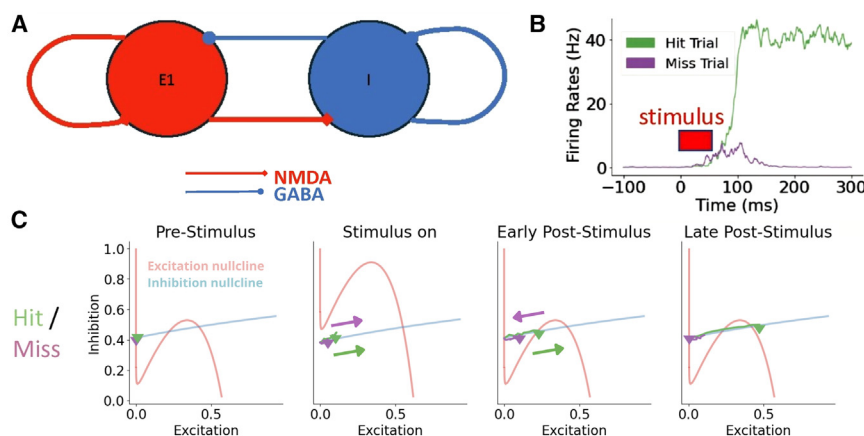
Figure 4. A dynamic bifurcation mechanism for ignition underlies stimulus detection
