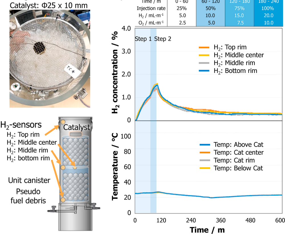
Fig. 7. Catalyst configuration and arrangement #1: Center Top.
