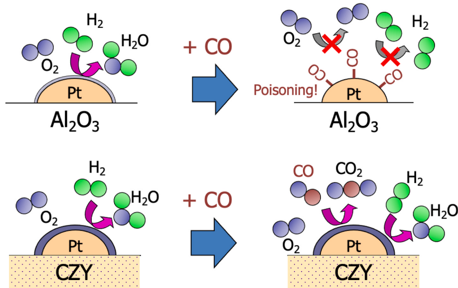
Fig. 12. Image diagram of reaction termination due to CO poisoning in Pt/ Al_2O_3 catalysts, and hydrogen recombination overcoming CO poisoning in Pt/CZY catalysts.
