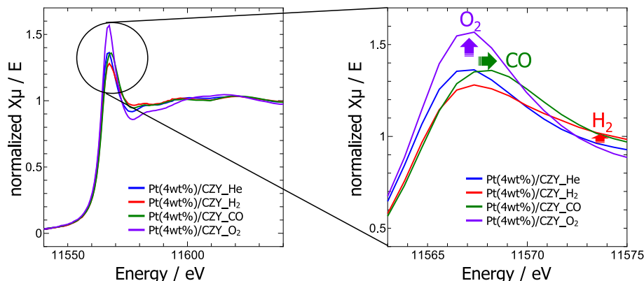
Fig. 10. Pt L_{III} -edge XANES spectra of Pt/CZY under individual gas atmospheres at room temperature.
