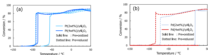
Fig. 3. Cryogenic activity of pre-reduced and pre-oxidized catalysts, (a) Pd/Al 2 O 3 and (b) Pt/Al 2 O 3 .
