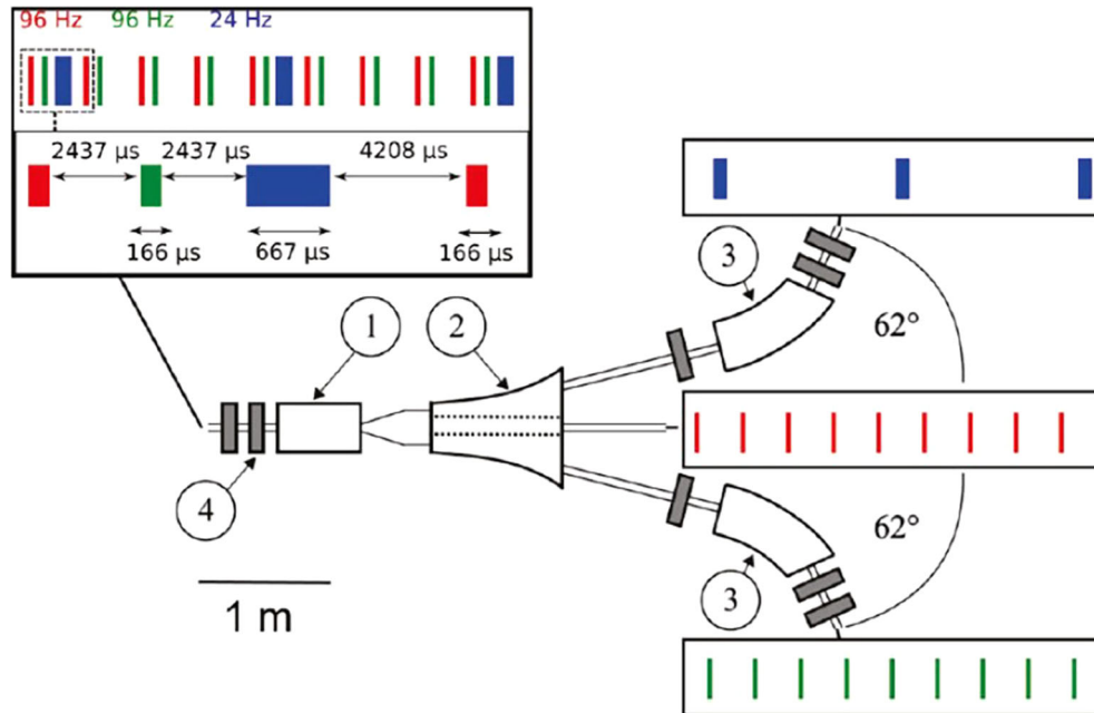
Figure 3. Schematic outline for the design of the HBS multiplexer system. 14 1: Bipolar kicker magnet, 2: Septum magnet with three different field regions, 3: 45° sector bending magnets, 4: Quadrupole magnets (all in grey). After the multiplexer the proton pulses are split into three beam trails with a tilt of \pm 62^\circ . The timing scheme of the pulse sequence is shown: red and green with two 96 Hz pulses of 167 \mu s length, blue with one 24 Hz pulse of 667 \mu s length. 9 Adapted with kind permission by Forschungszentrum Jülich GmbH.
