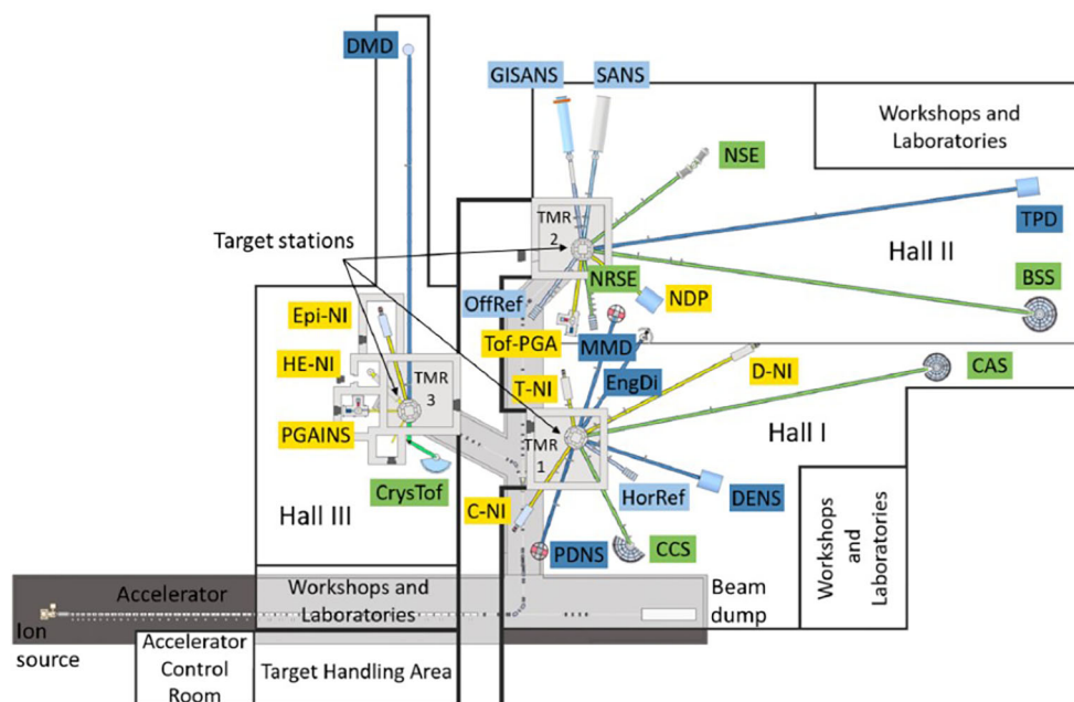
Figure 7. HBS facility as proposed with three target stations and 24 instruments. The acronyms of the instruments correspond to those in Table 1. 24 Adapted with kind permission by Forschungszentrum Jülich GmbH.
