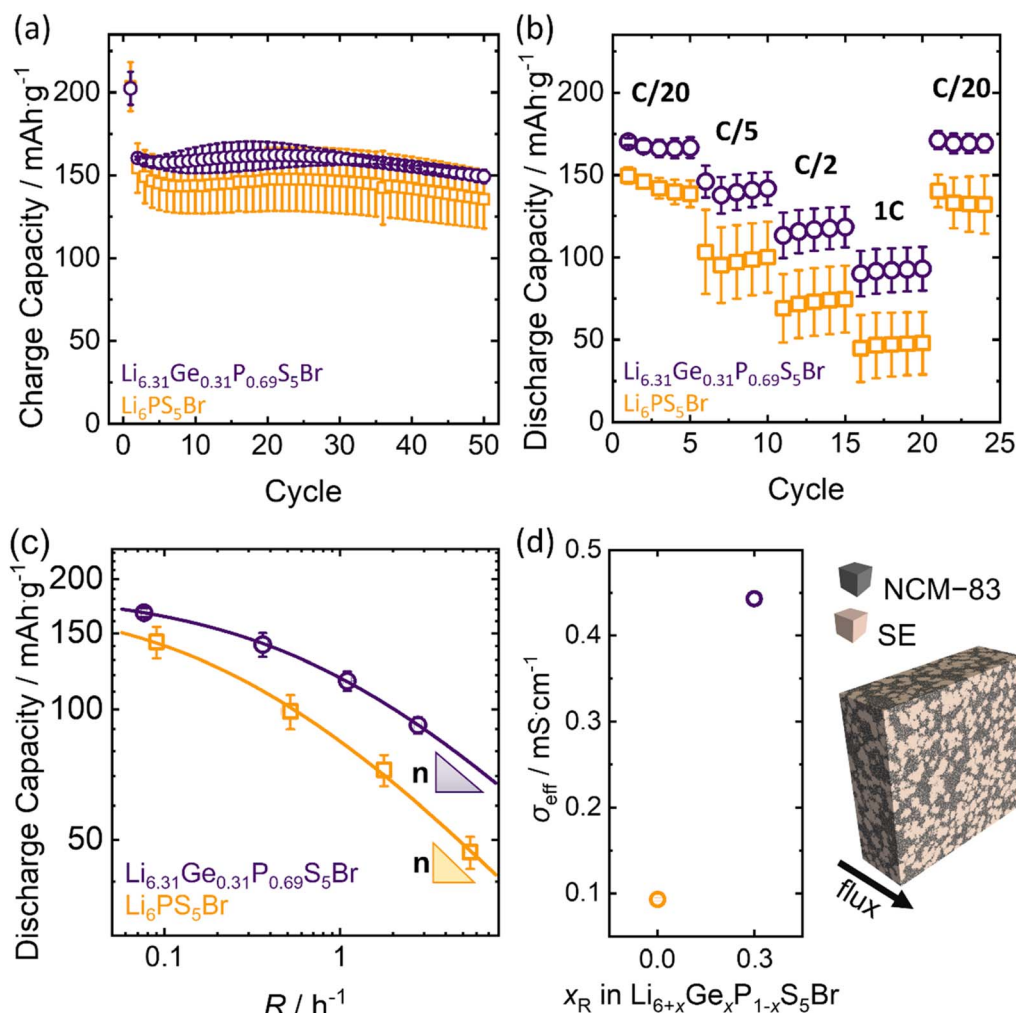
Fig. 7 Cell performance of In/LiIn| \text{Li}_{5.5}\text{PS}_{5.5}\text{Cl}_{1.5} |NCM-83 : \text{Li}_{6+x}\text{Ge}_x\text{P}_{1-x}\text{S}_5\text{Br} , for x = 0 and x = 0.31 in half-cell setups. (a) Charge capacities for 50 cycles at 0.1C. (b) Discharge capacities of rate-performance test show that \text{Li}_{6.31}\text{Ge}_{0.31}\text{P}_{0.69}\text{S}_5\text{Br} exhibits enhanced rate-stability. (c) Capacity retention of both systems as a function of the practical rate R . Fits corresponding to the model proposed by Tian et al. 55 are given as lines. All errors are calculated from triplicate measurements. (d) Exemplary virtual composite, representing an NCM-83|SE electrode of size 60 \mu\text{m} \times 180 \mu\text{m} \times 180 \mu\text{m} and effective ionic conductivities as obtained from the resistor network model.
