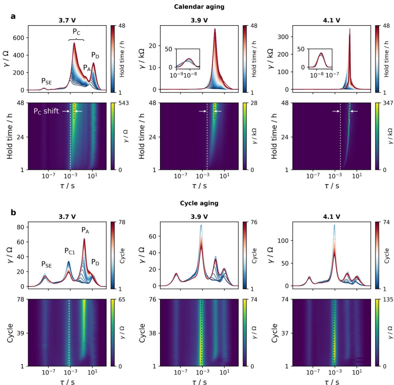
Figure 5. DRT evolution and corresponding 2D DRT surfaces (a) during potentiostatic hold and (b) at end of discharge of cycles in high C-rate regime. In 2D DRT, the maximum value displayed on each color bar represents approximately the highest DRT intensity and the dashed lines indicate the relative position of P_C peak. Data from all investigated cut-offs with Nyquist and Bode plots can be found in Figure S6-9 .
