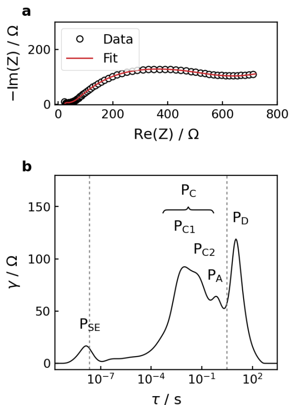
Figure 4. (a) Typical Nyquist plot with DRT fit and (b) respective DRT analysis of the impedance data. The dashed lines in the DRT mark the high- and low-frequency boundaries of the measured range in EIS.
