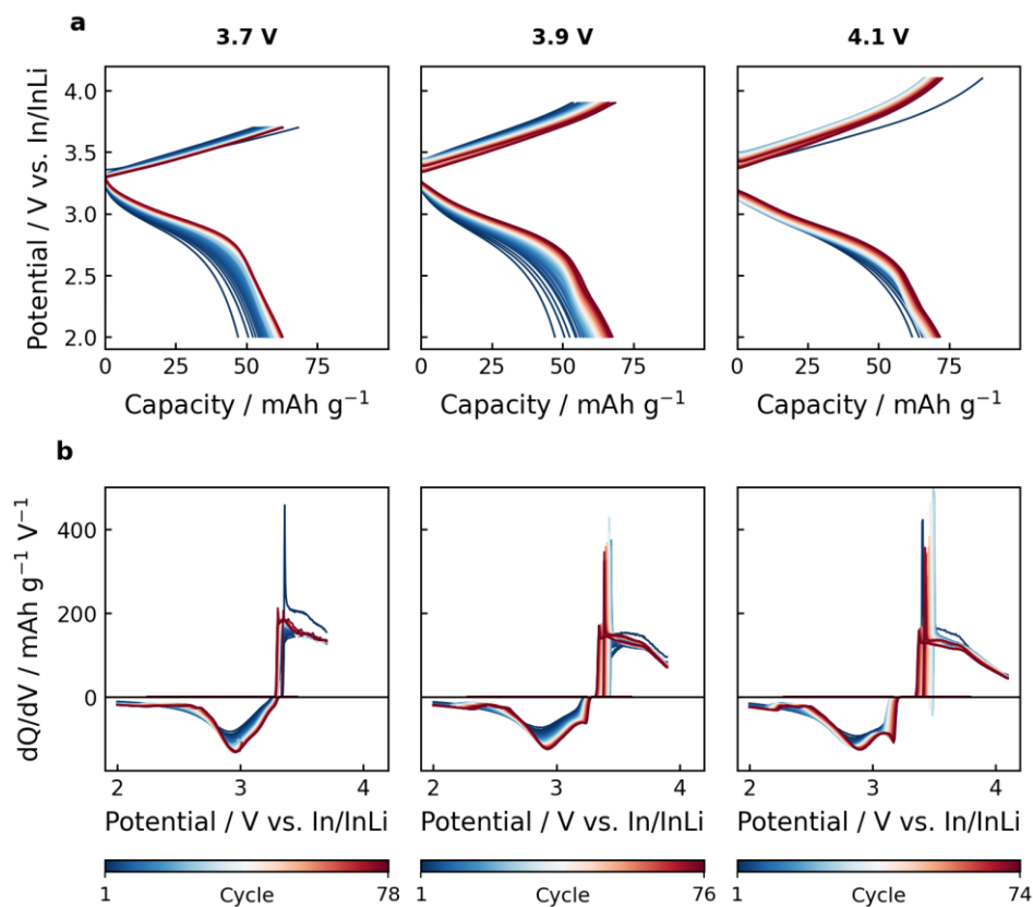
Figure 7. (a) Galvanostatic charge-discharge curves and (b) corresponding differential capacity plots during accelerated cycle aging (1C cycling) periods. Data from accelerated calendar aging periods and all investigated cut-offs can be found in Figures S12-S14 .
