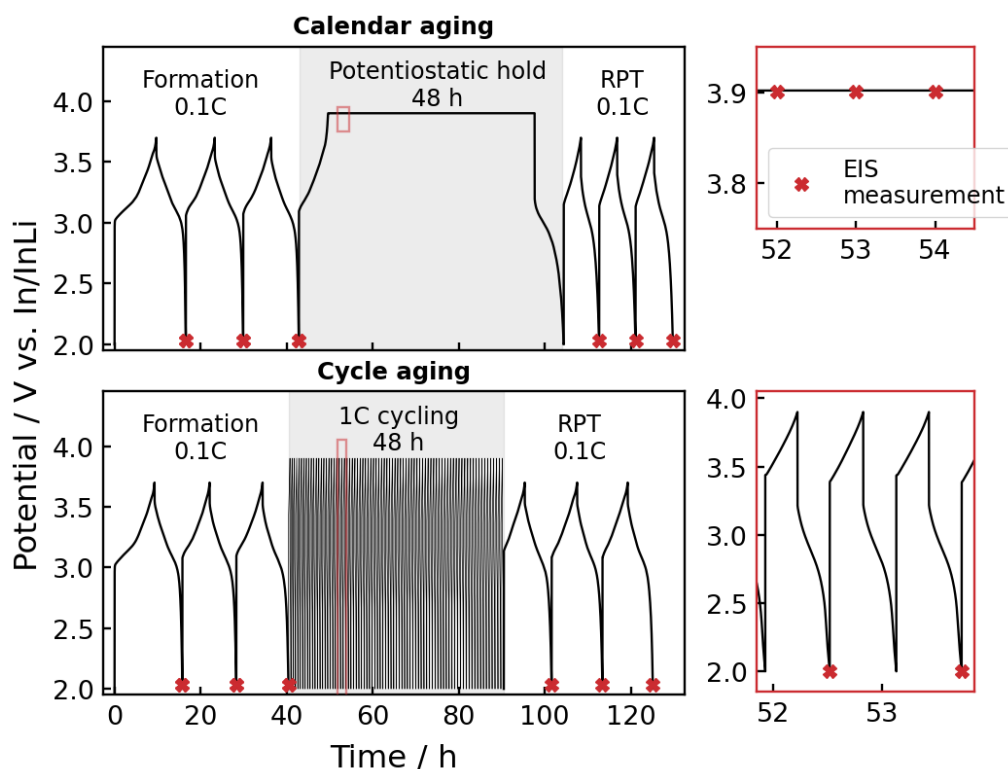
Figure 1. Example of cell potential profiles during accelerated aging protocols. Formation and reference performance test (RPT) steps are fixed in all experiments with a variation of upper cut-off potential in aging periods (grey field). Cross mark (X) symbols represent points where EIS measurement was recorded. An EIS measurement was implemented every hour during potentiostatic hold and end of discharge of every two cycles during 1C cycling. For formation and RPT steps, EIS was measured at the end of discharge for every cycle.
