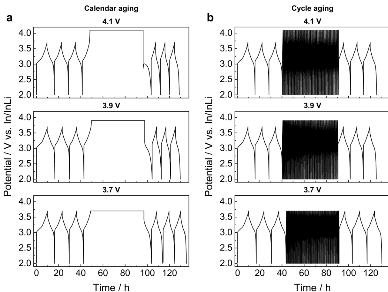
Figure 2. Potential versus time profile of accelerated (a) calendar aging and (b) cycle aging cells at different cut-offs. Data from all investigated cut-offs can be found in Figure S1 .
