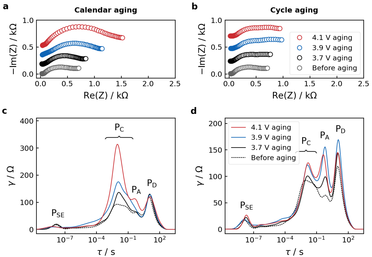
Figure 6. Data measured at the last formation cycles (before aging) and last RPT cycles (aging). (a-b) Nyquist plots and (c-d) DRT of calendar and cycle aging cells, respectively. Data from all investigated cut-offs can be found in Figure S10 .
