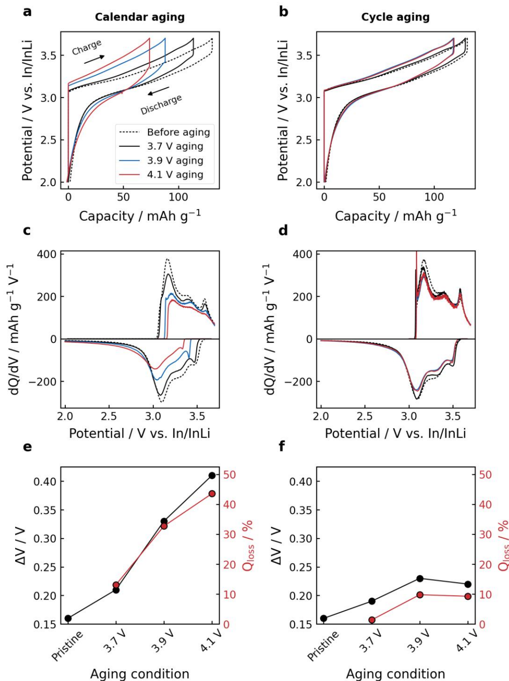
Figure 3. Data measured in the last formation cycles (before aging) and last RPT cycles (aging). (a–b) Potential versus capacity profiles, (c–d) corresponding differential capacity plots, and (e–f) comparison of voltage gap and capacity loss of accelerated calendar and cycle aging cells, respectively. Data from all investigated cut-offs can be found in Figure S2 .
