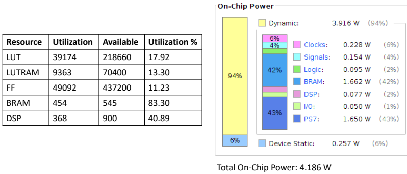
Figure 3.25 | Resources utilization and power report. Utilization of the programmable logic part of the XC7045 AMD Xilinx Zynq SoC device for the implemented HNC node prototype (left), and the AMD Xilinx Vivado on-chip power report for a PL clock frequency of f_{clk} = 200 MHz (right).
