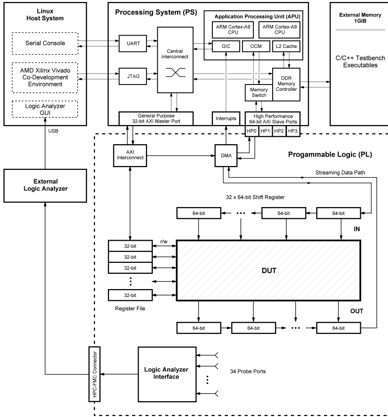
Figure 4.2 | Testbench. The testbench setup exploits the AMD Xilinx Zynq-7000 SoC device architecture. It makes use of the Application Processing Unit (APU) to set up a software-controlled test environment. The hardware component to be tested – the device under test (DUT) – can be connected to a register file as well as a streaming interface. For timing analysis and debugging purposes, a 34-channel logic analyzer interface is provided, which allows for probing any signal.
