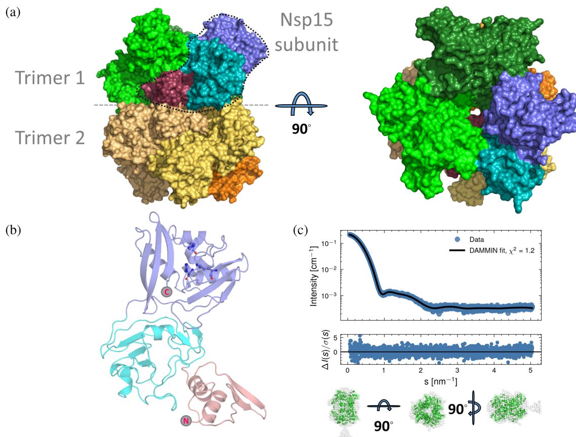
FIGURE 5 (a) The Nsp15 hexamer in two orientations (rotated 90 degrees). Each Nsp15 subunit has a unique color. For one subunit, circled in dashed line, the three domains of the protein are shown (Nsp15 N-terminal domain in raspberry, the middle domain in cyan and the EndoU in slate blue). (b) Domain organization and domain boundaries of Nsp15. The catalytic triad is in ball and stick. (c) DAMMIN fit (solid line) and the hexamer model (produced from PDB ID 6wlc, in green) overlaid to the ab-initio model (gray beads) shows that Nsp15 is mostly hexameric in solution as well.
