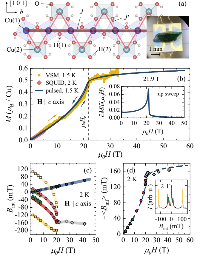
FIG. 1. (a) Sawtooth-chain unit in atacamite (space group Pnma ) formed by Cu(1) (basal) and Cu(2) (apical) sites; structural data from Ref. [27]. The Cu-O plaquettes are completed as Cu(1)(OH) 4 Cl 2 and Cu(2)(OH) 5 Cl octahedra [28]. Inset: atacamite single crystal on a puck for heat-capacity measurements. (b) High-field magnetization for \mathbf{H} \parallel c axis measured using a vibrating sample magnetometer (VSM) in dc fields as well as pulsed-field magnetometry [28]. We used SQUID data for scaling the pulsed-field data. Inset: field derivative of the magnetization (pulsed). (c),(d) ^1\text{H} -NMR results for \mathbf{H} \parallel c axis. A typical ^1\text{H} -NMR spectrum for the low-field AFM ground state is shown in the inset of (d). We plot the field dependence of (c) the internal fields B_{\text{int}} of the individual resonance lines, as well as (d) the mean shift of each line pair \langle B_{\text{int}} \rangle , which represents the local uniform magnetization within the AFM phase. The blue dashed line in (d) corresponds to the bulk magnetization from panel (b) scaled by -0.33 \text{ T } \mu_B^{-1} .
