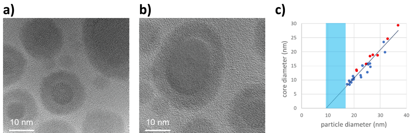
Fig. 2. a-b) Examples of HR-TEM images showing spherical/spheroidal core-shell nanoparticles used for diameters analysis. c) Scatter graph of core diameters vs. nanoparticle diameters, where red points refer to nanoparticles subjected to 10 min exposure to air and blue points to nanoparticles subjected to 6 months exposure. Black dashed line extrapolates linear fitting of the entire dataset to d_c = 0 . Cyan area emphasizes the lack of nanoparticles with core-shell structures smaller than about 17 nm although in principle they could exist down to about 9 nm.
