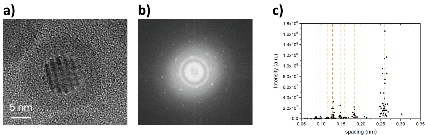
Fig. 3. a) Example of an HR-TEM image and corresponding FFT analysis (b). c) Statistic of the lattice spacing values extracted from FFT analysis on 30 nanoparticles, obtained by plotting the intensities of the Fourier components against lattice spacing values. Orange dashed lines are positioned along the weighted averages of spacing values of each accumulation groups of dots.
