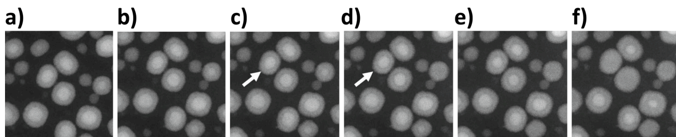
Fig. 5. a-f) HAADF-STEM image series showing structural transformations within Sn/SnOx nanoparticles. Images side is 80 nm, elapsed time between frames is 26 s. Framed area in a) is slightly shifted upward with respect to objects position. Arrows in c-d highlight the particle enlarged in Fig. 6 a-b.
