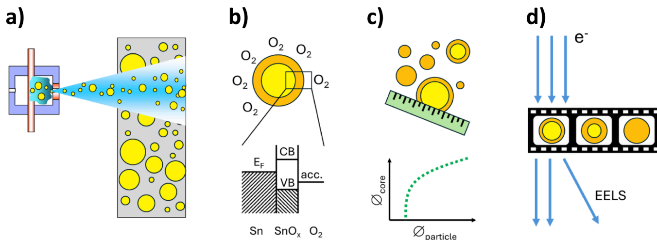
Fig. 1. Scheme of the research content of the article. a) Sn nanoparticles were produced in UHV by Supersonic Cluster Beam Deposition. b) Air exposure at room temperature induced surface oxidation according to Cabrera-Mott mechanism, based on electron tunnelling from Fermi level of Sn ( E_F ) to oxygen acceptor levels (acc.). c) Diameters of particles and of their metallic cores were correlated. d) Electron Energy Loss Spectra (EELS) and evolution of core–shell structures upon e-beam irradiation were finally investigated.
