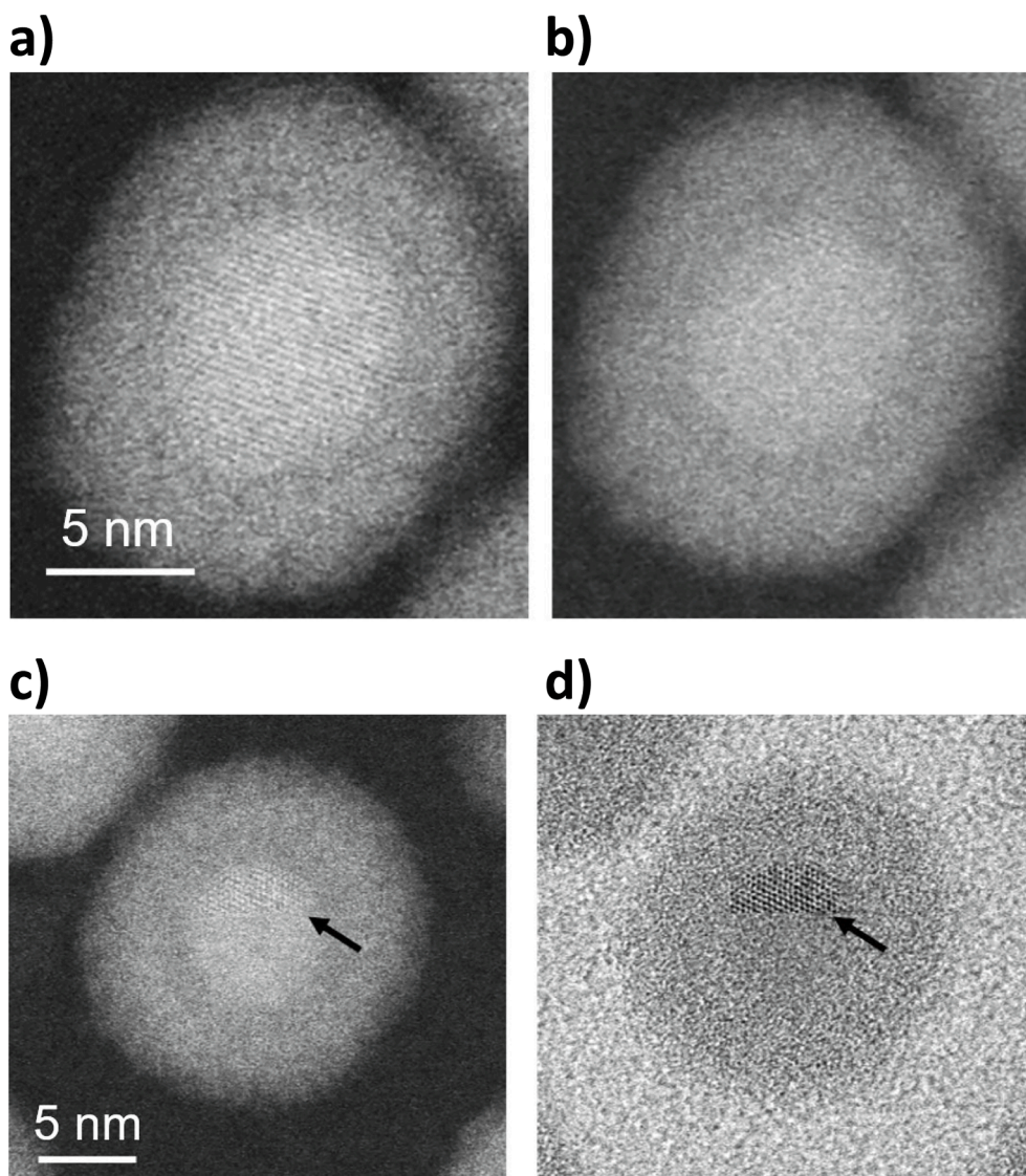
Fig. 6. a-b) Consecutive frames of an HAADF-STEM image series of the same core-shell nanoparticle during e-beam irradiation, showing the sudden disappearing of the crystalline lattice structure in the metallic Sn core. As the image contrast of the core in the second frame is still different (lighter) from the one of the oxide shell, we argue that a phase transition from crystalline solid to liquid is taking place in metallic tin core. The images refer to the particle pointed by the arrows in Fig. 5. c-d) Corresponding HAADF and bright-field STEM during e-beam irradiation, showing the sudden disappearing of the crystalline lattice structure during image acquisition (see image contrast change in the bright field image, black arrow) in the metallic Sn core. Again, the image contrast of the core in the corresponding HAADF-STEM image is still different (lighter) from the one of the oxide shell.
