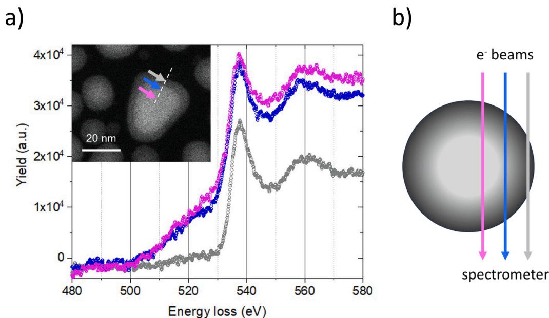
Fig. 4. a) EELS spectra from different regions of a single core-shell nanoparticle: core (purple), shell (grey), and in between region (blue), as indicated in the inset, where the side of the white square is 50 nm. Peak at energy loss values 530–545 eV is attributed to oxygen K-edge, which overlaps to tin M4 – M5 delayed edges constituting the background signal on the rise at around 500 eV. Except for the rise of tin-related background in blue and purple spectra, no major differences can be highlighted. We suppose that, due to spherical geometry and similar dimensions of shells and cores, EELS spectra collected at different radial positions are the overlap of contributions of different stoichiometries in similar amount, as schematically shown in b).
