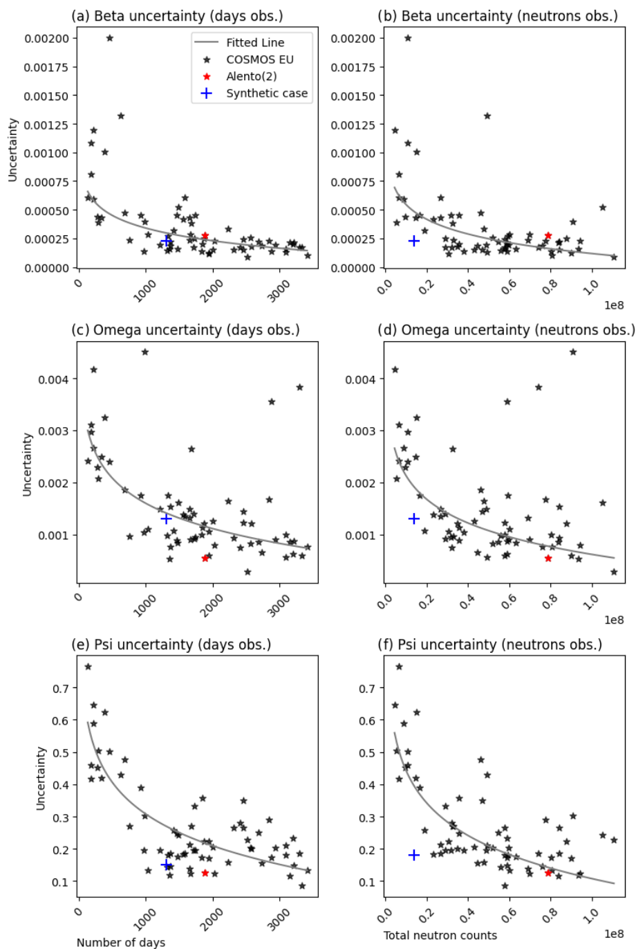
Figure 5. Uncertainty of beta, psi, and omega with respect to consecutive days of measurement ( a , c , e ) and neutron flux ( b , d , f ) over the whole time period. One outlier was removed for omega. Uncertainty calculated for the Alento site is marked as a red asterisk, and the synthetic test case (1000 realizations) is marked as a blue plus. The solid grey lines denotes the logarithmic fitted line.
