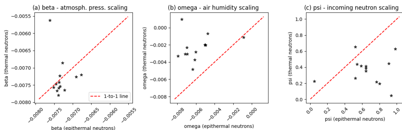
Figure 6. Results of scaling parameters, namely (a) beta, (b) omega, and (c) psi, for thermal neutron counts using bare counter tubes against epithermal neutron counts using a moderated tube. Moderated, i.e. epithermal, counts are commonly used for soil moisture determination with CRNSs.
