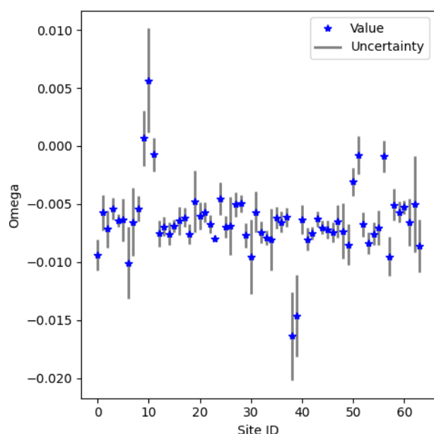
Figure 3. Omega estimates (blue star) and uncertainty (grey bars) of omega estimates for scaling CRNS counts with air humidity. The result of the site WEC001 is excluded because of its high uncertainty (uncertainty = 0.02).
