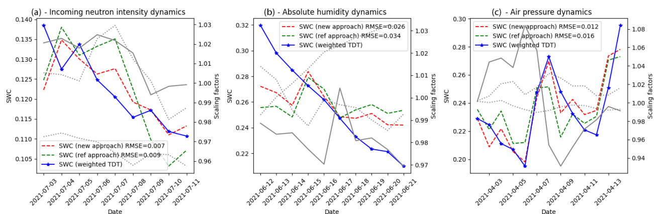
Figure 7. Evaluation results for MFC2 at the Alento site (ALC002 in Bogena et al., 2022). High variations in (a) incoming neutron intensity, (b) absolute air humidity, and (c) atmospheric pressure are compared against observed vertically weighted soil water content (SWC). Solid grey lines are the respective correction factors, with the other dashed lines representing the corresponding secondary scaling factors for this period.
