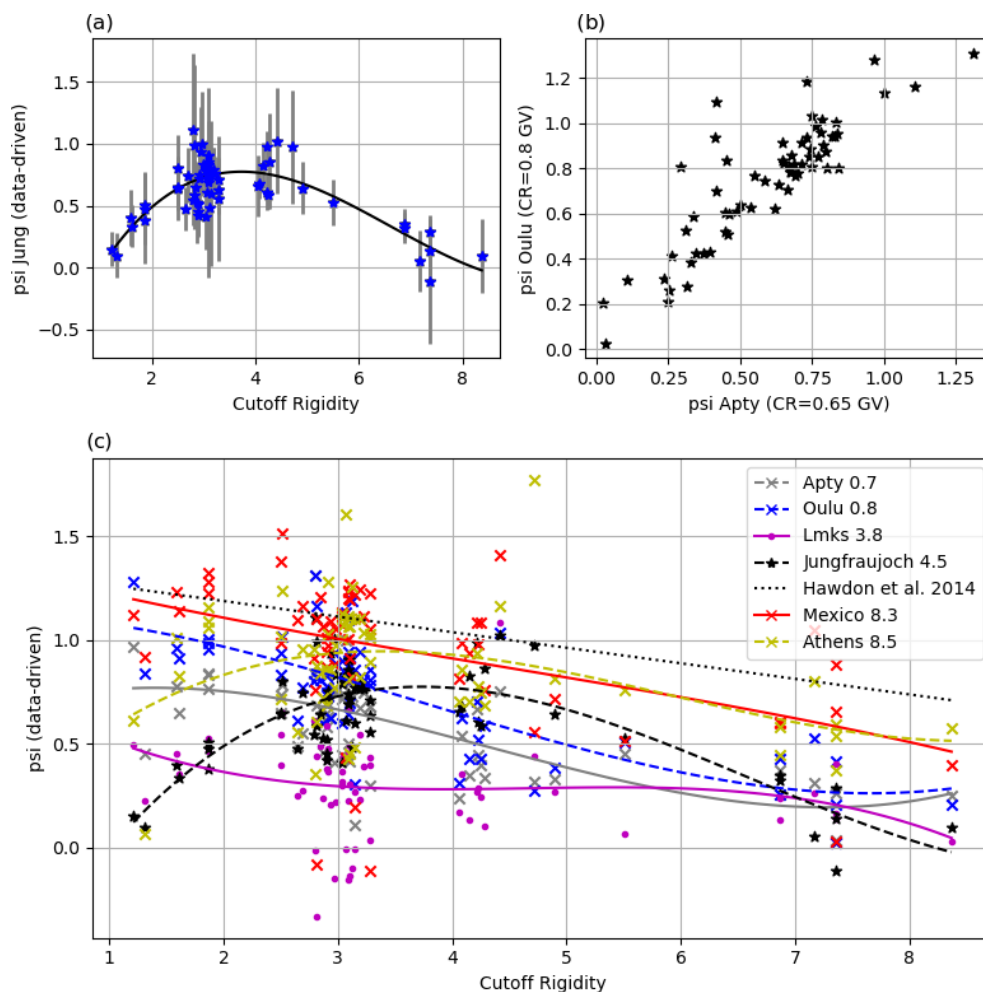
Figure 2. Psi estimated for 64 COSMOS-Europe sites and different NMDB monitors: (a) Jungfraujoch and (b) Apty and Oulu. Panel (c) includes also results for Lmks, Mexico, and Athens with the NMDB monitor's cutoff rigidity denoted in the legend. Psi estimates are provided as dots, X's, and asterisks. Polynomial regressions to NMDB monitors are shown as lines. Hawdon et al.'s (2014) study is provided with reference to Jungfraujoch.
