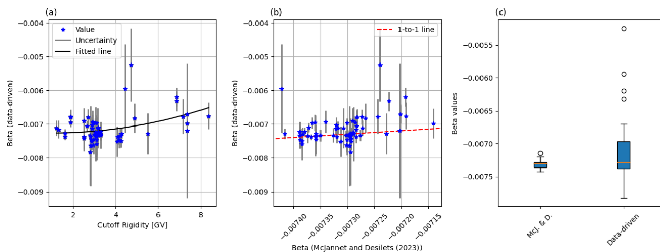
Figure 1. (a) Beta estimate and second-order polynomial regression with cutoff rigidity for the COSMOS-Europe sites, excluding sites BUC001 and LEC001. (b) Beta estimates of this study (data-driven) in comparison to those derived by McJannet and Desilets (2023). (c) Boxplot of beta estimates of this study (data-driven) in comparison to those derived by McJannet and Desilets (2023). Indicated are the median of the data sets (horizontal bar), the outliers (circles), the box (25th and 75th percentile – interquartile range), and whiskers (1.5× interquartile range).
