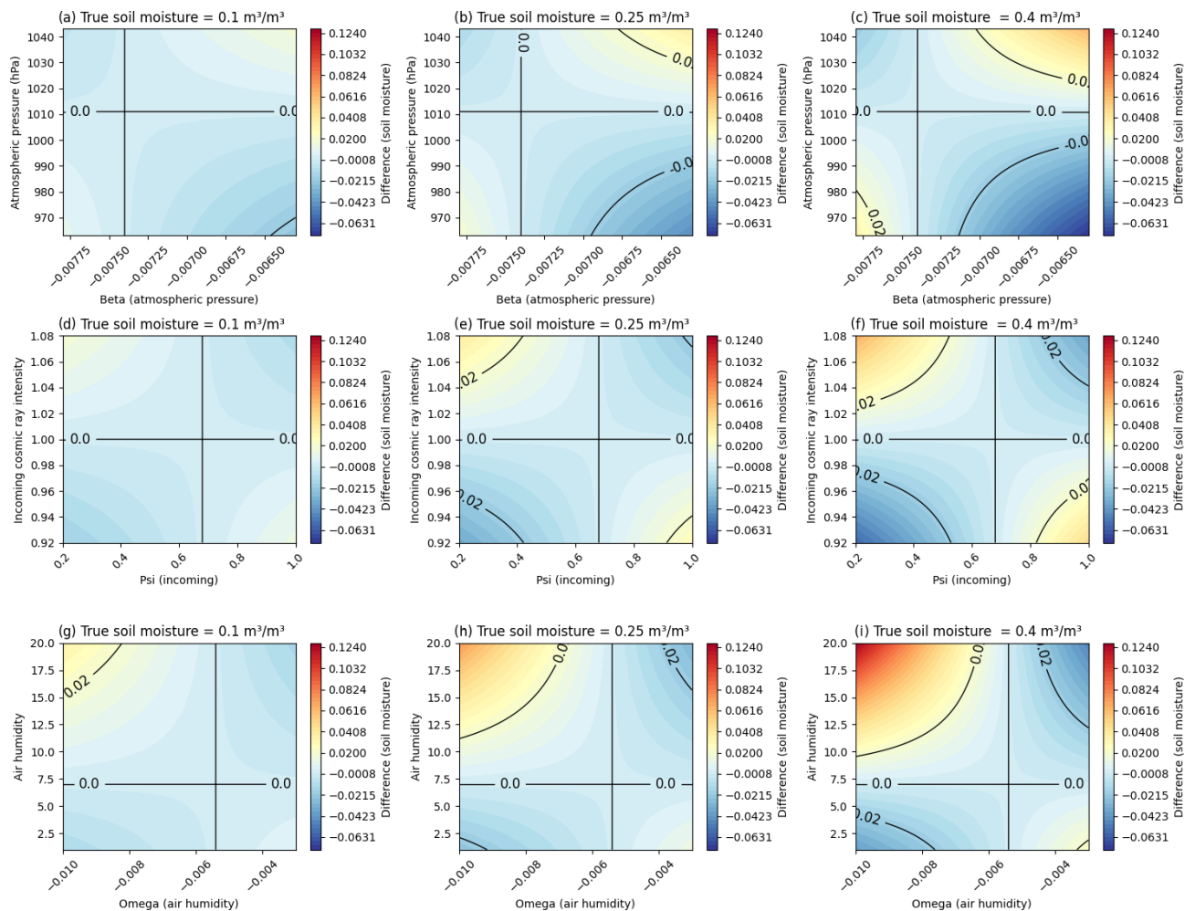
Figure 4. Sensitivity of soil moisture calculated as the difference between estimated and true soil moisture. Estimated soil moisture depends on atmospheric pressure (a–c), incoming neutron intensity (d–f), and air humidity (g–i) and their respective ranges. True soil moisture remained constant, while estimated soil moisture depends also on the reference value of omega and reference value of air humidity. Contour lines show soil moisture differences of 0.02 \text{ m}^3 \text{ m}^{-3} (curved) and 0.00 \text{ m}^3 \text{ m}^{-3} (straight) to reference values. Differences between the estimated moisture and true soil moisture were always highest for moist conditions, e.g. 0.4 \text{ m}^3 \text{ m}^{-3} .
