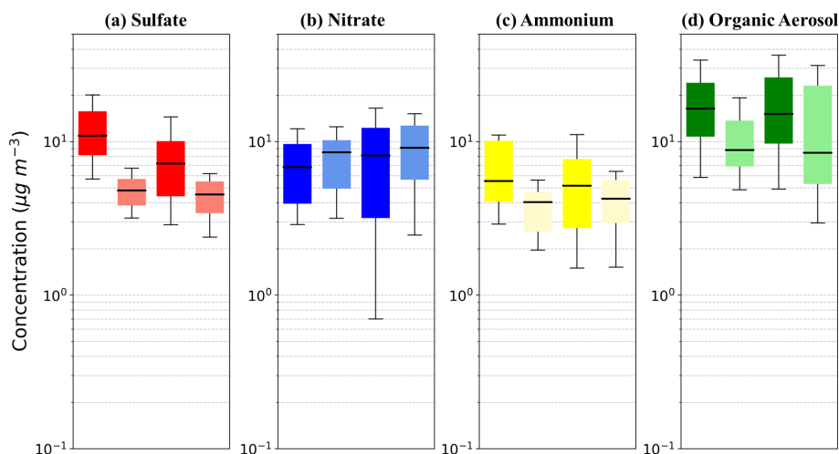
Figure 17. Decadal PM 1 concentration trends in Eastern Asia expressed by the bar plots of the mass concentration (in \mu\text{g m}^{-3} ) for (a) sulfate, (b) nitrate, (c) ammonium, and (d) OA during the periods 2006–2012 (left) and 2013–2020 (right) as calculated from the AMS observational dataset (dark colors) and the corresponding simulation values (light colors). The upper and lower whiskers range from 10 % to 90 % of the dataset, and the quartiles from 25 % to 75 % of the dataset. The black line is the median.
