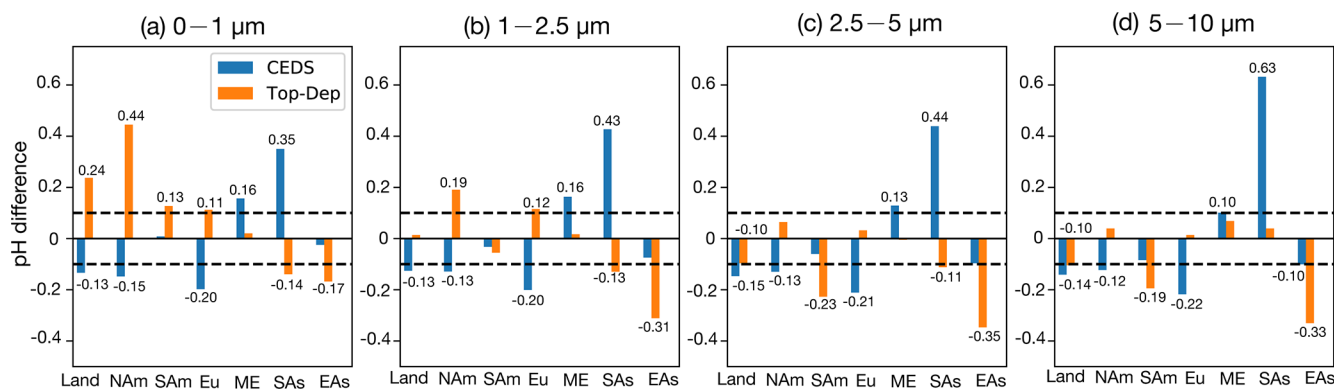
Figure 10. Bar plots for the pH value absolute difference between the CEDS/Top-Dep case and base case in the four size ranges (a–d), with the two dashed lines representing the value of 0.1 and -0.1 , respectively (Land: global land; NAM: North America; SAM: South America; Eu: Europe; ME: Middle East; SAs: South Asia; EAs: East Asia).
