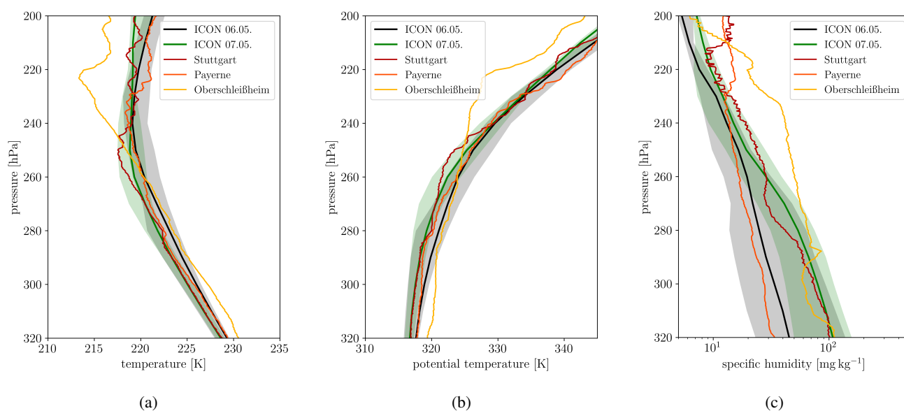
Figure A4. (a) Temperature, (b) potential temperature, and (c) specific humidity as function of pressure from three radio sounding sites (red) and the ICON model simulations sampled over the origin region of the trajectories (shown in Fig. 11). Black and green colors correspond to ICON initialisation dates of 12 UTC 06 May 2013 and 00 UTC 07 May 2013, respectively. In contrast to Fig. 11 the simulations have been sampled in their respective trajectory source areas. The solid line shows the median profile, the shading indicates the 5 th to 95 th percentile range.
