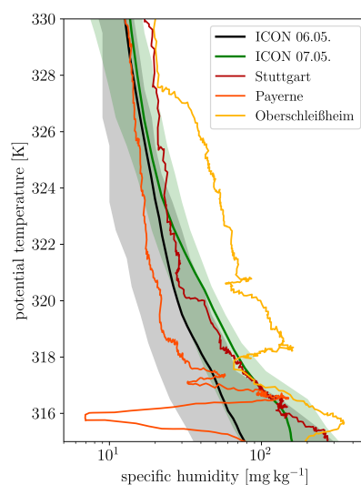
Figure A3. Specific humidity profile as function of potential temperature at 00 UTC on 07 May 2013 from three radiosonde sites (red) and the ICON model simulations sampled over the origin region of the trajectories (shown in the left panel). Black and green colors correspond to ICON initialisation dates of 12 UTC 06 May 2013 and 00 UTC 07 May 2013, respectively. In contrast to Fig. 11 the simulations have been sampled in their respective trajectory source areas. The solid line shows the median profile, the shading indicates the 5 th to 95 th percentile range.
