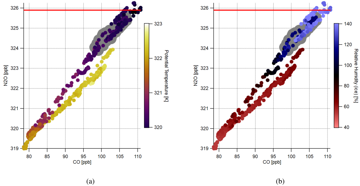
Figure 4. Scatter-plots of N 2 O versus CO color coded with (a) potential temperature and (b) relative humidity with respect to ice. The N 2 O-defined tropopause is marked as red line with lower N 2 O mixing ratios implying stratospheric air. Grey circles indicate cirrus occurrence.
