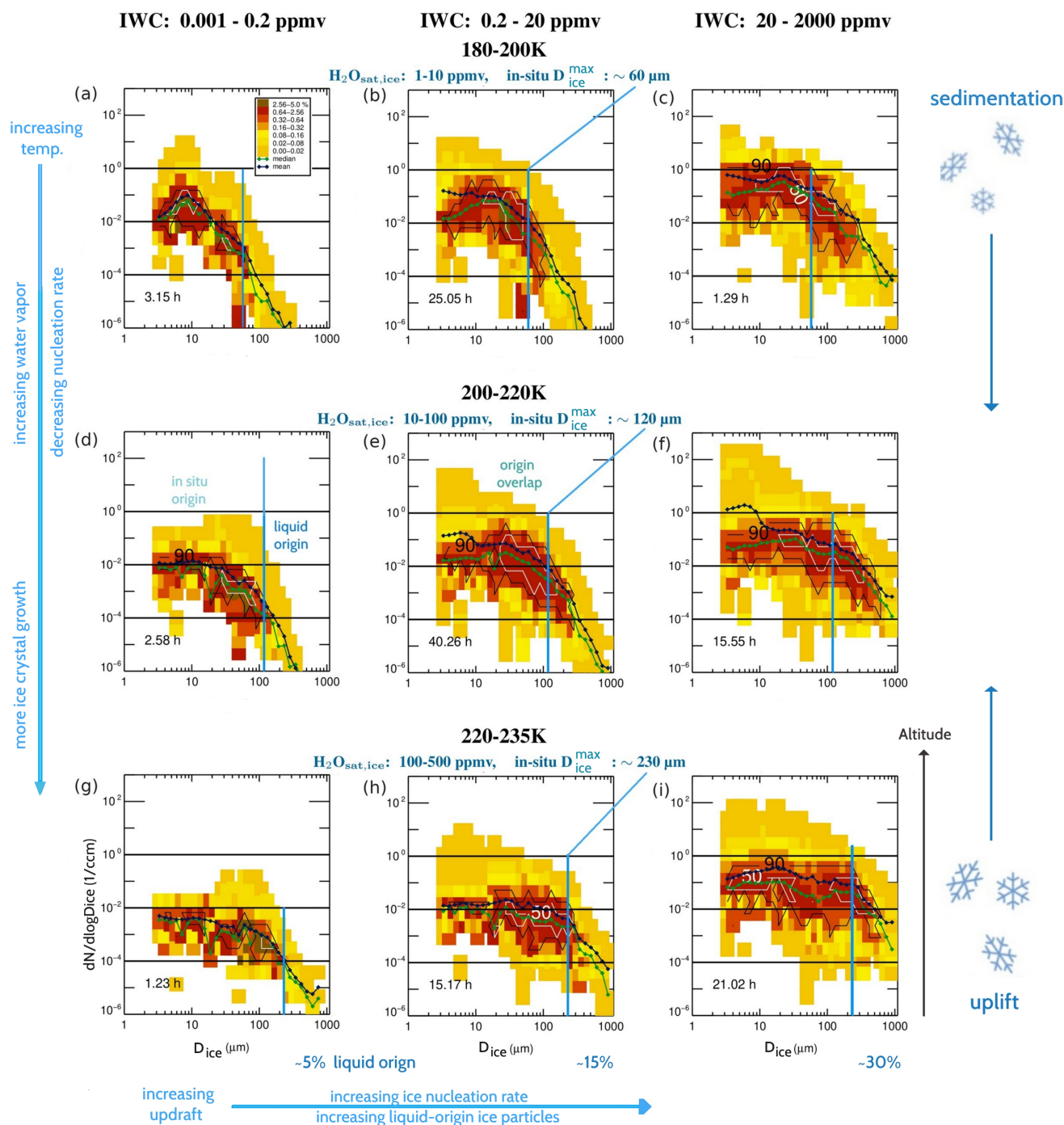
Figure 7. Cirrus cloud particle size distributions (PSDs) in nine IWC-T (Ice Water Content - Temperature) intervals, color coded by frequencies of occurrence; green/black lines show median/mean PSDs, black/white contour lines enclose 90 / 50% of the data points; the entire data set represent 137.3 hours of measurements. In the respective temperature ranges, the water vapor saturation mixing ratios ( H_2O_{sat,ice} ) and the simulated maximum ice crystal sizes for in situ-origin cirrus (in situ D_{ice}^{max} ) are denoted in blue (see also Tables 1 and 2).
