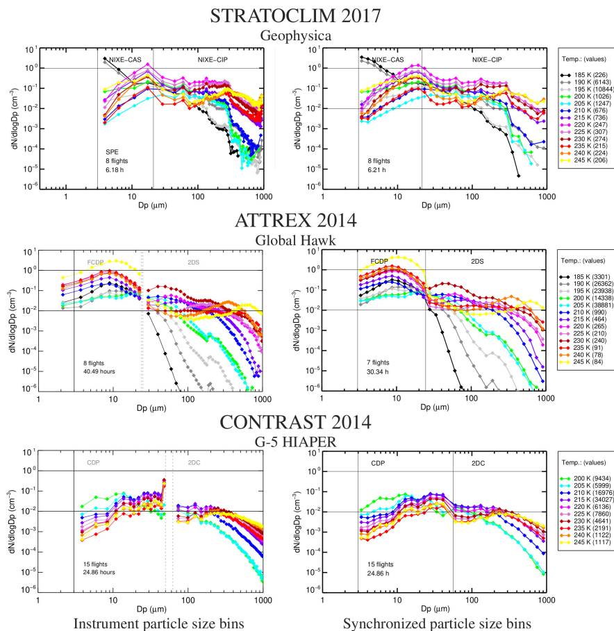
Figure 5. Cloud particle size distributions in 5K temperature intervals from three field campaigns with different aircraft and different pairs of instruments: NIXE-CAPS (StratoClim; CAS-depol+CIPgs), FCDP+2D-S (ATTREX) and CDP+2D-C (CONTRAST; note that the CDP outliers at 50 \mu\text{m} are filtered out); the size of the particles from the optical array probes (CIPgs, 2D-S, 2D-C) is maximum dimension. Left column: original irregular size grid of the instruments; Right column: synchronized logarithmic equidistant size grid. Note that the transition between each respective pair of instruments is smooth, indicating no systematic errors in the measurements of the individual instruments.
