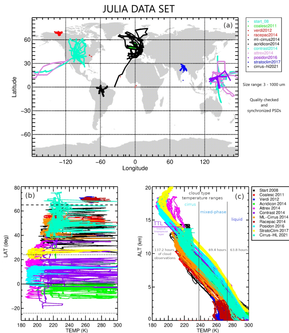
Figure 4. The Jülich In situ Aircraft data set (JULIA) of particle size distributions (PSDs). (a) map of flights (adapted with changes from Bartolomé García et al., 2024), (b) latitude-temperature distribution, (c) altitude-temperature profiles. The data set contains 11 campaigns between 2008 and 2021 (as indicated in the legends) where PSDs were measured; this corresponds to 163 flights, totalling 270.4 hours in cirrus, mixed-phase and liquid clouds).
