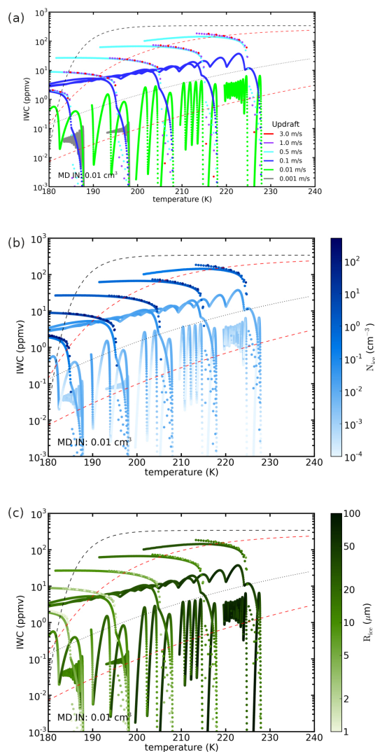
Figure 3. Cirrus cloud MAID IWC climatology; MD, INP = 0.01 cm^{-3} , s09, het-hom, 80 - 13000 min, dyn. equil., (adapted from Krämer et al., 2016, ).
