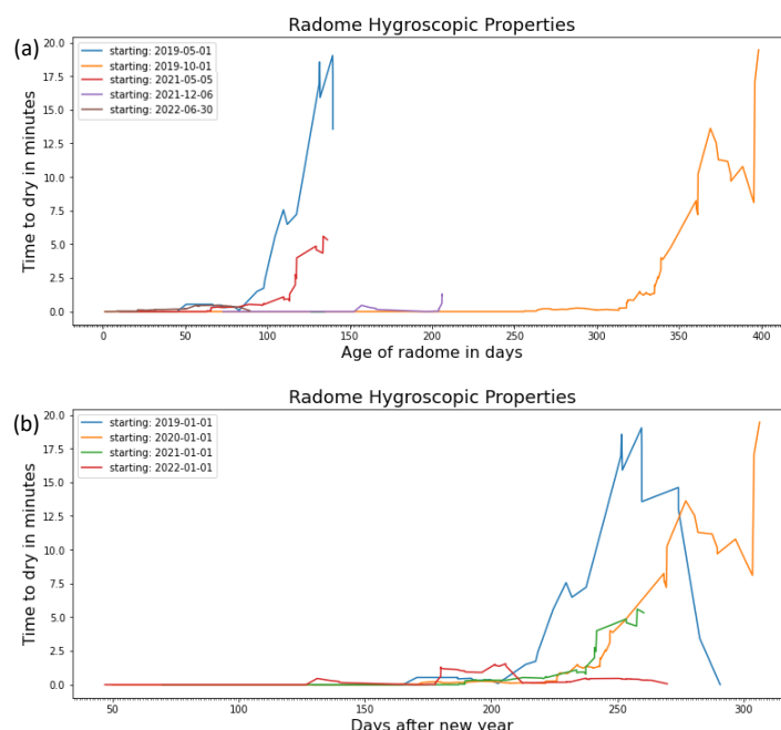
Figure 12: 30 day rolling maximum of “time to dry” plotted against radome-age (a) and days of the year (b) for DWDHAT. This evolution only contains the worst cases. Several rain events under more favorable conditions in between lead to a shorter “time-to-dry”.
