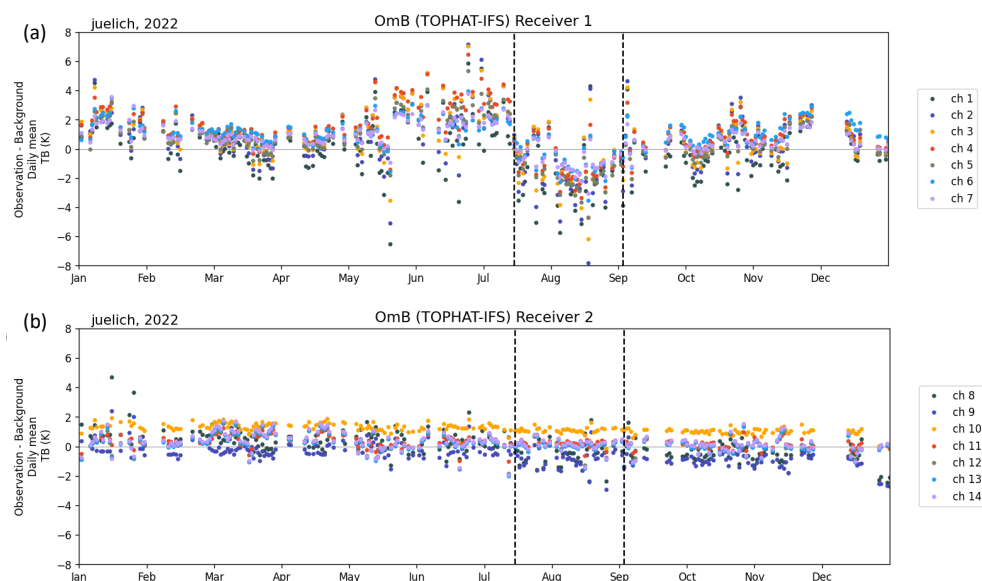
Figure 5: Daily means of OmB brightness temperature differences for TOPHAT at JOYCE during 2022, (a) for K-band (Receiver 1) and (b) V-band (Receiver 2). The dashed lines indicate times of LN2 calibrations. Observations and background are clear-sky only.
