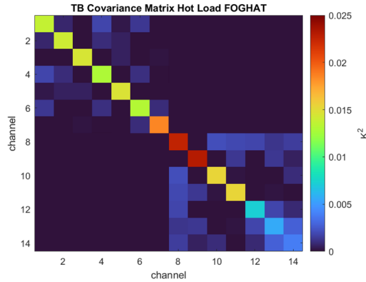
305 Figure 2: Typical T_B covariance matrix for FOGHAT (Gen5 HATPRO) with a 5 min observation time on the hot load target (1 s integration time). The square root of the elements on the diagonal yields the noise values for each channel.
