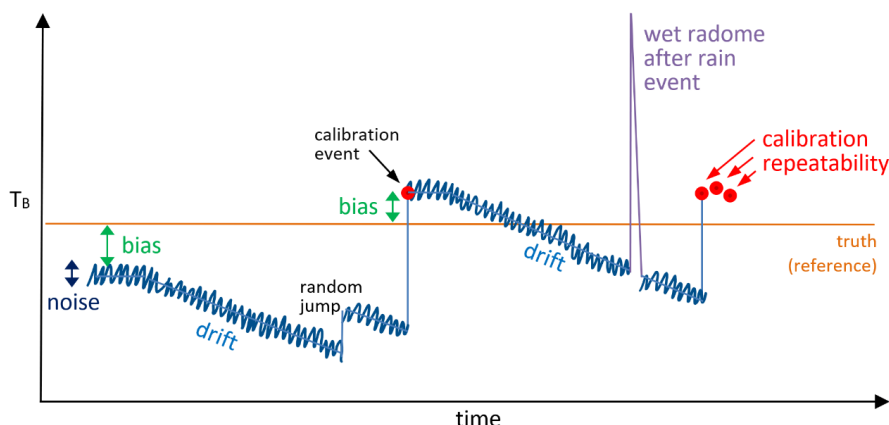
95 Figure 1: Sketch showing an overview of the analyzed MWR instrument uncertainties in terms of brightness temperatures ( T_B ) over time. It depicts radiometric noise, long-term drifts or jumps between absolute calibrations, calibration repeatability, biases, and radome degradation. Biases usually disclose instrument differences to an absolute reference or theoretical truth but can also describe the differences between two instruments. Radome degradation is a measure of how long a wet radome needs to dry after a rain event.
