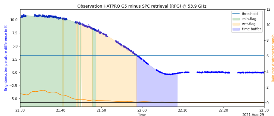
620 Figure 11: Observation minus SPC-retrieval (blue curve) of DWDHAT during events with rain on 29 Aug. 2021. The rain rate is shown in orange. Rain events registered by the precipitation sensor are shaded green, while the wet flag is shaded orange, and the time buffer is shaded purple. The solid blue line indicates the threshold for OmSPC ( \Delta T_{limit} ) on this day.
