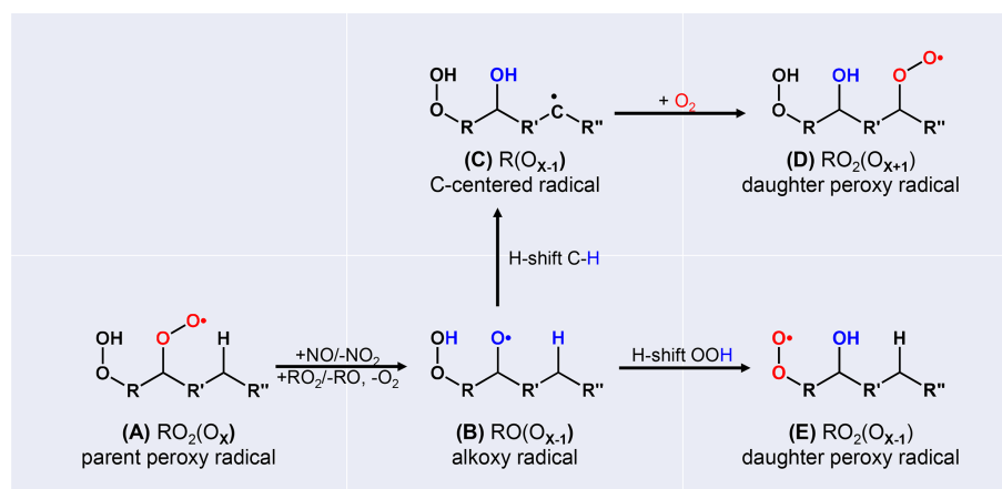
Figure 1. Schematic sketch of the alkoxy-peroxy pathways (A, B, C, D) and (A, B, E), considering fast isomerization of the alkoxy radical (B) by H-shift from a C-H bond, or by H-shift from a HO 2 • group. The resulting peroxy radicals (D), (E) have one more or one less oxygen atom compared to the parent peroxyradical (A); thus, the parity of the oxygen number is changed.
