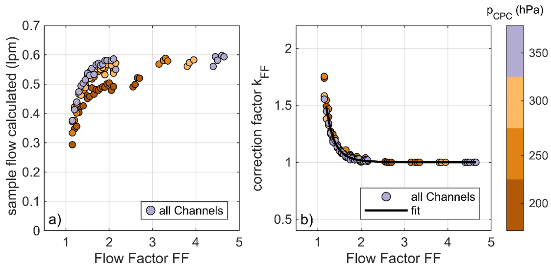
750 Figure B1: a) sample flow of all three mc-CPC channels combined measured by a TSI flowmeter against the Flow Factor FF, b) correction factor k_{FF} ( = \text{flow}_{\text{max}}/\text{flow} ) derived from the sample flow, color coded by the internal pressure. The measurements were done at GUF. The data points represent binned data.
