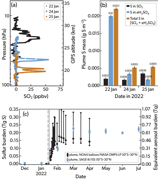
Figure 2.11: Balloon-borne vertical profiles of SO 2 over the Maïdo...in La Réunion. a) and b) adapted from Asher et al. (2023). c) The calculated total sulfur burden (and equivalent aerosol burden) calculated based on a combination of NASA OMPS-LP measurements and balloon-borne measurements, and from SAGE-III/ISS measurements assuming 70 percent weight of sulfuric acid in aerosol. Data in c) from Asher et al. (2023) and Duchamp et al. (2023). Error Bars represent the measurement uncertainty.
