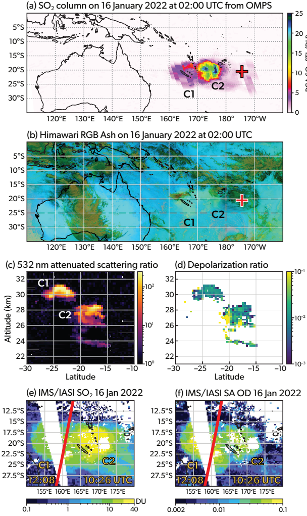
Figure 2.6: (a) SO 2 column for C1 and C2 clouds as seen from OMPS on 16 January 2022 at 2 UTC adapted from Carn et al. (2022), (b) Himawari false colour imagery using channels at 8.5, 10.4 and 12 \mu m for the same time showing C1 and C2 sulfate aerosols as greenish bright patches; brown patches are clouds and Australia is bright due its high infrared emission, (c) 532 nm attenuated scattering ratio from CALIOP on 16 January 2022 at 15:08 UTC intersecting C1 and C2, (d) depolarisation ratio in C1 and C2 at the same time, (e) SO 2 column from IASI on 16 January 2026 from two swaths spanning C1 and C2, (f) sulfate aerosol optical depth on the same swaths (mainly retrieved from 8.5 \mu m band). The red line in panels (e) and (f) is the CALIOP track shown in (c) and (d). b-f are adapted from Legras et al. (2022).
