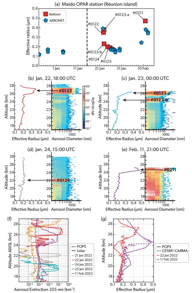
Figure 2.12: Aerosol size over Maito OPAR station (Réunion Island) in the first month following eruption (until 15 February 2022). (a) Time series of effective radius ( r_{\text{eff}} in \mu\text{m} ) from balloon-borne measurements with POPS (maximum r_{\text{eff}} , as a function of altitude, within the Hunga plume) with red squares (from Asher et al., 2023) and from AERONET column-integrated effective radius with blue pentagons (Boichu et al., 2023). Plume parcels (#) are illustrated in panels b–e below. (b–e) Vertical distribution of effective radius (left) and aerosol number size distribution dN/d \log D_p (right) up to an altitude of 30 km on (b) 22 Jan 18:00 UTC, (c) 23 Jan 00:00 UTC, (d) 24 Jan 15:00 UTC, (e) 11 Feb 21:30 UTC, b–e adapted from Asher et al. (2023). (f) Vertical profile of aerosol extinction at 355 nm calculated from POPS size distributions and Lidar backscatter observations (using vertical profiles of lidar ratios, i.e., aerosol extinction to backscatter coefficient ratios, derived from observations on each night). (g) Vertical distribution of aerosol effective radius on 22 January and 11 February from POPS observations (solid lines) and daily mean simulations with the CESM1-CARMA sectional aerosol model (dashed lines), adapted from Li et al. (2024).
