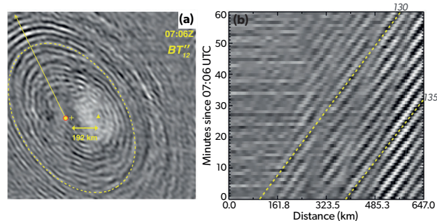
Figure 2.3: Taken from Horváth et al. (2024), Figure 15. (a) Second-order derivative in time of the brightness temperature from GOES 17 channel 12 at 07:06 UTC filtered to emphasise the wave field and (b) time–distance plot for the period 07:06–08:06 UTC along the yellow arrow in panel (a). The interval used to calculate time derivatives is \Delta t = 1 min. The yellow dashed curve is an ellipse fitted to one of the concentric rings with its centre marked by the plus sign. The distance between the ellipse centre and Hunga (yellow triangle) is also indicated. The observed 192 km shift is due to advection of the wave field by the mean flow (see Horváth et al., 2024).
