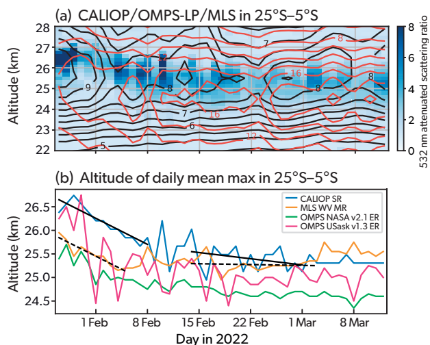
Figure 2.10: a) Comparative evolution of CALIOP attenuated scattering ratio (color), MLS water vapour mixing ratio (black contours, ppmv), OMPS-LP 745 nm extinction ratio (red contours) based on the NASA v2.1 product as in Taha et al. (2022). b) daily mean vertical locations of maximum of aerosols ratios and water mixing ratio. All quantities are zonally averaged in the 25°S–5°S latitude band. Slopes are fitted for CALIOP scattering ratio and MLS water vapour: respectively -79.0 \text{ m d}^{-1} and -78.8 \text{ m d}^{-1} in the early period before 8 February and -18.8 \text{ m d}^{-1} and -2.6 \text{ m d}^{-1} in the second half of February. Both panels show common descent of water and aerosols until early February followed by vertical separation.
