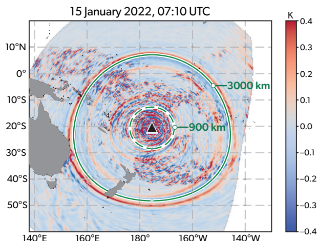
Figure 2.2: Himawari brightness temperature second-order difference at 07:10 UTC on 15 January 2022 (channel 8), adapted after Matoza et al. (2022). Wave fronts associated with the leading Lamb wave and slower gravity wave packets triggered by the eruption are clearly visible. Green circles are drawn to indicate equal distances from Hunga (dashed: 900 km; solid: 3,000 km).
