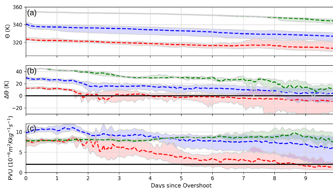
Figure 9. Forward trajectories. For three different \Theta levels, an ensemble of forward trajectories originating in the area of overshooting occurrence ( 58\text{--}59^\circ\text{N} , 11\text{--}14^\circ\text{E} ) is calculated using CLaMS. For the median (dashed lines) and the 10 %–90 % percentile (shaded), the plots show the evolution in coordinates of \Theta (a), \Theta difference to thermal tropopause (b) and PVU (c). The 2 PVU level in (c) is indicated by the black line.
