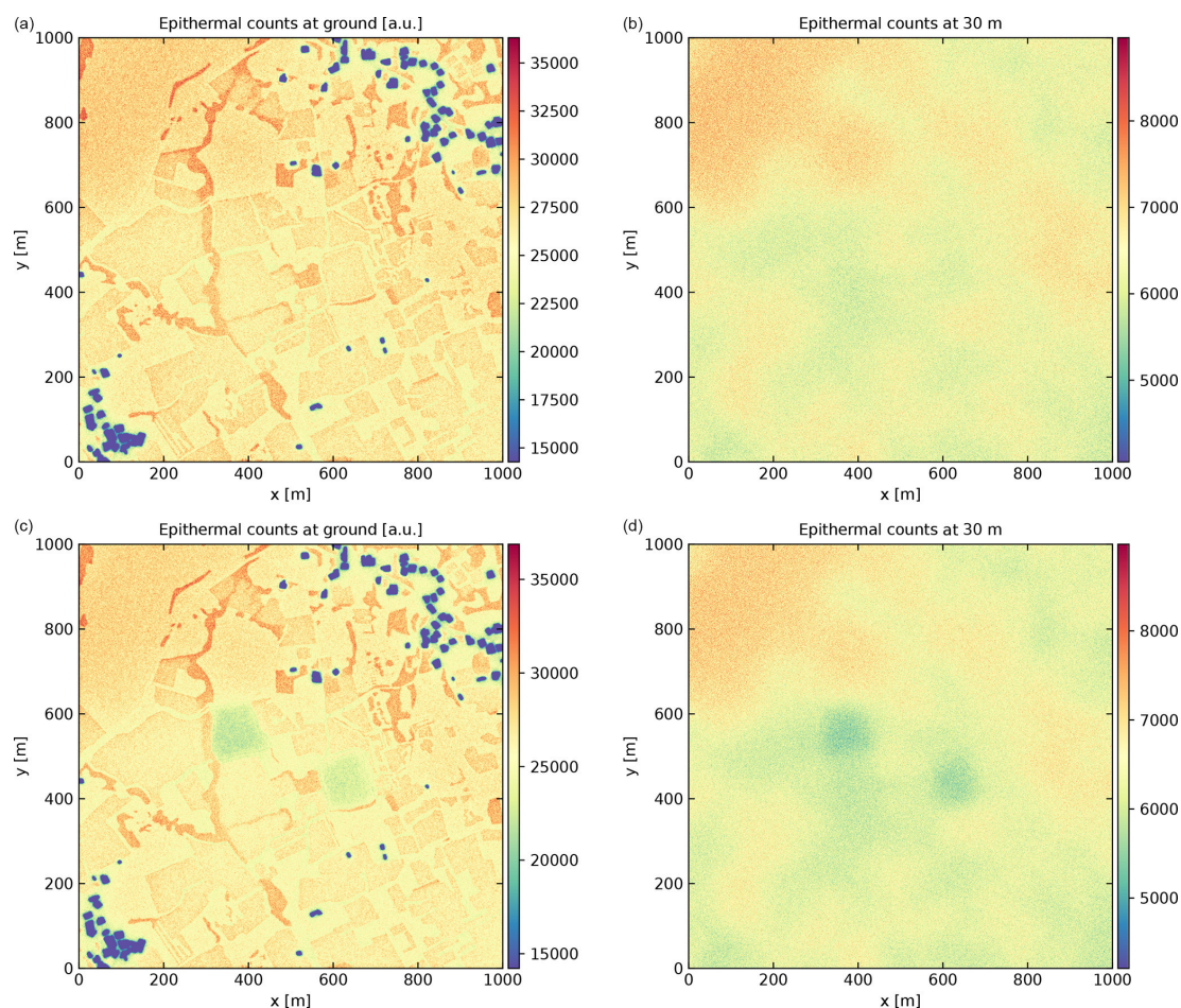
Figure 11. Simulated counts of epithermal neutrons near the ground (1–2 m, a ) and at 30 m ( b ) in a realistic Mediterranean landscape under conditions of low soil moisture variability (agia_dryout_dryin, a , b ) and with irrigated fields in dry surroundings (agia_dryout_wetin, c , d ).
