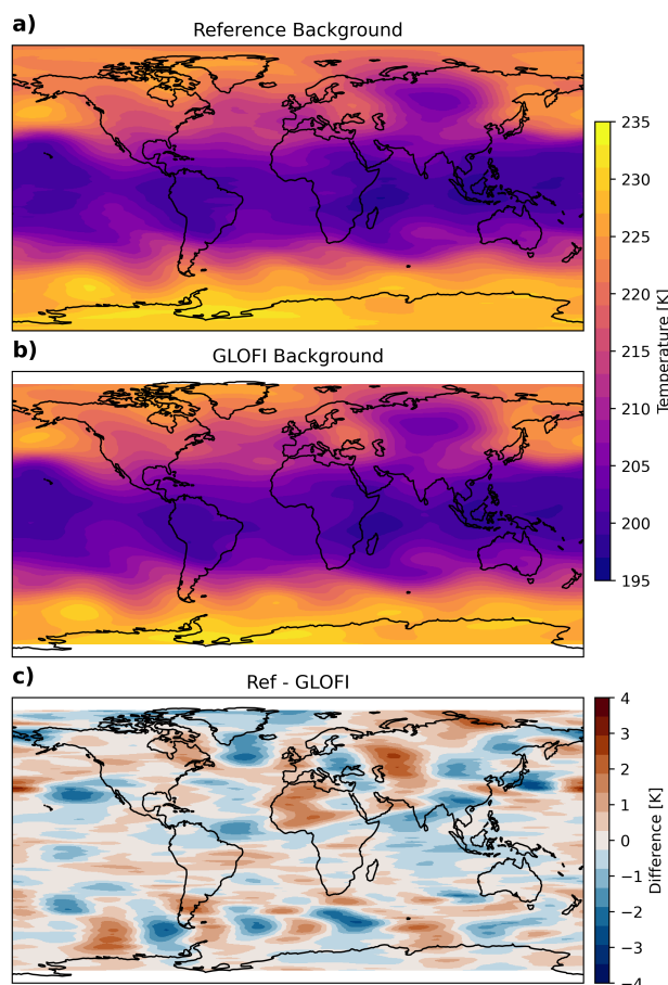
Figure 7. Temperature background from model data (a) and reconstructed from the GLOFI PW spectrum shown in 4.2 (b) as well as the difference between both (c). Shown is 2019-01-16T00:00 at 15 km altitude. Note that the differences are mostly due to the lack of tides.
