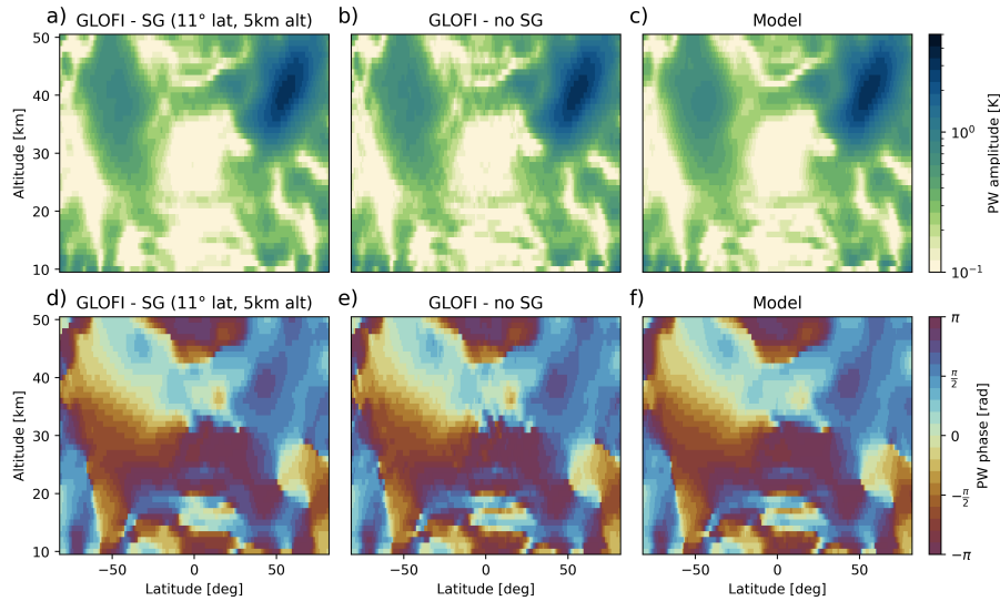
Figure 5. Comparison of amplitude and phase for the PW with zonal wavenumber 1 and frequency of -\frac{3}{28} cycles/day (9-day period) as determined by GLOFI with (a & d) and without Savitzky-Golay filtering (b & e) and from the full model data (c & f). The data shows the spectrum for the time window 2019-01-16 to 2019-02-12.
