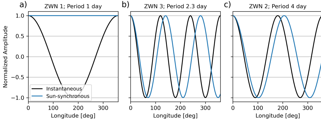
Figure 1. Sampling of global-scale waves from a sun-synchronous orbit for a) DW1 solar tide (e.g. Oberheide et al., 2000), b) quasi-two-day wave (e.g. Ern et al., 2013) and c) a fast Rossby-wave mode (e.g. Salby, 1984). Black is the actual wave at t = 0 and blue is the observed perturbation from the moving instrument accounting only for a single (e.g. ascending) orbit direction. Descending orbits would observe the system phase shifted depending on latitude.
