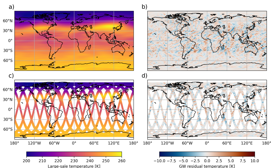
Figure 3. Example of the prepared test data for 2019-01-24. The upper row shows the model temperature large-scale background (a) and GW residuals (b) as the snapshot at 12:00 UTC. The bottom row shows the simulated observations of the (time-dependent) large-scale background as evaluated from the model PW spectrum (c) and the sampled GW residuals (d).
