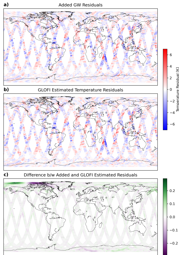
Figure 8. GW residuals as sampled from the model (a), as determined from the GLOFI algorithm (b) and the difference between the two (c) at 35km altitude for the day 2019-01-20.
