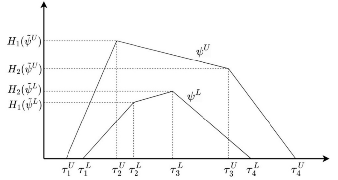
Fig. 2. Interval type-2 fuzzy set (IT2FS) \psi .
