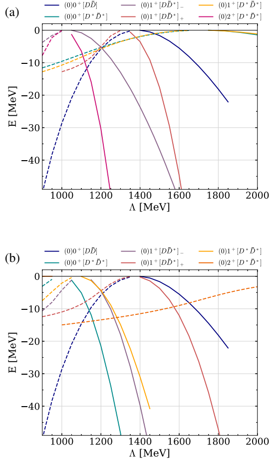
FIG. 4. Binding energy of the bound states (solid curves) or virtual states (dashed curves) in the single channels isoscalar systems as \Lambda increases. (a) With \delta(\mathbf{r}) . (b) Without \delta(\mathbf{r}) .
