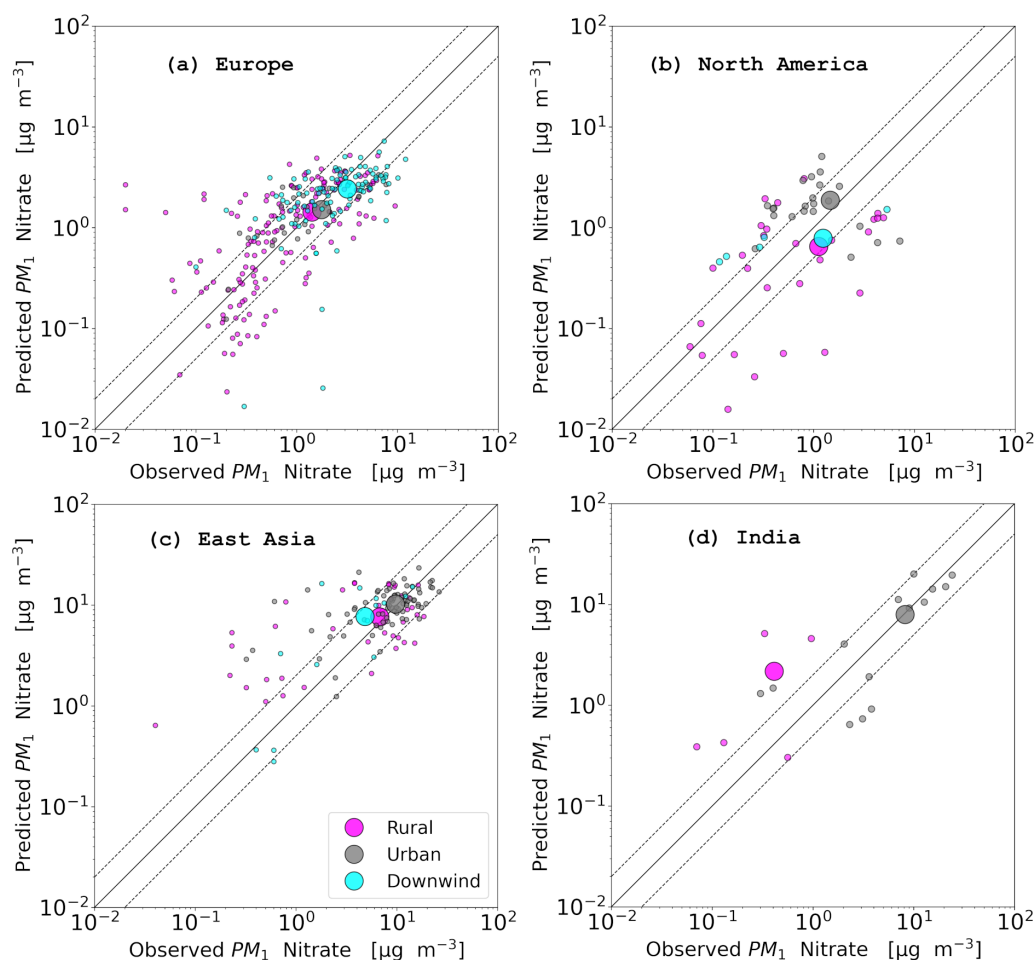
Figure 4. Scatterplots comparing monthly mean surface concentrations of \text{PM}_1 \text{NO}_3^- as simulated by EMAC from the base case and measured by AMS instruments in field campaigns in the regions of (a) Europe, (b) North America, (c) East Asia and (d) India. Enlarged dots indicate the 2010–2018 period averages from all locations. Also shown are the 1 : 1 line (solid) as well as the 2 : 1 and 1 : 2 lines (dashed).
